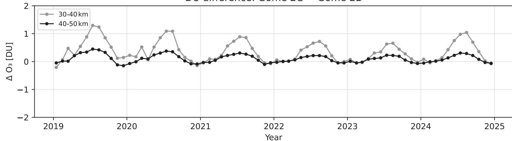
DU difference: Gome 2C – Gome 2B
