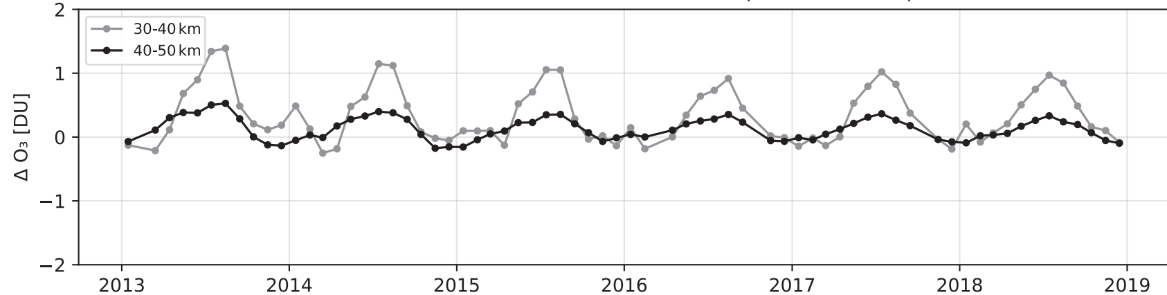
DU difference: Gome 2C – Gome 2B
