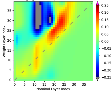
AveragingKernel 10 percentile; Lat 55N
