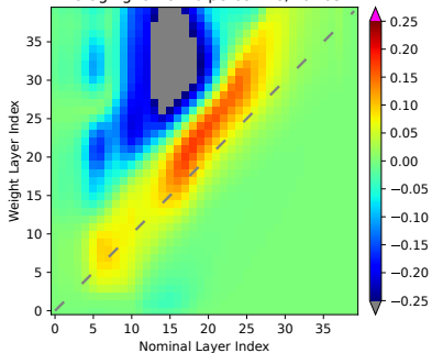
AveragingKernel 10 percentile; Lat 65N
