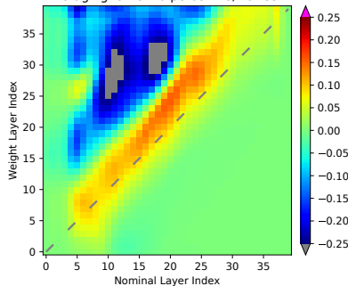
AveragingKernel 10 percentile; Lat 85N
