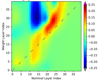
AveragingKernel 10 percentile; Lat 35N
