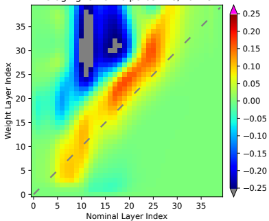
AveragingKernel 10 percentile; Lat 75N
