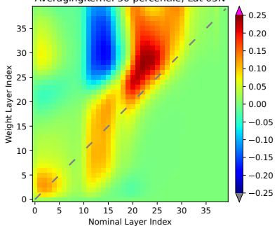
AveragingKernel 50 percentile; Lat 35N
