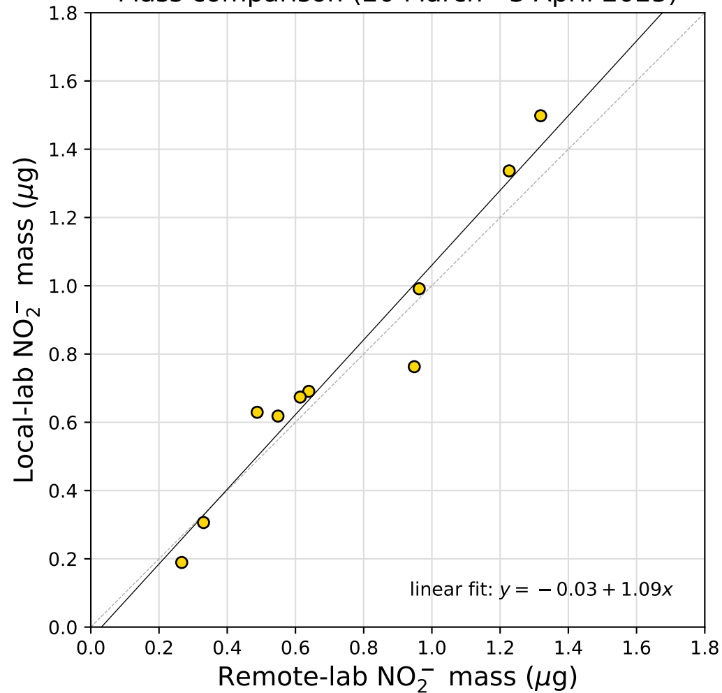
Mass comparison (20 March - 3 April 2025)
