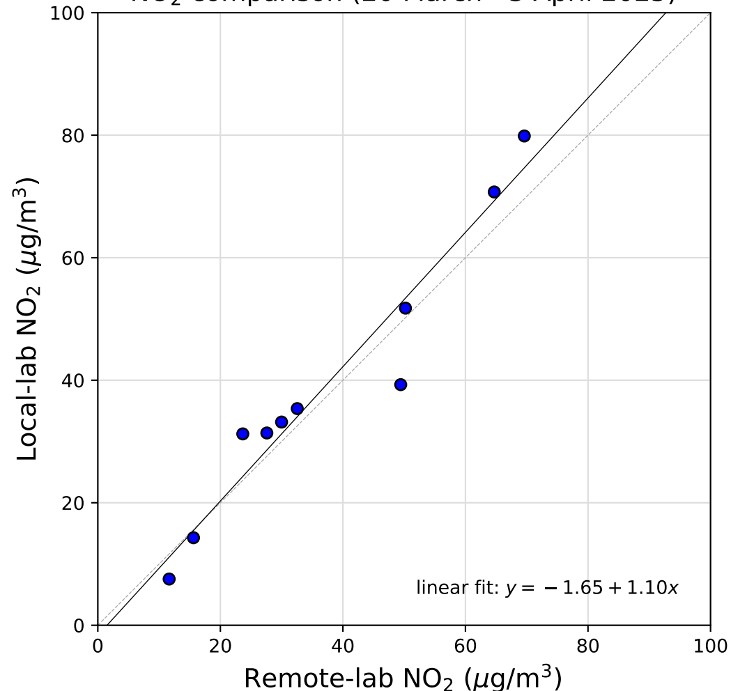
\text{NO}_2 comparison (20 March - 3 April 2025)
