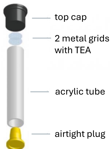
Figure 1. Components of the diffusion tube used in this study.
