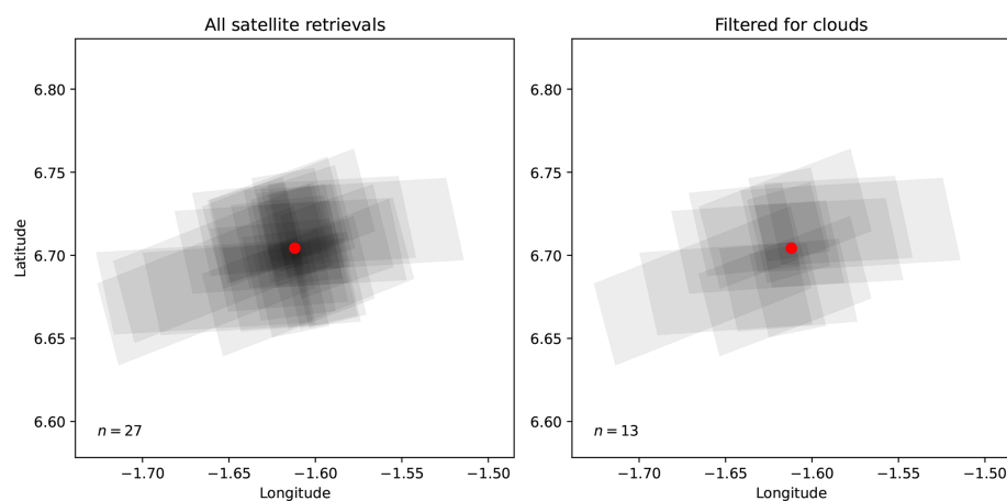
Figure 3. Sampling of location KU-016 (red dot) by TROPOMI during the measurement campaign (7 March–3 April). The left panel shows all satellite footprints in this period for a 28 \times 28 \text{ km}^2 area ( n = 27 ); the right panel shows only satellite footprints from valid retrievals under sufficiently cloud-free conditions ( n = 13 ).
