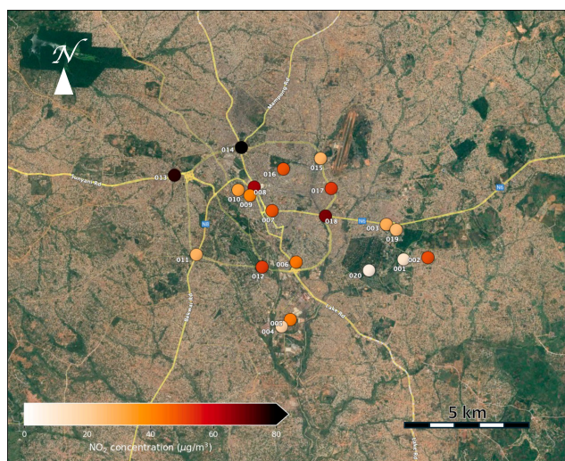
Figure 7. \text{NO}_2 concentrations measured in Kumasi by PDTs in March 2025. (Basemap taken from Google Maps © 2025 Google.).
