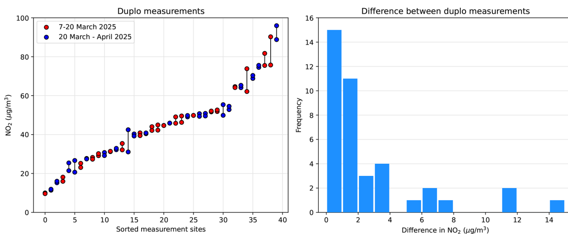
Figure 6. Results of duplo measurements done in the Kumasi network, sorted from small to large \text{NO}_2 concentrations (left). Most duplos agree within 2 \mu\text{g m}^{-3} (right).
