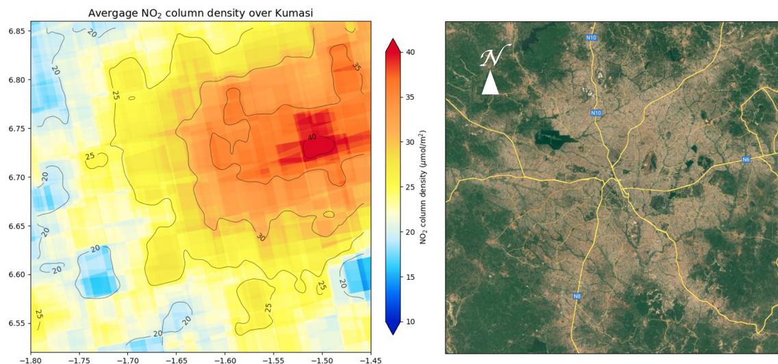
Figure 9. Averaged satellite measurement of tropospheric \text{NO}_2 columns density over Kumasi from 7 March to 3 April 2025. The map represents an area of 38 \times 38 \text{ km}^2 . Contour lines are shown for the measurement field smoothed with a Gaussian kernel of \sigma = 400 \text{ m} . (Basemap taken from Google Maps © 2025 Google.).
