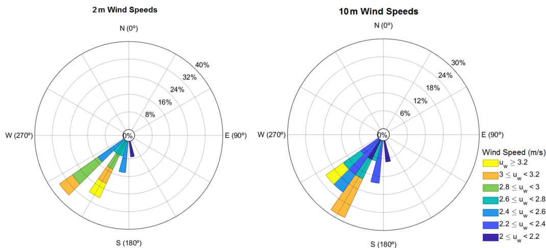
Figure 5. Wind roses for Kumasi Airport for March 2025.
