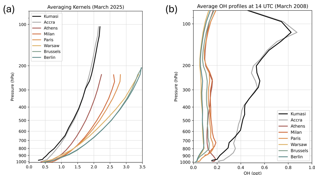
Figure 11. (a) Tropospheric averaging kernels from TROPOMI over selected cities, averaged over March 2025. (b) Average OH profiles around satellite overpass time from TM5-MP simulations at 1^\circ \times 1^\circ resolution for March 2008.
