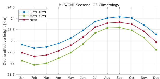
Figure 3. Seasonal climatology of ozone effective height derived from MLS/GMI data for the latitude bands 35–40° N (blue) and 40–45° N (green), along with their mean (red), which is considered more representative for the latitude of LAP.AUTH.
