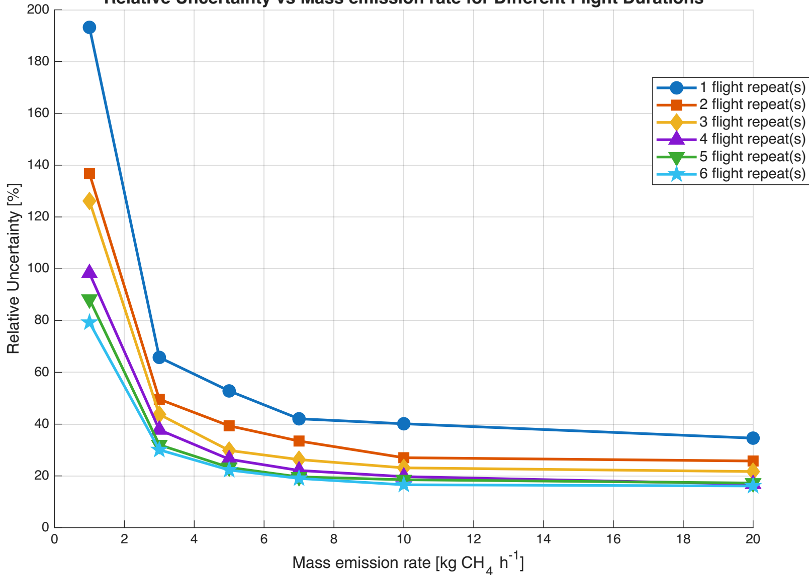
Relative Uncertainty vs Mass emission rate for Different Flight Durations
