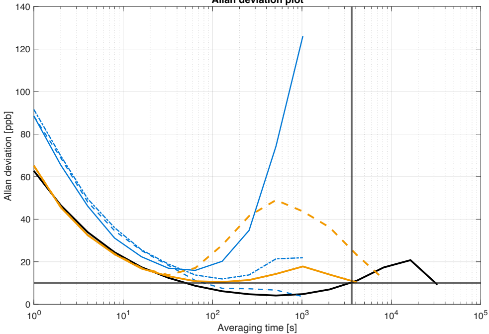
Allan deviation plot
