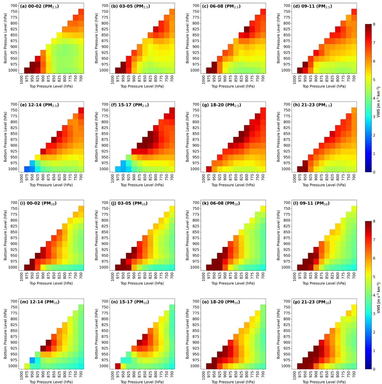
Figure 12. Same as Fig. 11, but under clean days.
