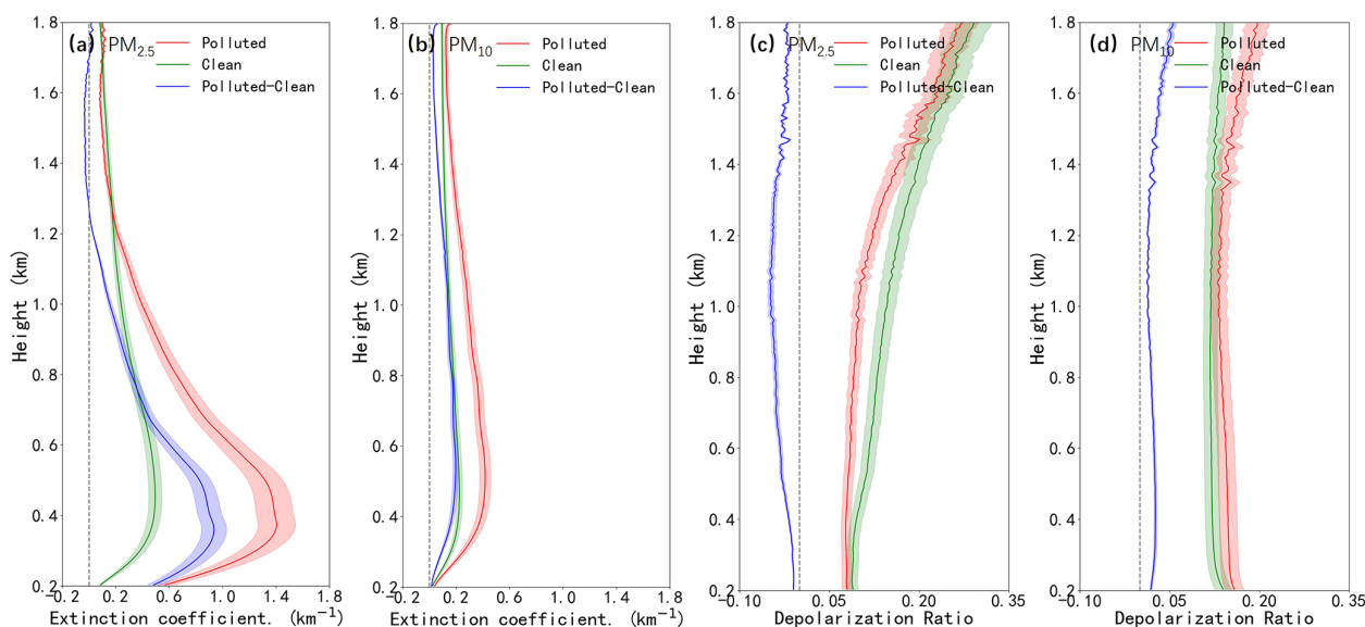
Figure 7. Vertical profiles of aerosol (a, b) extinction coefficient and (c, d) depolarization ratio at 532 nm for (a, c) PM 2.5 in winter and (b, d) PM 10 in spring on polluted, clean days, and the difference between the two. The gray dashed line represents the zero line. Note: The extinction coefficient and depolarization ratio of individual polluted and clean days are positive physical quantities. Negative values in the “Polluted-Clean” panels indicate that the aerosol optical parameters (extinction coefficient or depolarization ratio) are higher on clean days than on polluted days. All data are presented in Beijing time (BJT = UTC + 8 h) for the 532 nm channel.
