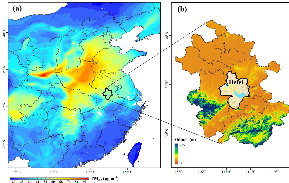
Figure 1. The spatial distribution of (a) the averaged PM 2.5 concentration during winter from 2021 to 2023 (Ministry of Environmental Protection in China, https://air.cnemc.cn:18007/ , last access: 5 January 2025) and (b) the location of the study area (Hefei, China). The digital elevation model (DEM) data are derived from the NASA Shuttle Radar Topography Mission (SRTM) 30 m product ( https://glovis.usgs.gov/ , last access: 15 January 2025), and the land use map of the study area is obtained from the 30 m resolution annual China Land Cover Dataset (CLCD) dataset. The monitoring station is marked by the blue dot.
