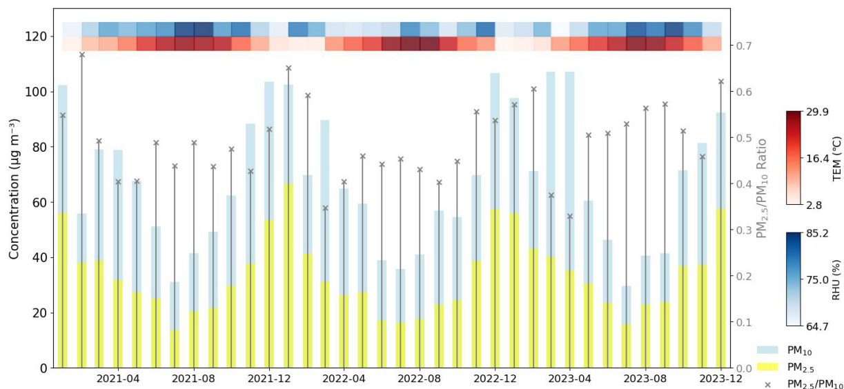
Figure 2. Monthly variation of PM 2.5 (marked as the yellow bars) and PM 10 (marked as the blue bars) concentrations, PM 2.5 /PM 10 ratio (the grey lines with markers on top), temperature (TEM), and relative humidity (RH) during 2021–2023 in Hefei (Beijing time, BJT = UTC + 8 h).
