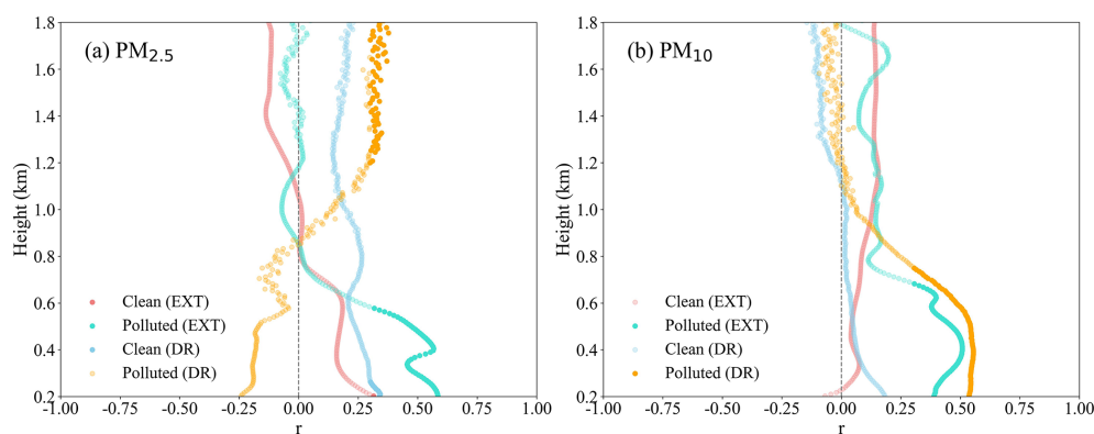
Figure 9. Vertical distributions of correlation ( r ) between aerosol optical properties (532 nm) and ground-based pollutants ( a : PM 2.5 in winter, b : PM 10 in spring) on clean and polluted days. EXT = extinction coefficient; DR = depolarization ratio. The gray dashed line represents the zero line.
