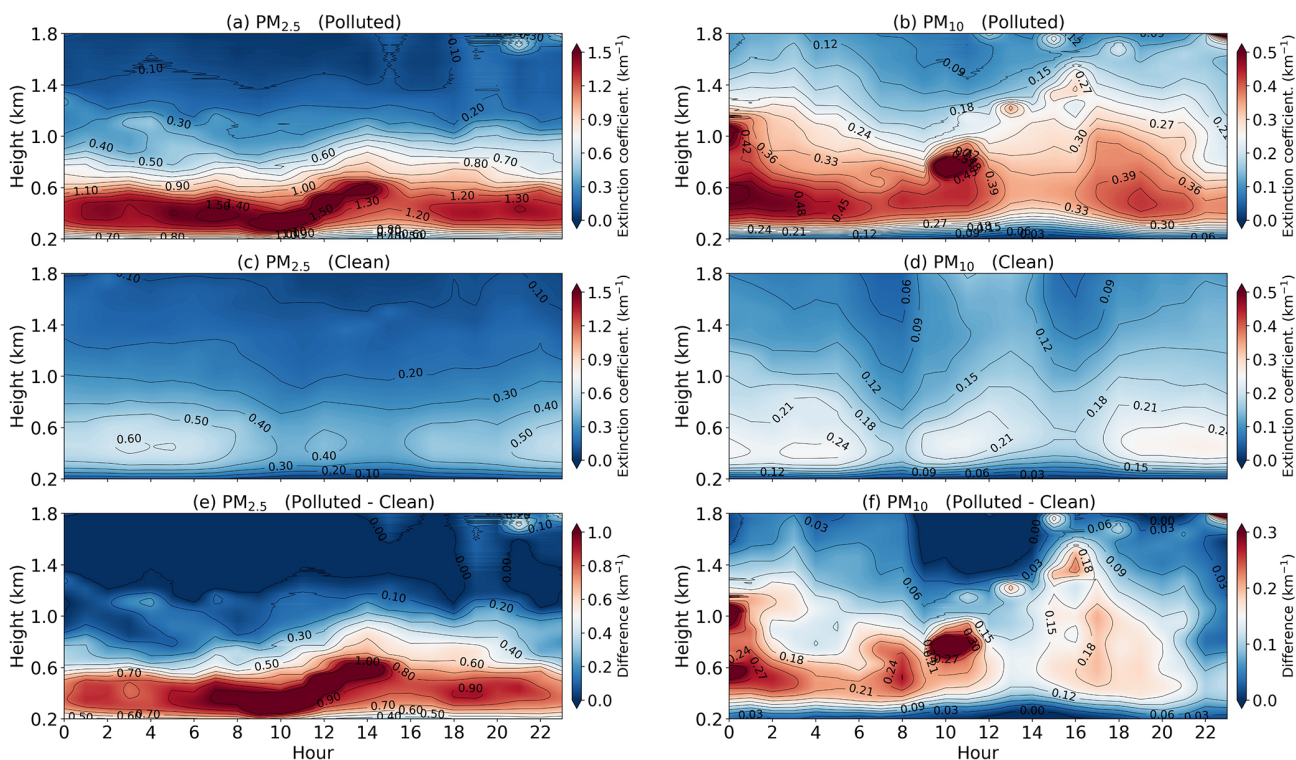
Figure 5. Diurnal variation in the vertical distribution of aerosol extinction coefficient (Winter days for PM 2.5 : First column; Spring days for PM 10 : Second column) under days with (a, b) polluted, (c, d) clean, and (e, f) the difference between the two. All data are presented in Beijing time (BJT = UTC + 8 h) for the 532 nm channel.
