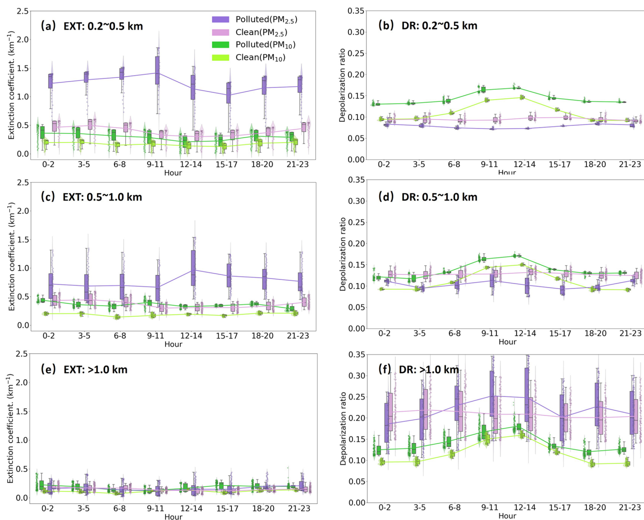
Figure 8. Diurnal variations of (EXT: a , c , and e ) extinction coefficient and (DR: b , d , and f ) depolarization ratio at 532 nm on polluted and clean days for PM 2.5 and PM 10 at ( a , b ) 0.2–0.5 km, ( c , d ) 0.5–1.0 km, and ( e , f ) above 1.0 km, respectively. The whiskers represent the 90th and 10th percentiles, respectively. The shaded areas represent the 25th–75th percentiles. The connected lines depict the trend of mean values across different heights. All data are presented in Beijing time (BJT = UTC + 8 h) for the 532 nm channel.
