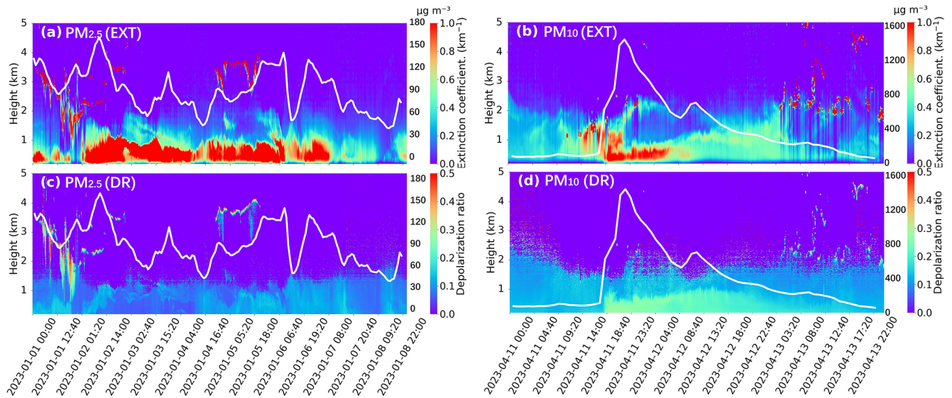
Figure 10. Pollution Episodes: Temporal dynamics of (a, b) extinction and (c, d) depolarization parameters for the 532 nm channel during severe (a, c) PM 2.5 (1–8 January 2023) and (b, d) PM 10 (11–13 April 2023) periods in Hefei. The white lines represent the hourly (a) PM 2.5 and (b) PM 10 concentrations, with their scale on the secondary y-axis. All data are presented in Beijing time (BJT = UTC + 8 h). EXT = extinction coefficient; DR = depolarization ratio.
