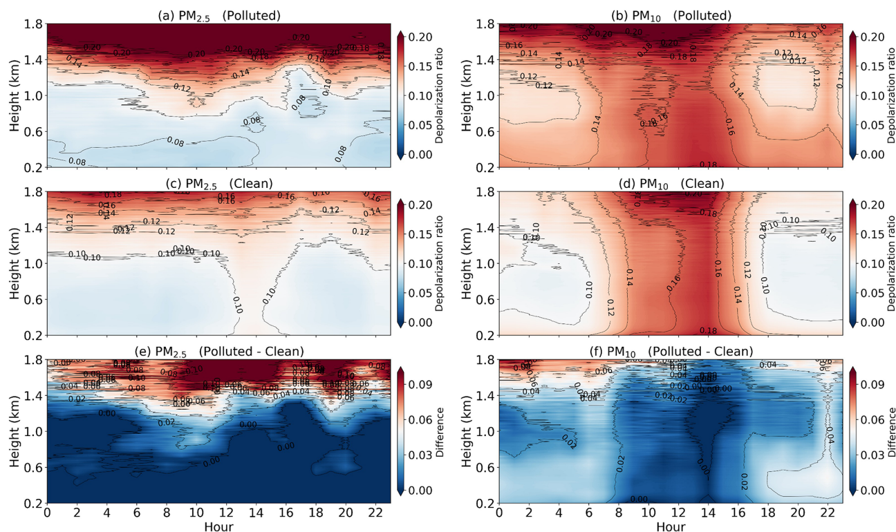
Figure 6. Same as Fig. 5, but for depolarization ratio.
