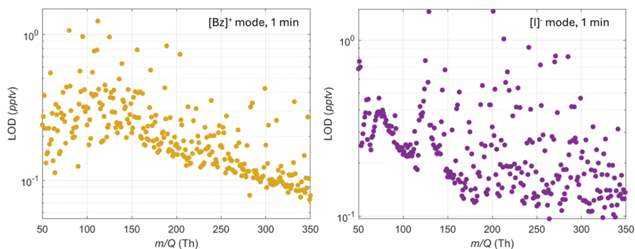
Figure 4. Limits of detection ( 3\sigma ) for chemical ionization using [\text{Bz}]^+ and [\text{I}]^- reagent ions across the mass spectrum assuming ionization is collision limited and a standard sensitivity in 1 min of 30 \text{ ncps pptv}^{-1} .
