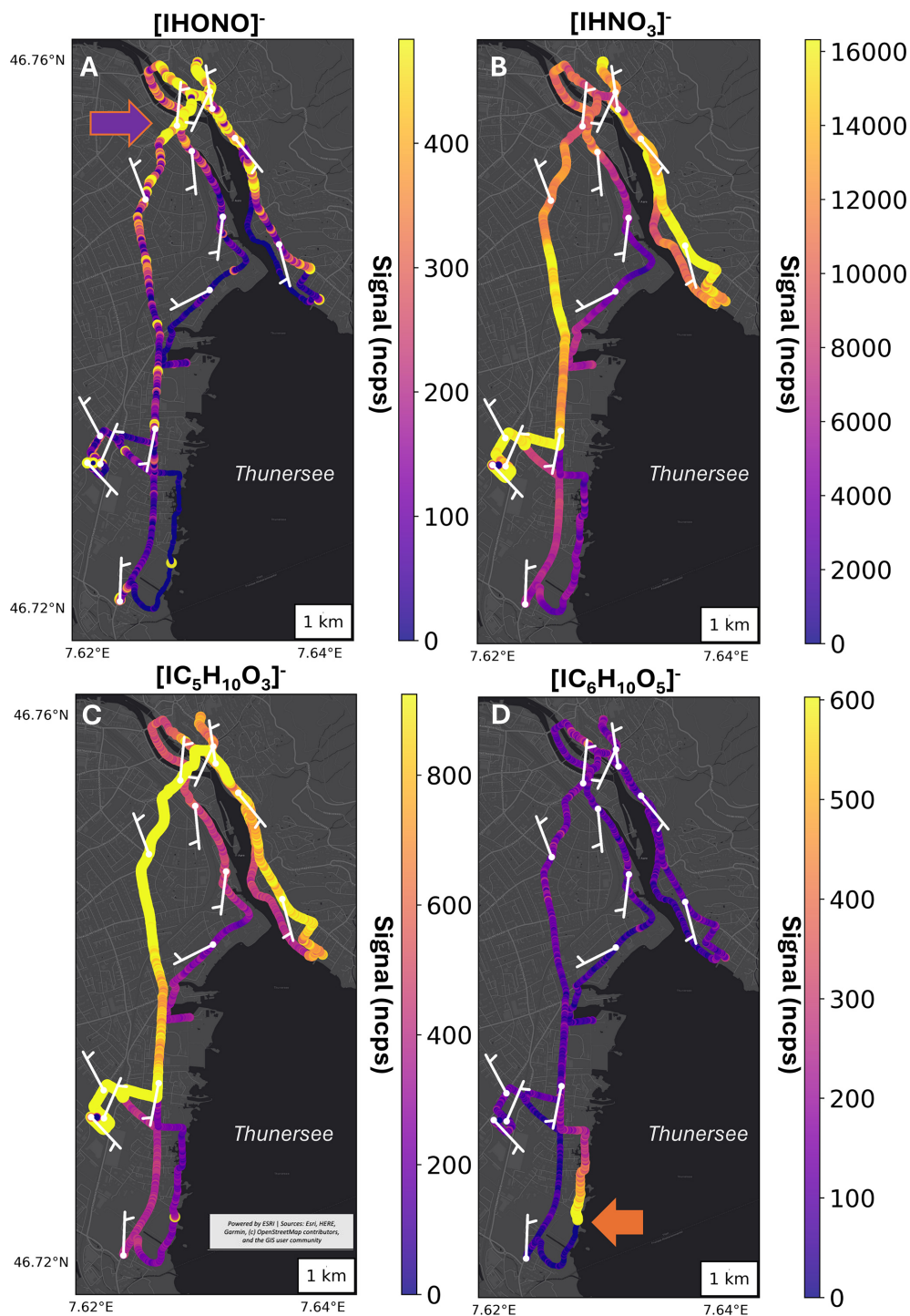
Figure 6. e-Bike Deployment Data of Portable-TOF-CIMS in Iodide ion Mode overlaid with wind barbs and signal profiles of different key pollution species with colormap in units of normalized cps (a) Signal profile of m/Q consistent with iodide ion adduct with nitrous acid (173.905 Th) and purple arrow pointing to major bus station in Thun. (b) Signal profile of m/Q consistent with iodide ion adduct with nitric acid (189.900 Th). (c) Signal profile of m/Q consistent with C_5H_{10}O_3 (244.967 Th) adduct with iodide ion. (d) Signal profile of m/Q consistent with C_6H_{10}O_5 (288.967 Th) adduct with iodide ion. Estimated sensitivities are: 22, 30, 30, and 30 ncps pptv -1 for [IHONO]^- , [IHNO_3]^- , [IC_5H_{10}O_3]^- , [IC_6H_{10}O_5]^- , respectively. Further information on sensitivities are shown in Table S2. Maps: Sources: Esri, HERE, Garmin, © OpenStreetMap contributors, and the GIS user community | Powered by Esri.
