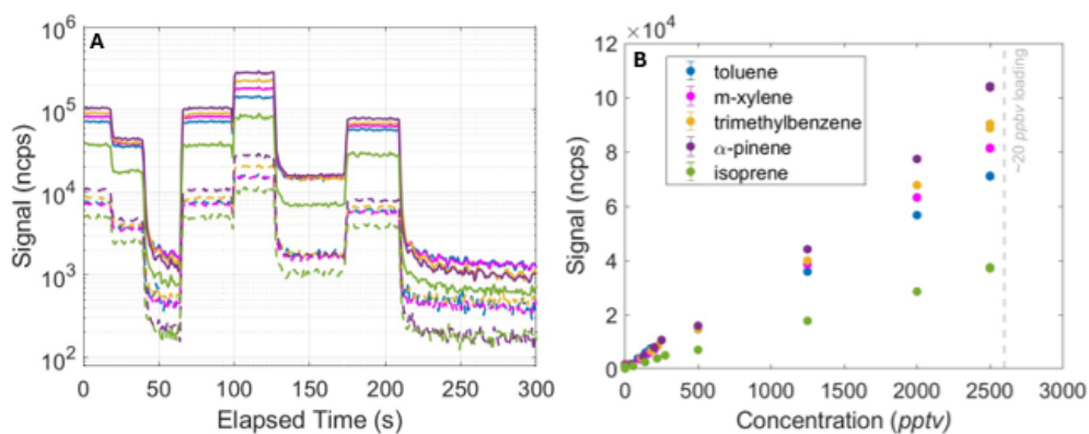
Figure 2. (a) Calibration sequence using a custom calibration gas mixture in [\text{Bz}]^+ ionization mode, C13 isotopes traced with dashed lines, normalized by reagent ion signal and multiplied by 1 \times 10^6 . (b) Calibration curve for toluene, m-xylene, trimethylbenzene, \alpha -pinene, and isoprene adduct in [\text{Bz}]^+ ionization mode calculated from time averages in panel (a) at concentrations that are within the linear response range (retainment of 60 % of reagent ion signal).
