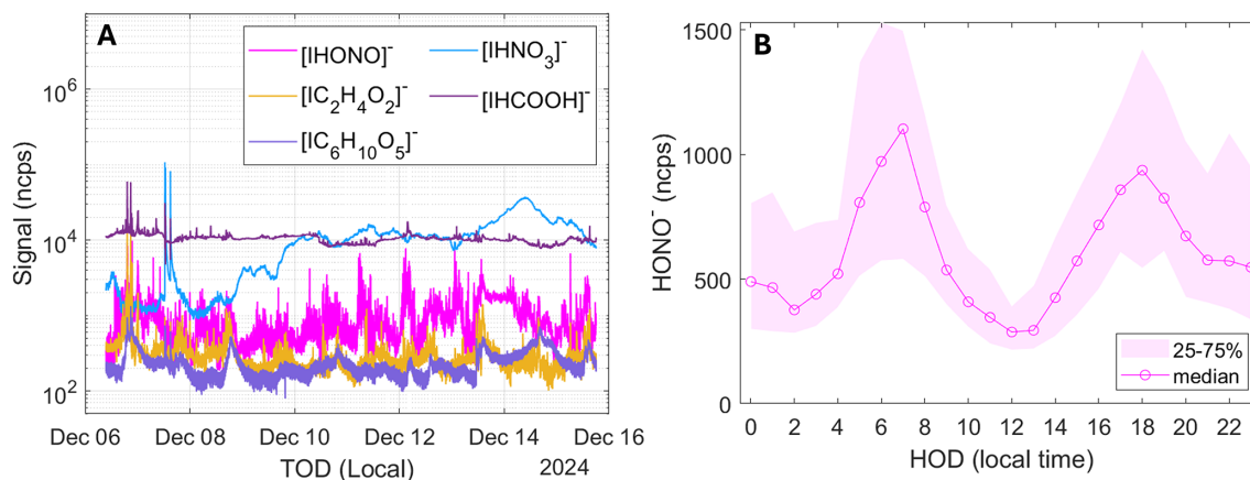
Figure 5. (a) Stationary measurements of key air pollutants for tracing anthropogenic activity with continuous measurements for 10 d using iodide ion chemical ionization. (b) Diurnal cycle using [\text{IHONO}]^- Signal averaged hourly. Sensitivities are: 22, 30, 3.4, 8.4 and 30 \text{ ncps pptv}^{-1} for [\text{IHONO}]^- , [\text{IHNO}_3]^- , [\text{IC}_2\text{H}_4\text{O}_2]^- , [\text{IHCOOH}]^- , [\text{IC}_6\text{H}_{10}\text{O}_5]^- , respectively. Further information on sensitivities are shown in Table S2.
