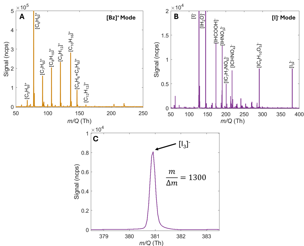
Figure 3. (a) Normalized high-resolution mass spectrum of a calibration gas over lab air in [\text{Bz}]^+ mode with labelled analyte signals. (b) Normalized high-resolution mass spectrum of air measurements in the field in iodide anion mode with labelled analyte signals. (c) Zoom in on \text{I}_3^- cluster signal illustrating representative peak widths for the high-resolution mass spectrum in Fig. 3b.
