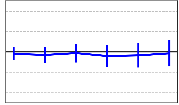
Forecast Day
