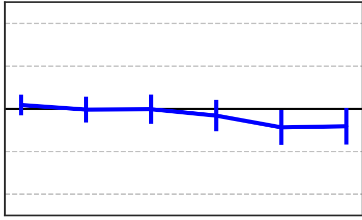
Forecast Day
