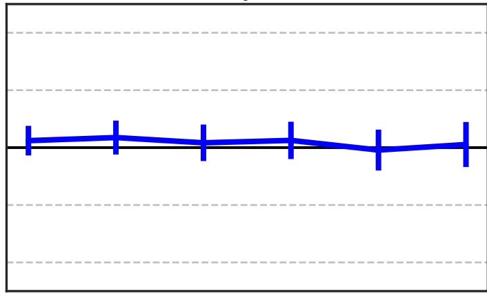
Tropics
