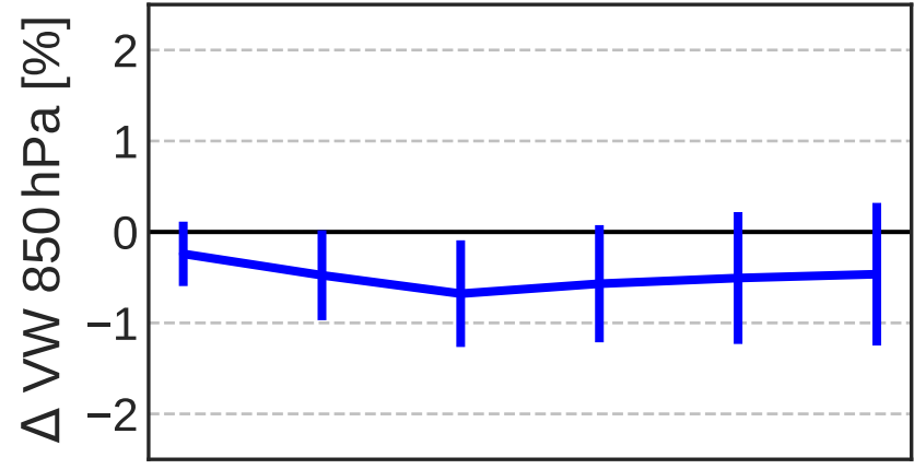
Forecast Day
