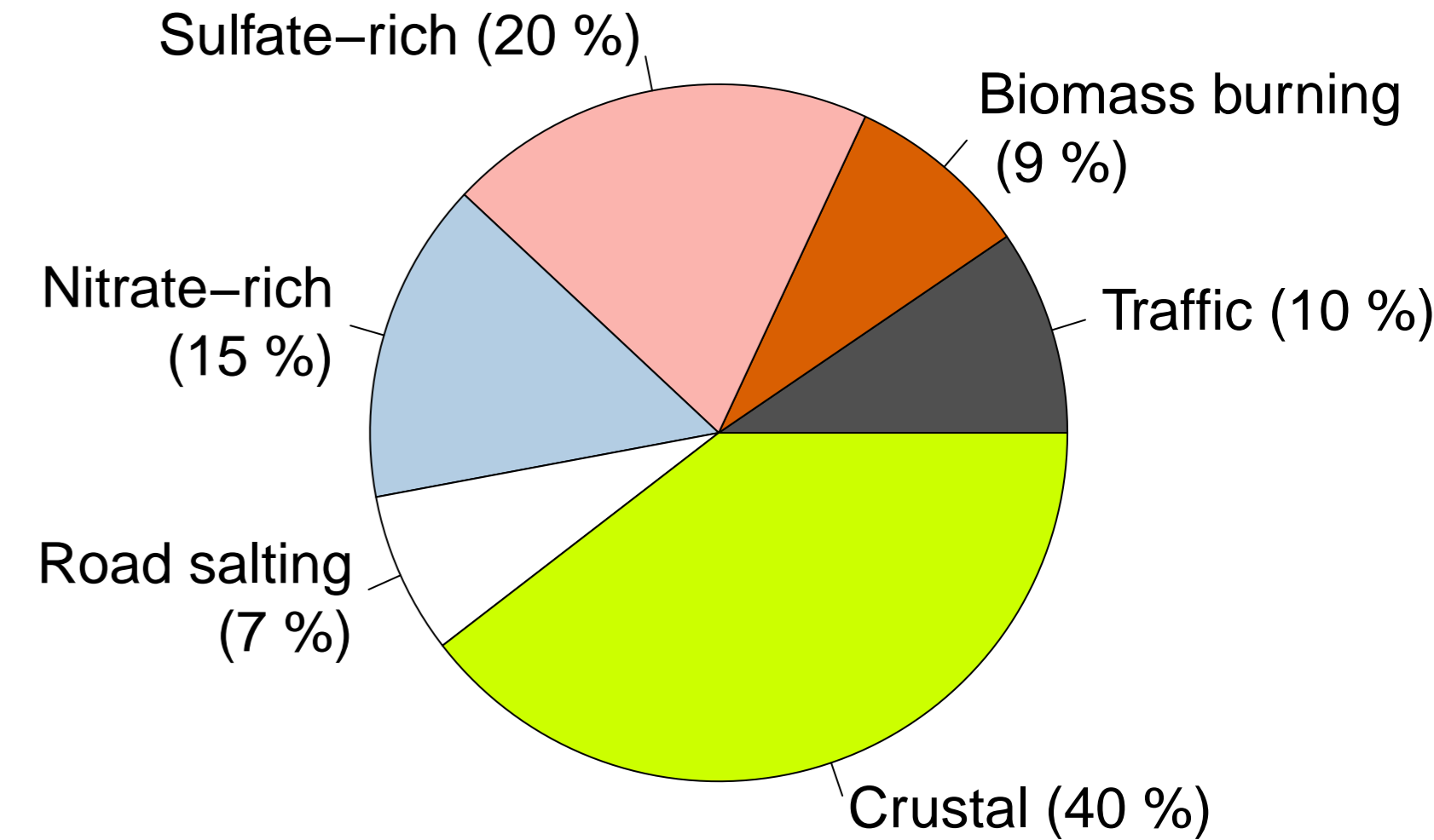
(c) Chemical source apportionment (data set 1, 2020–2021)
