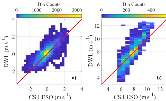
Figure 8. Cumulative scatter plots compare LESO-based CopterSonde (CS) vertical wind (a) and horizontal wind (b) estimates against Doppler wind Lidar (DWL) measurements, aggregating data from 16 vertical profiles ( N=31\,386 data points). The color density in each plot indicates the frequency of observations, and a red one-to-one line marks perfect agreement. Prior to analysis, outliers from low DWL signal-to-noise ratios were removed. The correlation coefficient ( R ), mean difference (MD), standard deviation (SD), and RMSE for each panel are: (a) vertical wind with R=0.791 , MD=-0.197\text{ m s}^{-1} , RMSE=0.492\text{ m s}^{-1} , and SD=0.451\text{ m s}^{-1} ; (b) horizontal wind speed with R=0.90 , MD=-0.287\text{ m s}^{-1} , RMSE=1.025\text{ m s}^{-1} , and SD=0.984\text{ m s}^{-1} .
