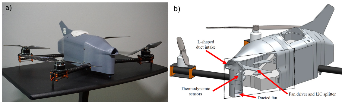
Figure 2. (a) CopterSonde-3D concept developed in early 2022. This quadcopter UAS is designed for thermodynamic observations and vertical profiling of the lower atmosphere. Its distinctive shape results from an optimized internal layout that enhances airflow across the sensors via a wind vane flight mode. (b) Section cut of the front shell from the CopterSonde-3D CAD model, illustrating the solar shield and sensor compartment design, along with the placement of the thermodynamic sensors and other critical components. The dotted rectangle marks the plane of the cut.
