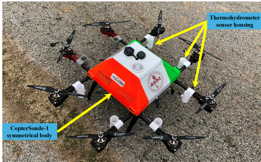
Figure 1. CopterSonde-1 concept made in early 2017. An H-frame octocopter UAS with thermohydrometer sensors distributed in a symmetrical arrangement around the main body. The atmospheric sensors were housed and protected inside white plastic tubes and mounted on the UAS's arms below the rotors, shown by the yellow arrows pointing to some of the sensors.
