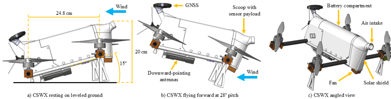
Figure 4. (a) Right-side view of the CopterSonde-SWX (CSWX) resting on level ground and typical orientation during hover conditions in calm wind. Key dimensions are provided for scale. The wind-direction arrow is included for reference, clearly indicating the front and rear of the platform and highlighting the typical flight heading of the CSWX during vertical atmospheric profiling. (b) Side view of the CSWX in forward-flight configuration, exhibiting a 28^\circ pitch angle to counteract wind-induced drag. In this configuration, the aerodynamic profile of the CSWX effectively reduces air resistance, which is the primary purpose of the inclined body design. External components, such as the GNSS antenna and air intake, align with the wind vector, further enhancing aerodynamic efficiency. (c) Angled perspective view of the CSWX, providing a three-dimensional visualization of the UAS and its structural components.
