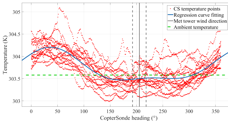
Figure A1. Scatter plot of temperature observations against the aircraft's heading collected with the CS3D while hovering and rotating with a constant angular speed of 2 rpm. The mean ambient temperature and wind direction were computed using observations from a nearby meteorological tower during the flight. The vertical dashed lines represent 3 times the standard deviation of the measured wind direction. The blue line represents the best-fit polynomial curve.
