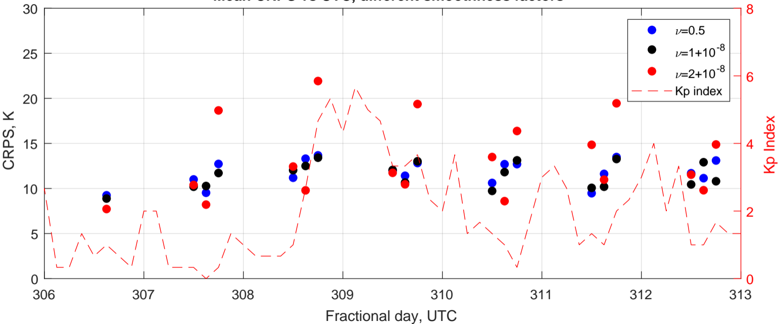
Mean CRPS vs UTC, different smoothness factors
