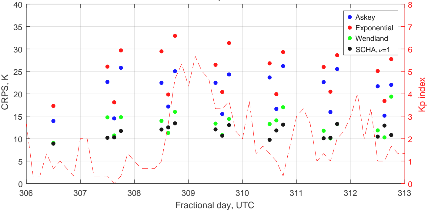
Mean CRPS vs UTC, different kernels
