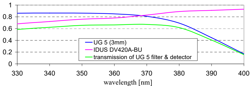
c) Combined effect of UG 5 filter and detector quantum efficiency
