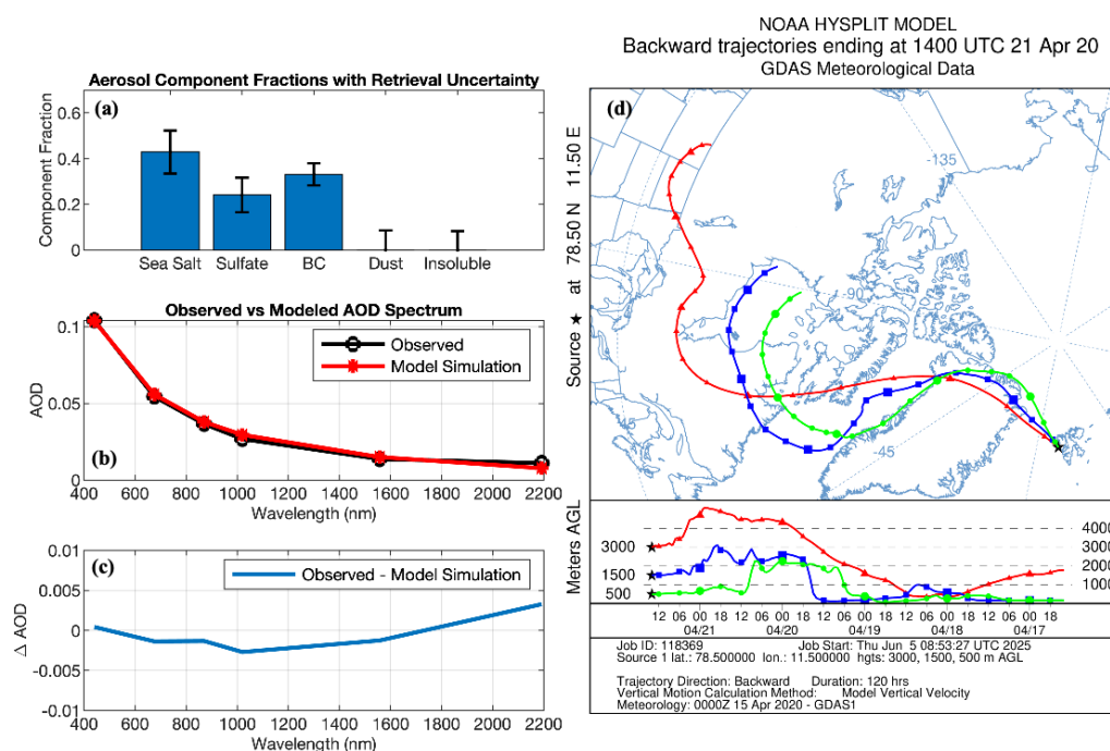
Figure 6. Aerosol composition retrieval from ground-based observations at Ny-Ålesund on 21 April 2020. (a) Retrieved aerosol component number concentration fractions (sea salt, sulfate, black carbon, dust, and insoluble aerosols) with uncertainties. (b) Observed versus modeled AOD spectra. (c) Residual differences between observed and simulated AOD. (d) 120 h backward trajectories arriving at Ny-Ålesund (78.9° N, 11.9° E) at altitudes of 500, 1500, and 3000 m above ground level, computed using the NOAA HYSPLIT model (Stein et al., 2015).
