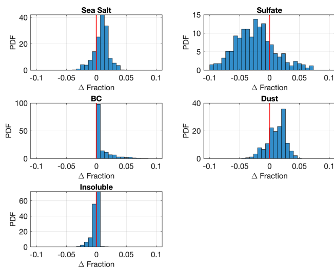
Figure 5. Distributions of relative changes in the retrieved aerosol component fractions from the sensitivity tests described in Sect. 3.6. Four auxiliary parameters ( SSA_{440} , AF_{440} , Reff , RH ) are perturbed, and deviations from the baseline retrieval are shown for each aerosol fraction. Red vertical lines indicate zero deviation.
