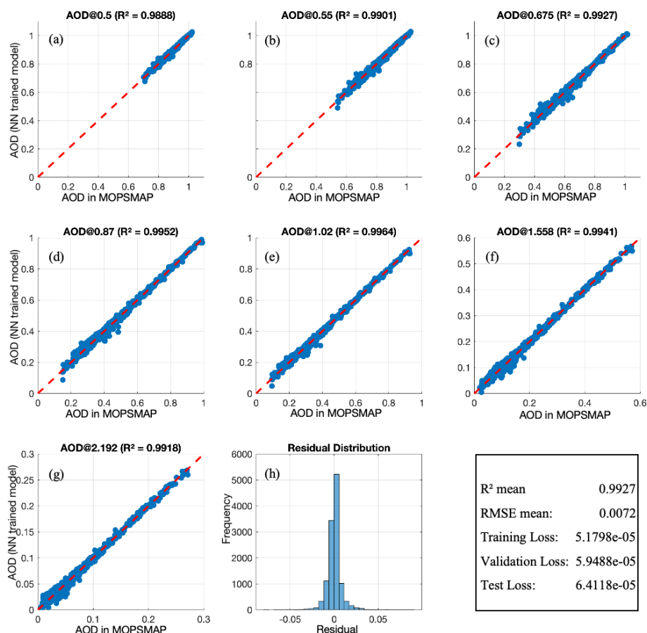
Figure 4. Performance evaluation of the machine learning model replacing MOPSMAP as the forward model. Panels (a)–(g) show scatter plots comparing the predicted normalized AOD from machine learning model with the normalized AOD from MOPSMAP at different wavelengths (0.5, 0.55, 0.675, 0.87, 1.02, 1.558, and 2.192 \mu\text{m} ). The red dashed line represents the 1 : 1 reference line. Panel (h) displays the residual distribution of the predicted AOD values. The table summarizes key performance metrics, including the mean R^2 , RMSE, and loss values for training, validation, and testing.
