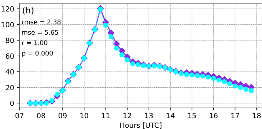
Ice
