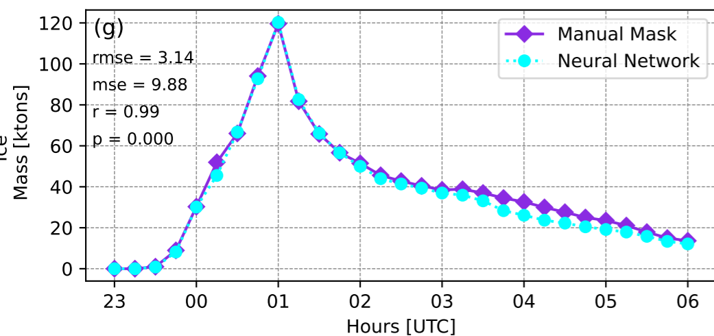
Ice
