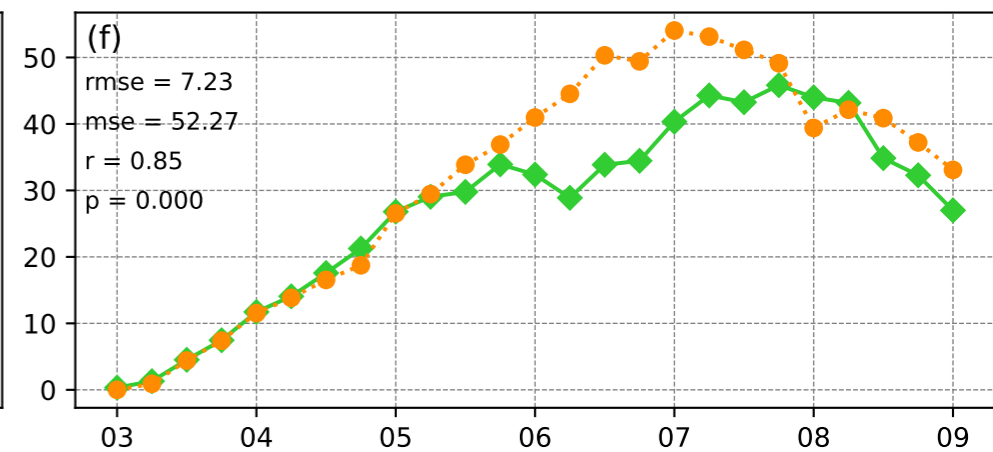
Ice
