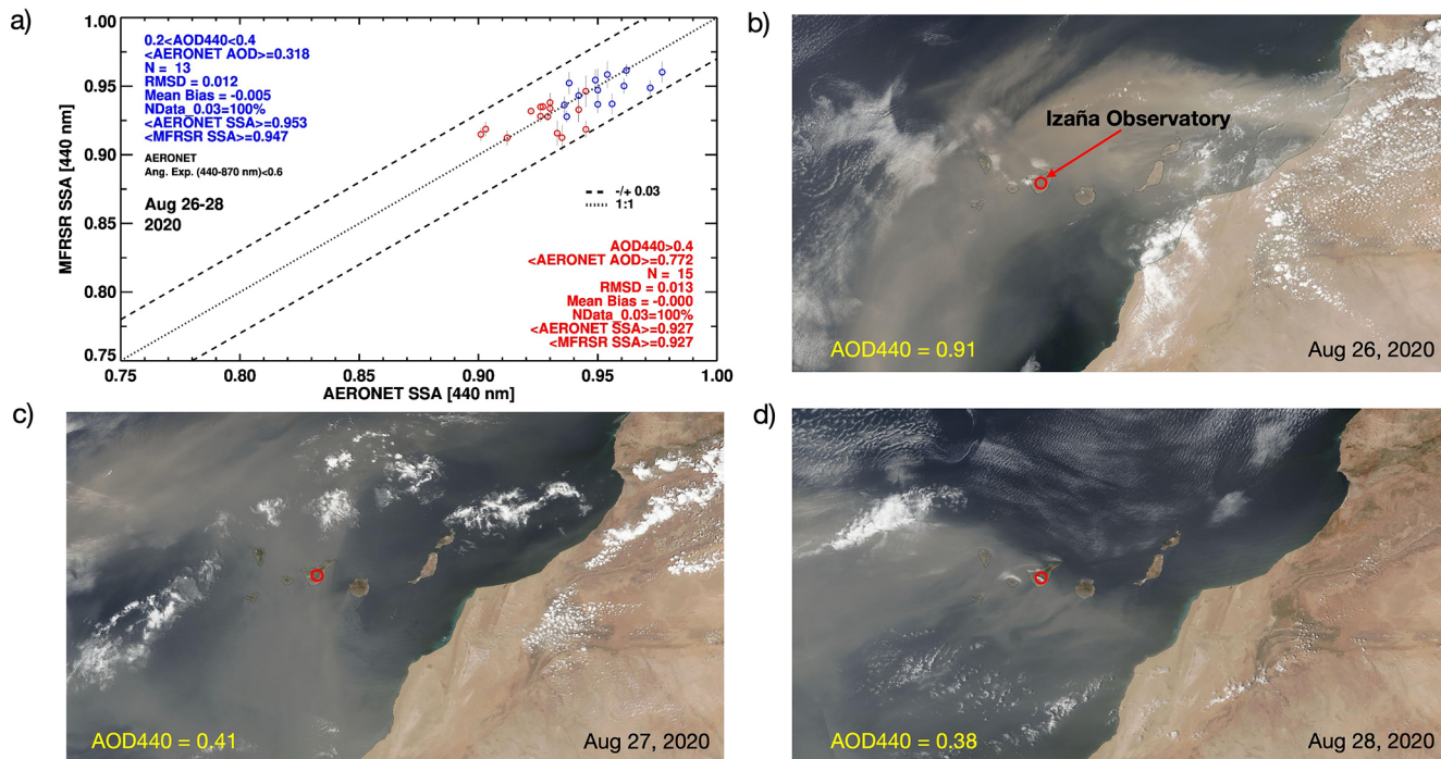
Figure 10. (a) Comparison of the MFRSR vs. AERONET derived SSA at 440 nm for the data acquired on 26, 27, and 28 August 2020. Blue and red circles represent temporally matched data with coincident AERONET-measured AOD (440 nm) 0.2–0.4 and > 0.4, respectively. The statistics of the comparison for different AOD conditions are included within the plots. The true-color RGB images acquired from Suomi-NPP/VIIRS sensor for three dates are shown in panels (b), (c), and (d).
