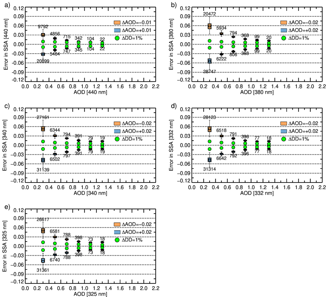
Figure 8. Same as in Fig. 7 but for the MFRSR-derived spectral SSA.
