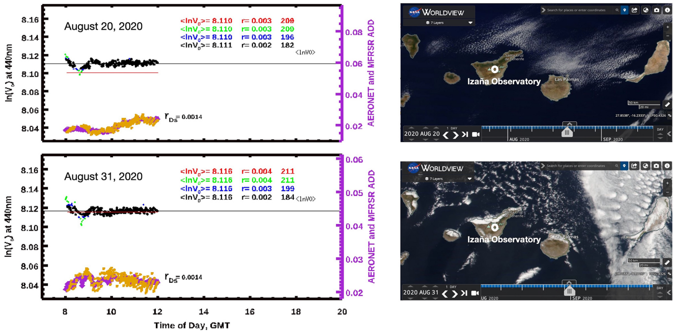
Figure 3. Examples of MFRSR Step 1 calibration plots on the cleaner days of 20 and 31 August 2020, when AERONET-measured AODs (440 nm) were quite lower ( < 0.03 ) (left). The logarithm of V_0 is shown against the left-hand y-axis as red-green-blue-black dots. The different colors show the effect of the iterative removal of V_0 outliers outside of 3\sigma standard deviation. The measured AODs from AERONET and the MFRSR instruments are shown as purple and orange dots, respectively, against the righthand y-axis. The MODIS true-color RGB images for the corresponding days showing a virtually aerosol-free atmosphere (right).
