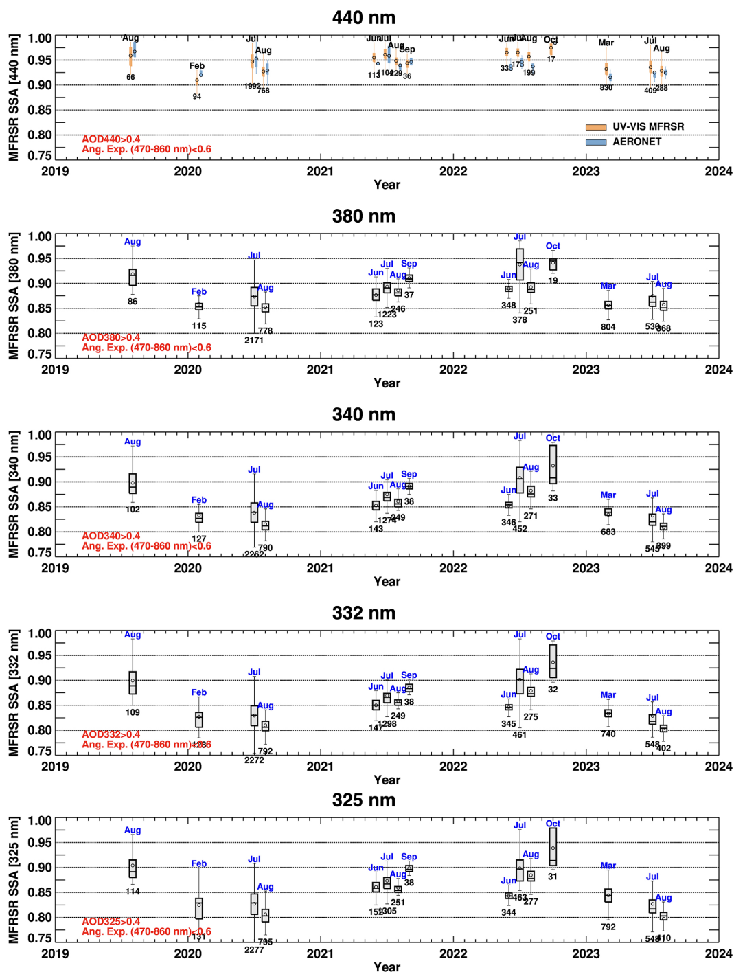
Figure 14. Monthly time-series charts of MFRSR-derived spectral SSAs. The data are represented as box and whisker plot; grey boxes and whiskers represent 25th–75th percentile range and 1.5 times the interquartile range, respectively. Data with AERONET AOD at respective wavelengths > 0.4 and Extinction Ångström Exponent < 0.6 are presented.
