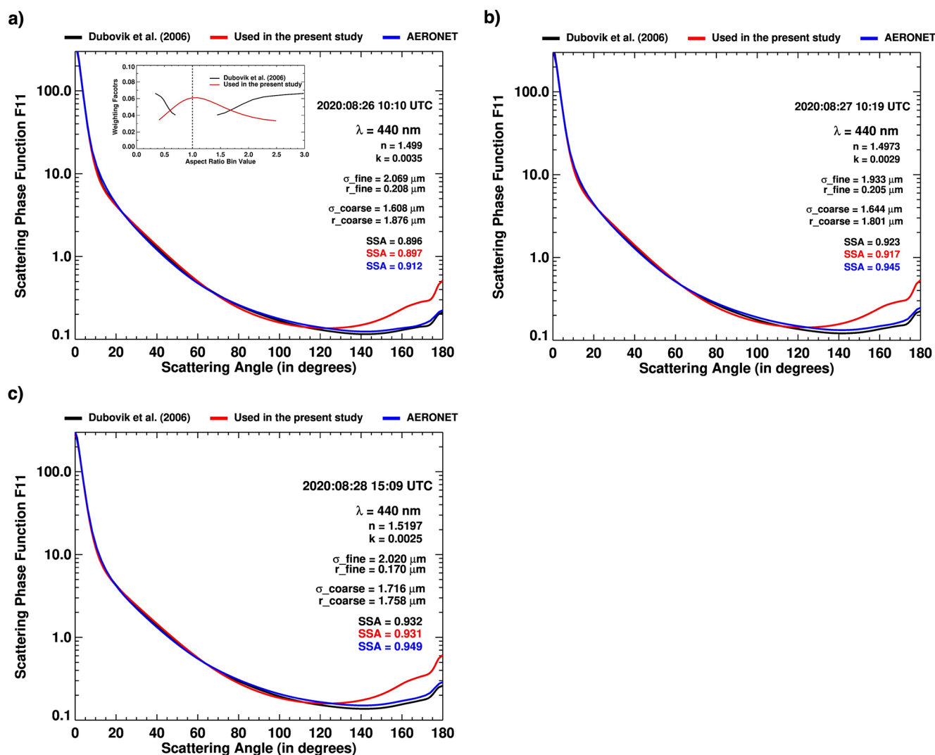
Figure 5. Scattering phase function F_{11} (440 nm) of mineral dust aerosols retrieved on (a) 26 August at 10:10 UTC, (b) 27 August at 10:19 UTC, and (c) 28 August at 15:09 UTC of 2020 corresponding to randomly oriented spheroids proposed in Dubovik et al. (2006) (black), empirically derived distribution (red) used in the present study, and that from AERONET inversion product (blue). F_{11} (except for AERONET) was simulated using the modified DLS software package for a single MFRSR-AERONET collocated measurement for the respective dates. Dust aspect ratio distribution (black curves; Dubovik et al., 2006) and OMI empirical aspect ratio distribution used in the presented study (red curve) are shown as an inset in panel (a).
