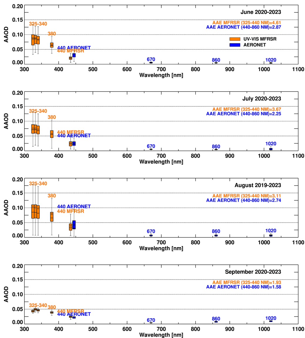
Figure 17. As in Fig. 15 but for the derived spectral aerosol absorption optical depth (AAOD). The aerosol Absorption Ångström Exponent (AAE) values calculated separately for UV and VIS-NIR wavelength ranges are also included in each AAOD plot.
