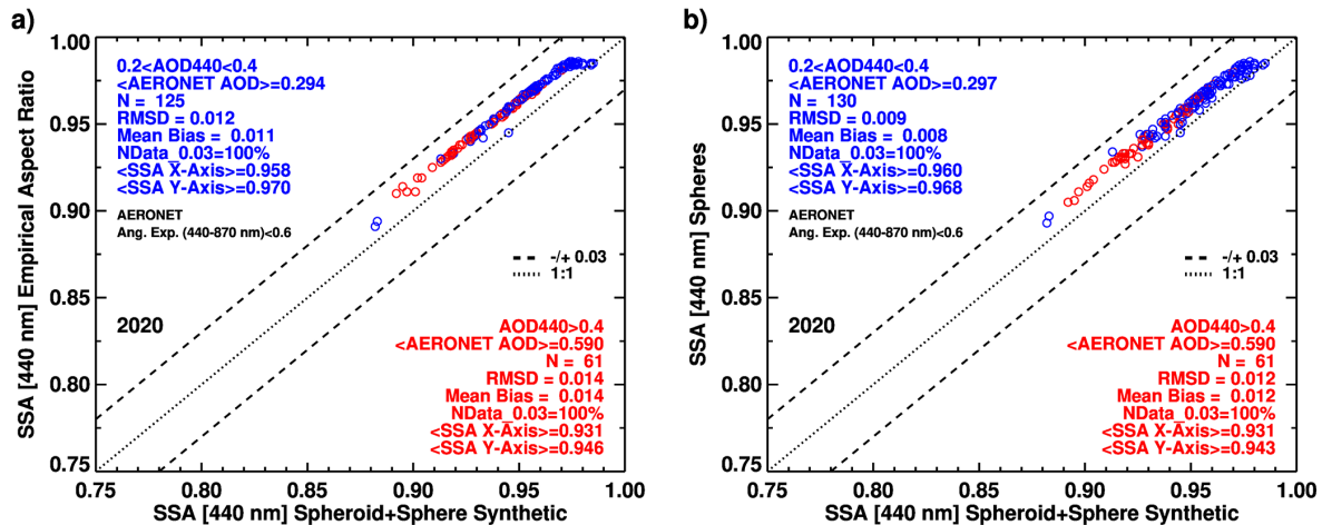
Figure 9. Comparison charts of SSA (440 nm) derived assuming (a) empirical aspect ratio and (b) spherical particles against those retrieved assuming AERONET-like spheroid-sphere combined approach. The synthetic diffuse-to-direct downwelling irradiance ratio simulated using actual AERONET Lev 1.5 inversion dataset collected at the Izaña site were treated as measurements in the inversion process. SSA matchup data points in blue and red represent the coincident AOD 440 conditions of 0.2–0.4 and > 0.4, respectively. The statistics of the comparison for different AOD conditions are included within the plots.
