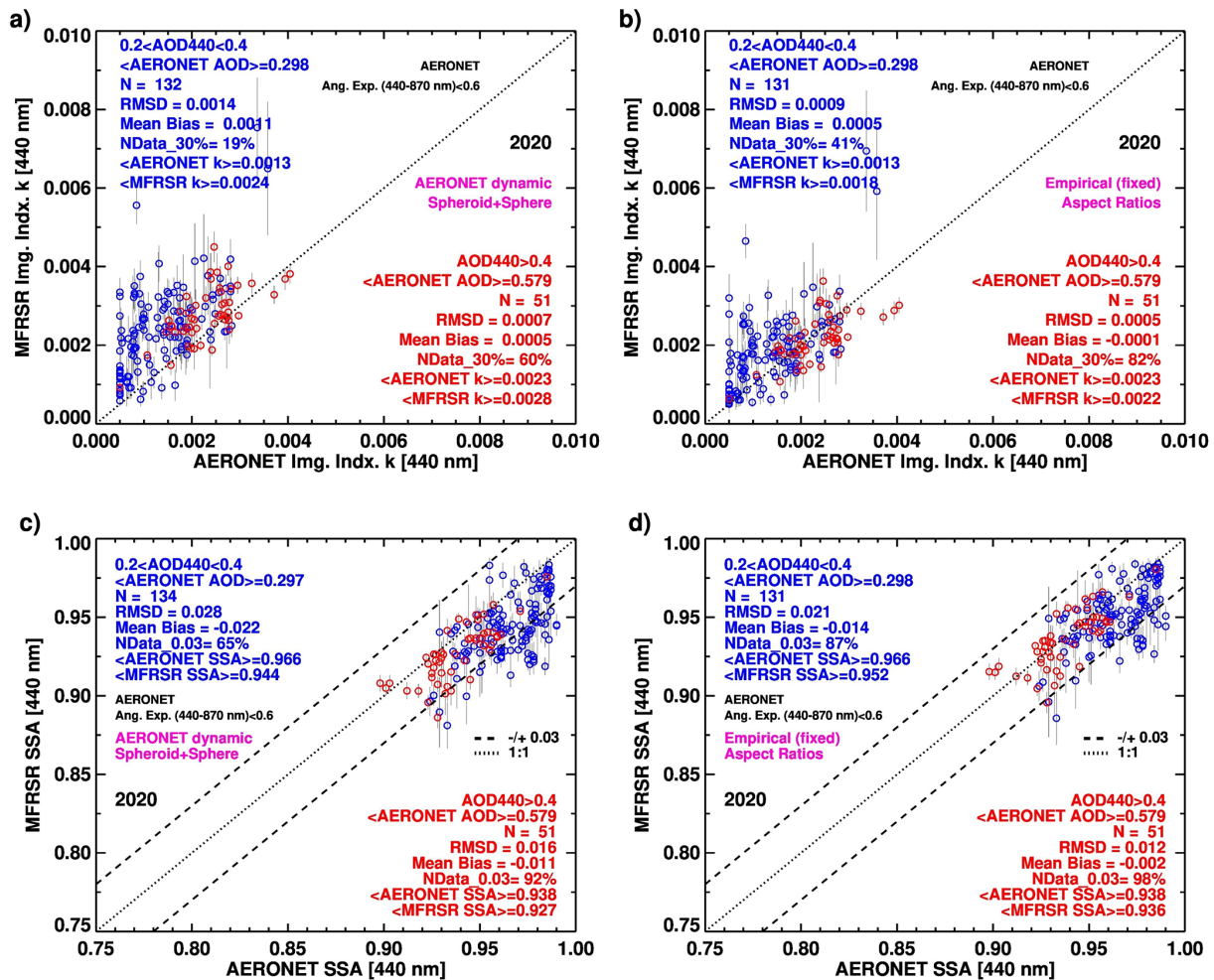
Figure 12. Comparison of MFRSR (y-axis) vs. AERONET (x-axis) collocated imaginary part of the refractive index (a, b) k and SSA (c, d) at 440 nm for the matchup data collected during 2020 at Izaña site derived assuming AERONET-like “mixing” approach (a, c) combining sphericity-weighted randomly oriented spheroid (Dubovik et al., 2006) and sphere, and empirically derived aspect ratios (b, d) adopted in the over-ocean dust aerosol models used for near-UV aerosol algorithm of OMI, EPIC, and TROPOMI sensors. SSA matchup data points in blue and red represent the coincident AOD_{440} conditions of 0.2–0.4 and > 0.4 , respectively. The statistics of the comparison for different AOD conditions are included within the plots.
