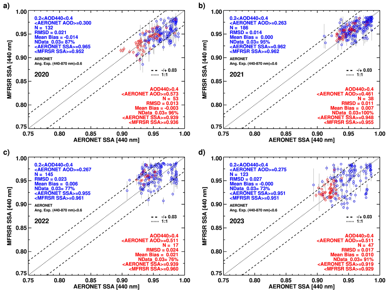
Figure 13. Comparison of MFRSR (y-axis) vs. AERONET (x-axis) SSA at 440 nm for the 2020–2023 (a–d) operation period of MFRSR measurements at Izaña site derived assuming empirically derived aspect ratios. Matchup data points in red (blue) represent AOD_{440} > 0.4 ( 0.2 < AOD_{440} < 0.4 ) conditions. The statistical measures of the comparison are included within individual plot.
