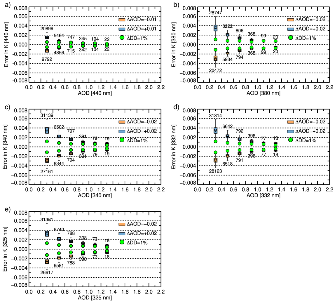
Figure 7. Errors in the MFRSR-retrieved spectral imaginary part of the index ( k ) resulting from (1) the uncertainties in the AERONET-measured AOD (orange and blue boxes) and (2) 1% change in the MFRSR-measured diffuse-to-direct irradiance ratio (filled green circles). Data represent MFRSR record from 2019–2023. Box-and-whisker elements indicate the interquartile range (25th–75th percentiles; boxes) and 1.5 times IQR (whiskers); mean values are shown as open circles and median values as horizontal lines.
