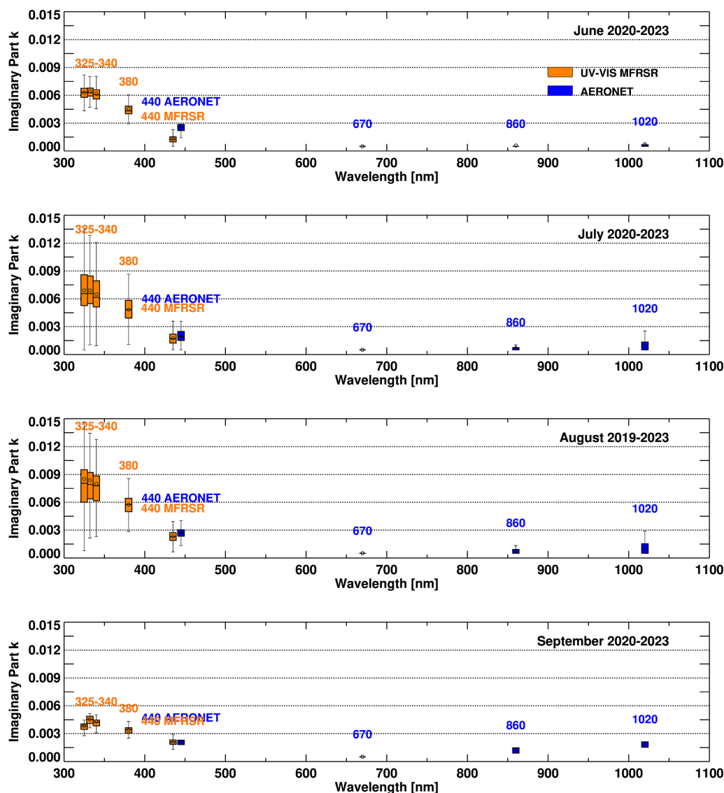
Figure 15. Spectral plots of the imaginary part of the refractive index retrieved from the MFRSR (325–440 nm) and AERONET (440–1020 nm) instruments. The spectral SSA dataset represents AE < 0.6 and AOD_{440} > 0.4 conditions and are shown as a box-whisker plot for each wavelength separately for the months of June, July, August, and September 2019–2023 in top to bottom order.
