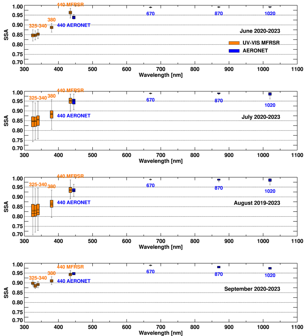
Figure 16. Same as in Fig. 15 but for the derived spectral SSA.
