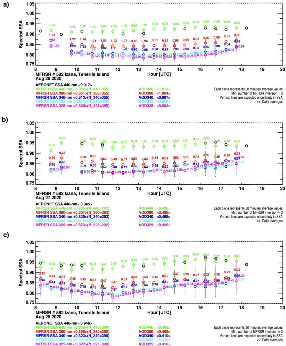
Figure 11. Sub-hourly spectral SSA derived from UV-VIS MFRSR observations acquired on 26, 27, and 28 August (a, b, c, respectively) of 2020. Each circle represents 30 min averaged SSA values with corresponding averaged AOD printed next to it. Vertical lines represent the expected uncertainty in the derived SSA, which combinedly accounts for both \pm 0.01 – 0.02 uncertainties in the AERONET-measured AOD and a 1 % error in the diffuse to direct irradiance ratio. Daily mean values of SSAs and AODs are printed on the bottom of each plot.
