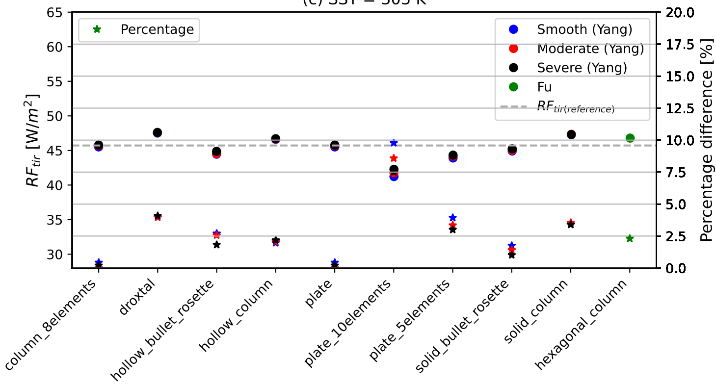
(c) SST = 303 K
