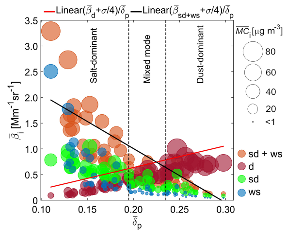
Figure 9. The scatterplot of plume-averaged backscattering ( \overline{\beta}_i ) versus plume-averaged depolarization ratio ( \overline{\delta}_p ) for different particles. Color of the circles indicates particle type: dark red-d, green-sd, blue-ws, and orange-sd+ws. The circle size corresponds to \overline{MC}_i . The Red and black solid lines are fits to (\overline{\beta}_d + \frac{\sigma}{4})/\overline{\delta}_p and (\overline{\beta}_{sd+ws} + \frac{\sigma}{4})/\overline{\delta}_p . Based on column 2 of Table 3, two black dashed lines separate the regions where dust or salt particles are dominant or a mixture of them is in the detected plume.
