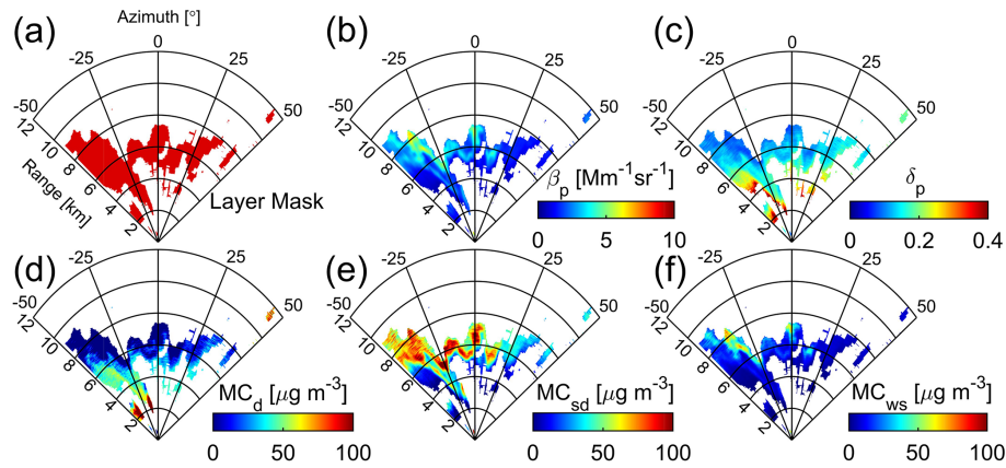
Figure 7. RA series of: (a) the layer mask obtained by applying the MSD algorithm on RCSs recorded by ISPL on 20 September 2022, 07:43–08:28 LT, see Fig. 6a, (b) the particle backscattering coefficient ( \beta_p ), (c) particle depolarization ratio ( \delta_p ), and mass concentration profiles of: (d) dust ( MC_d ), (e) salt-dust ( MC_{sd} ), and (f) wet-salt ( MC_{ws} ).
