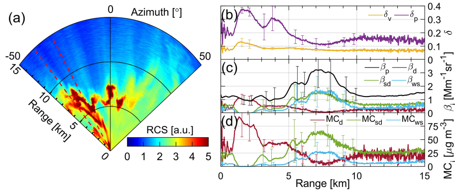
Figure 6. (a) RA series of the ISPL RCSs on 20 September 2022, 07:43–08:28 LT; 20 signals between the two red dashed lines were averaged to retrieve the profiles of (b) the volume linear depolarization ( \delta_v ) and the particle linear depolarization ( \delta_p ) ratios, (c) backscatter coefficient of dust ( \beta_d ), salt-dust ( \beta_{sd} ), wet-salt ( \beta_{ws} ) particles, and their sum ( \beta_p ), (d) mass concentration ( MC_i ) for the same particle types as in (c).
