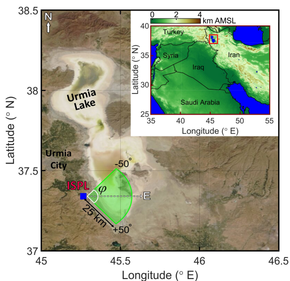
Figure 1. Urmia Lake in Northwest Iran, Terra MODIS true color, 20 September 2022. The blue square on the lake coast is the ISPL station at 37.34° N, 45.29° E, and 1270 m a.m.s.l. The green-shaded area represents the lidar azimuthal coverage over the lake. Inset is the topography map of the region. Terra/MODIS imagery courtesy of NASA LAADS DAAC.
