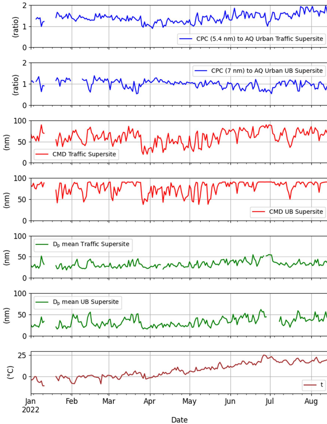
Figure S6. Ratio of the PNC measured with CPCs and AQ Urban sensors at the Traffic Supersite and at the UB Supersite together with CMD (count median diameter) obtained from AQ Urban sensors, mean particle diameter ( D_p ) calculated from DMPS measurements, and temperature during the 7.5-month measurement period. The temperature is measured at the Pasila weather station which is 1-2 km distance from the Traffic Supersite and UB Supersite. The time series are plotted from daily averages.
