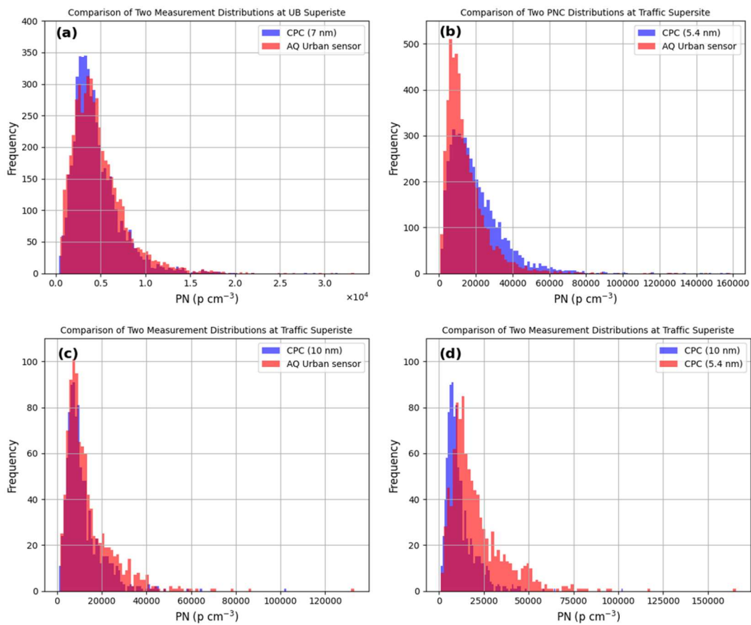
Figure S9. Comparison of measured PNC distributions between CPC and AQ Urban sensor at UB Supersite (a) and Traffic Supersite (b) and comparison of measured PNC distributions between CPC (10 nm) and AQ Urban sensor (c) and two CPCs (d) during the 6-week comparison period.
