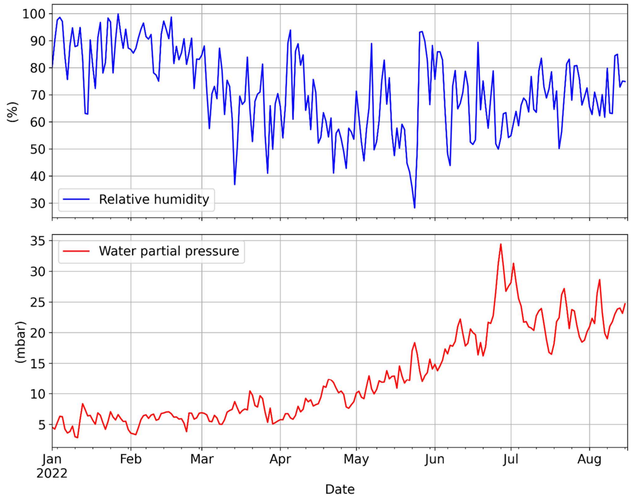
Figure S7. Daily averaged relative humidity and calculated water partial pressure during the measurement period. The relative humidity is measured at the Pasila weather station which is 1-2 km distance from the Traffic Supersite and UB Supersite
