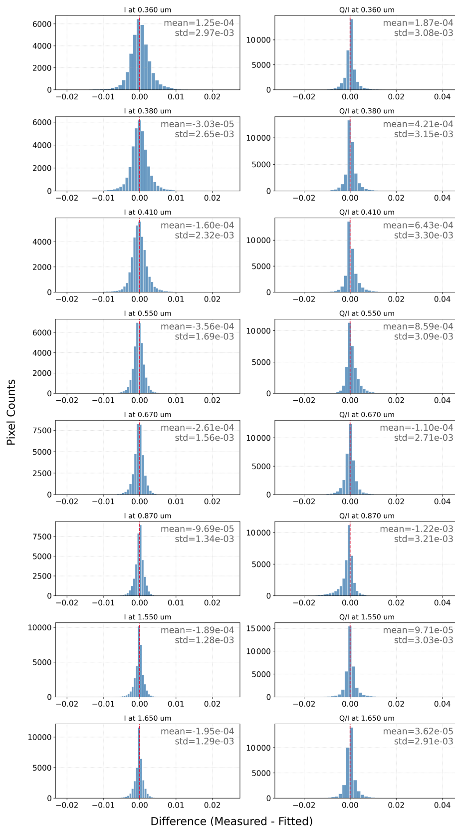
Figure 7. Histograms of Residuals (Measured – Fitted) for AOS polarimeter observations in 8 wavelengths across all scattering angles and pixels of the selected transect.
