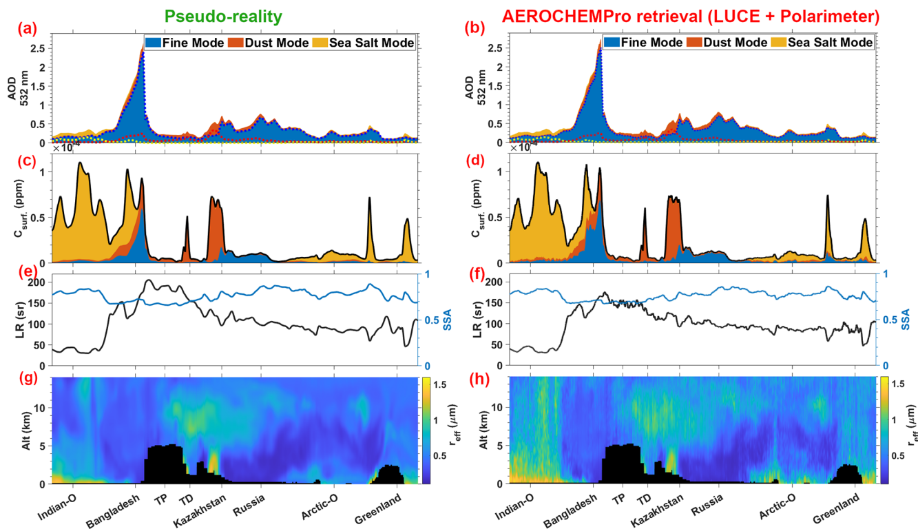
Figure 9. Comparison of (a, b) aerosol optical depth (AOD), (c, d) Surface mixing ratio ( C_{\text{surf}} ) in ppmV, (e, f) total-column SSA and LR at 532 nm and (g, h) total aerosol effective radius ( r_{\text{eff}} ) in \mu\text{m} , from top to bottom, respectively: Pseudo-reality left and retrievals right along the transect for fine mode, dust mode, and sea salt mode. For AOD and C_{\text{surf}} (a–d), stacked area plots represent the cumulative contribution of the fine, dust, and sea-salt modes. In the AOD plots (a, b), dashed lines indicate the absolute values for each mode: blue for fine mode, red for dust mode, and yellow for sea-salt mode. (The black shading area indicates the elevation.)
