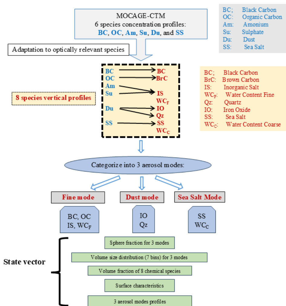
Figure 2. Steps to build the pseudo-reality.
