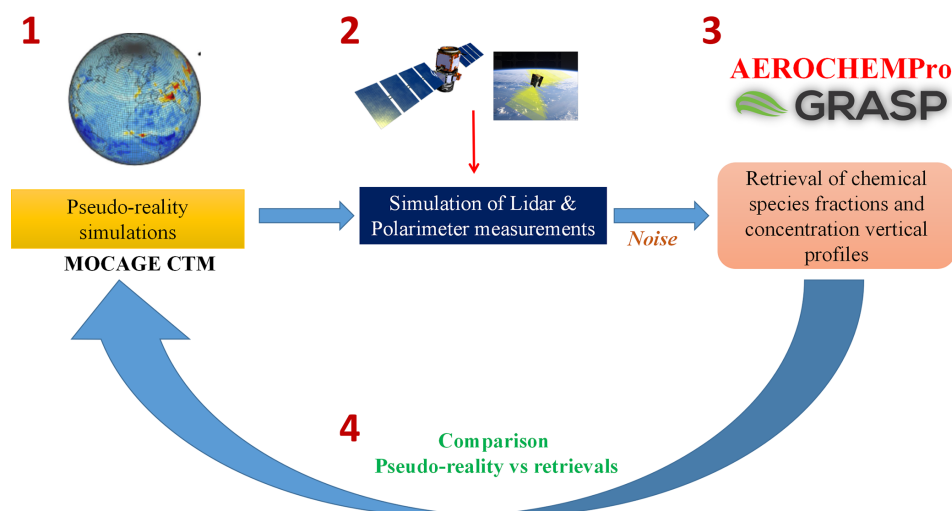
Figure 1. Scheme of the full observing system simulation experiment implemented for evaluating the performance of AEROCHEMPro.
