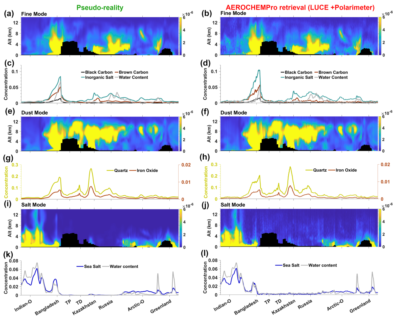
Figure 8. Comparison of vertical profiles for aerosol mode volume mixing ratio in ppmV (shaded) and total column volume concentrations in \text{um}^3 \text{um}^{-2} (line) along the transect: left – pseudo reality, right – retrieved. (The black shading area indicates the elevation.)
