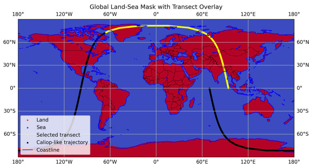
Figure 3. The selected transect extracted from MOCAGE data along the CALIOP-like trajectory and interpolated to match the spatial and temporal resolution of the observations on 15 May 2020 passing by the Indian Ocean, Bangladesh, Tibetan Plateau (TP), Taklamakan Desert (TD), Kazakhstan, Russia, Arctic Ocean, then reaching Greenland.
