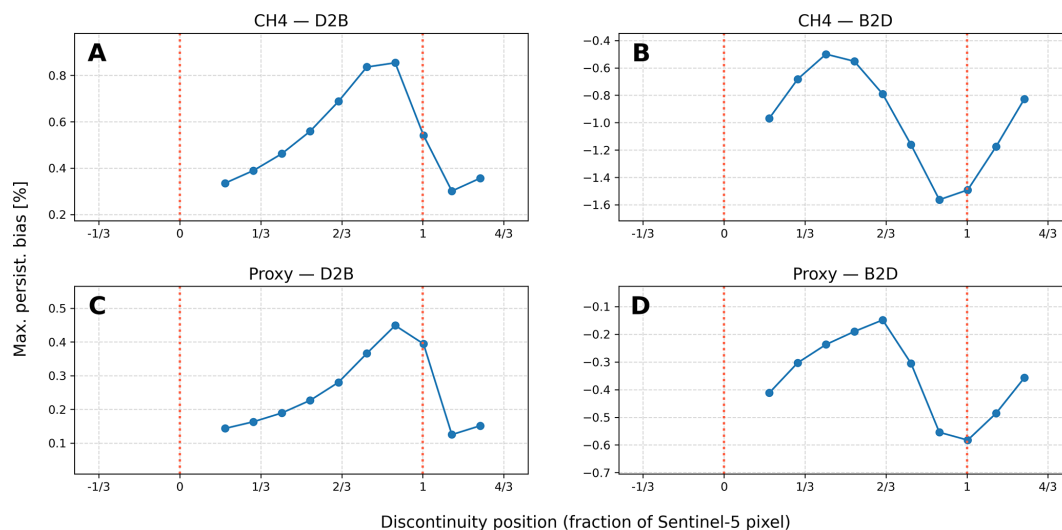
Figure B1. Panels (A) and (B) show the maximum persistence-induced CH 4 bias for the full-physics (scattering) retrieval as a function of the normalized position of the albedo discontinuity within the Sentinel-5 pixel, (0 = pixel start, 1 = pixel end). Panels (C) and (D) show the corresponding CH 4 /CO 2 bias for the proxy (non-scattering) retrieval. Panels (A) and (C) refer to the dark-to-bright (D2B) albedo scenes; and panels (B) and (D), to the bright-to-dark (B2D) albedo scenes. Two dotted red lines mark the Sentinel-5 pixel boundaries.
