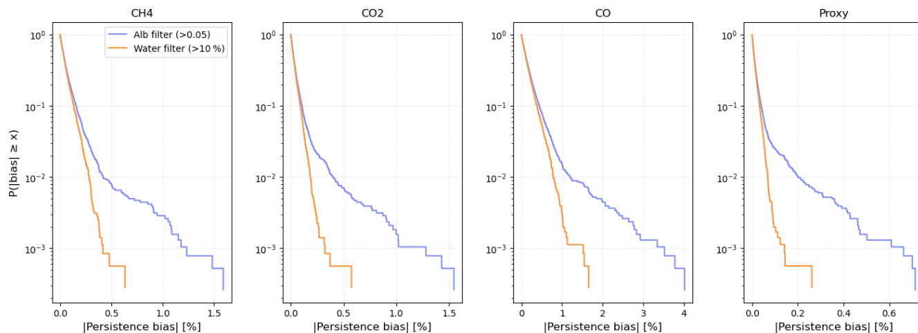
Figure 7. Each panel shows the complementary cumulative distribution function (CCDF) of the absolute persistence bias for CH 4 , CO 2 , CO, and for the CH 4 /CO 2 proxy ratio, combining data from the three Sentinel-2 scenes (the Nile Delta, California's Central Valley, and the Lusatian lignite district in Germany). Blue lines correspond to retrievals filtered with an albedo threshold of 0.05, consistent with the instrument sensitivity limit, while orange lines additionally include the water-land mask. The CCDFs represent the fraction of retrievals with an absolute bias exceeding a given threshold, allowing a direct comparison of the error-distribution tails for the two filter configurations.
