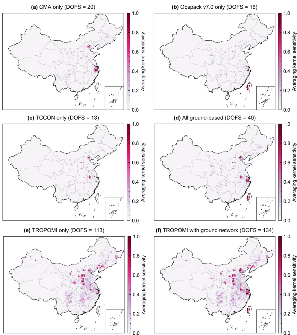
Figure 5. Spatial distributions of averaging kernel sensitivities in China using different observations in the Bayesian inversion. Panels (a)–(d) show observational constraints from (a) CMA (Fang et al., 2013; Wang et al., 2020; Zhang et al., 2022), (b) ObsPack 7.0 (Schuldt et al., 2024), (c) TCCON (Laughner et al., 2024; Liu et al., 2026; Morino et al., 2026; Shiomi et al., 2026; TCCON Team, 2022; Wunch et al., 2011; Zhou et al., 2026), and (d) all ground-based datasets combined. These observational constraints are only based on ground-based measurements and do not include any satellite observations. Panels (e) and (f) show observational constraints from (e) TROPOMI and (f) TROPOMI with all ground-based datasets combined. The DOFS value in each panel title indicates the national total DOFS in China contributed by the corresponding observational network. Surface station data © China Meteorological Administration (CMA). ObsPack data © NOAA. TCCON data © TCCON Team and contributing institutions. TROPOMI data © ESA/Copernicus.
