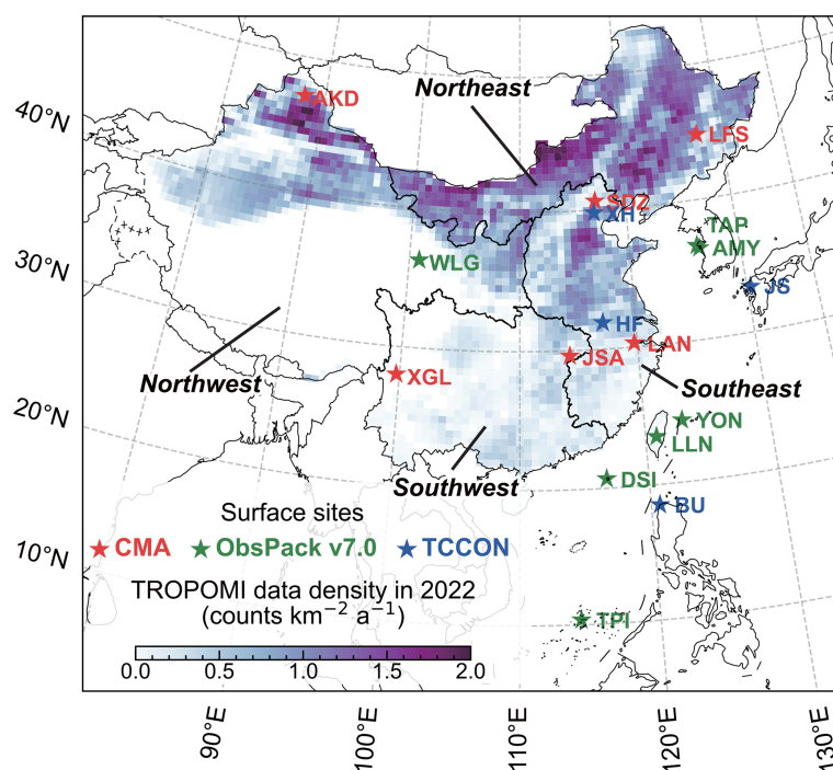
Figure 1. Spatial distribution of TROPOMI methane observation density ( \text{counts km}^{-2} \text{a}^{-1} ) and ground-based monitoring stations for the year 2022. The surface stations are sourced from networks and databases including the China Meteorological Administration (CMA) (Fang et al., 2013; Wang et al., 2020; Zhang et al., 2022), NOAA GLOBALVIEWplus \text{CH}_4 ObsPack v7.0 (Schuldt et al., 2024) and the Total Carbon Column Observing Network (Laughner et al., 2024; Liu et al., 2026; Morino et al., 2026; Shiomi et al., 2026; TCCON Team, 2022; Wunch et al., 2011; Zhou et al., 2026). The TROPOMI observation density is shown at 0.5^\circ \times 0.625^\circ horizontal resolution. Additional details regarding the surface site characteristics and TROPOMI observation information are provided in Table 1. The four regions (Northeast, Northwest, Southeast and Southwest) are spatially defined in Fig. 1. TROPOMI data © ESA/Copernicus. GLOBALVIEWplus \text{CH}_4 ObsPack data © NOAA. TCCON data © TCCON Team and contributing institutions. Surface station data © China Meteorological Administration (CMA).
