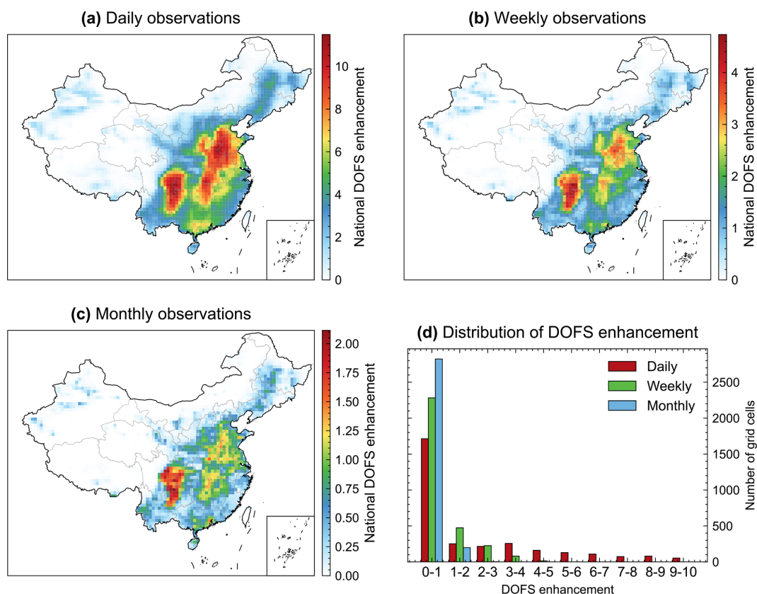
Figure 6. The degrees of freedom for signal (DOFS) enhancement in China by adding one ground station with different temporal frequencies. National total DOFS enhancement from adding one ground station per grid cell on the basis of the existing observational network assuming different sampling frequency: (a) Daily, (b) Weekly, and (c) Monthly. (d) Distribution of DOFS enhancement per grid cell for different sampling frequencies. The x axis represents the DOFS enhancement in each grid cell, divided into 10 evenly spaced bins from 0 to 10. The y axis represents the number of grid cells falling into each bin.
