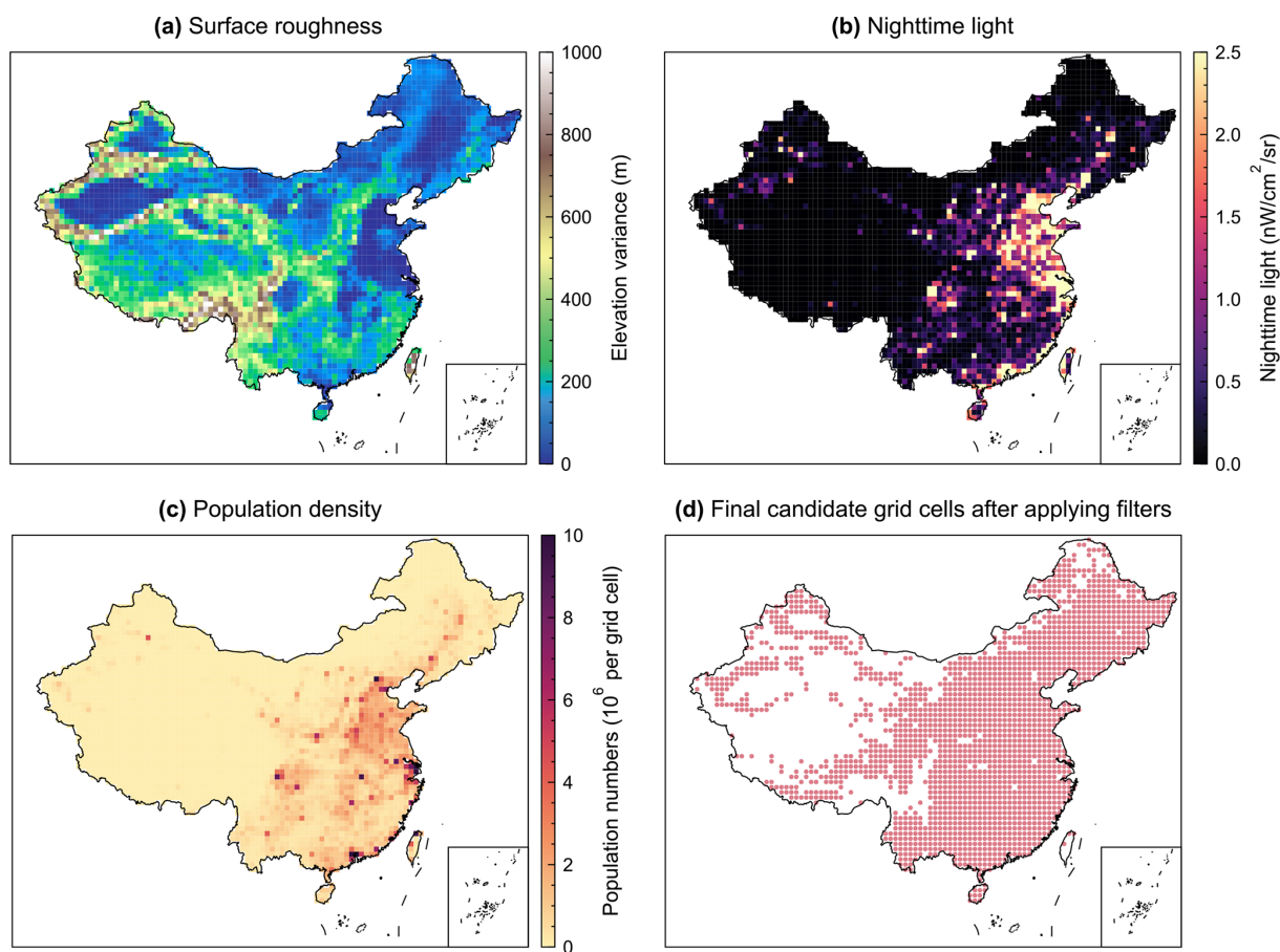
Figure 3. Grid cells suitable for new stations. Panels (a)–(c) illustrate the criteria that determine grid cells suitable for new stations. The following criteria are applied (excluding those containing existing stations): (a) Surface roughness, derived from DEM data (Geospatial Information Authority of Japan, 2025), calculated as the standard deviation of elevation across 30 arcsec pixels within each 0.5^\circ \times 0.625^\circ grid cell. (b) Nighttime light intensity from (Elvidge et al., 2013), averaged over 0.5^\circ \times 0.625^\circ grids. (c) Population density (Center for International Earth Science Information Network (CIESIN) – Columbia University, 2017). Panel (d) shows the final candidate grid cells after applying all selection filters, where grid cells are excluded if their surface roughness exceeds the 90th percentile, or if either population density or nighttime light intensity falls below the 20th percentile. These filtered grid cells are subsequently used in simulated annealing to identify the optimal locations for new stations. DEM data © Geospatial Information Authority of Japan (GSI). Nighttime lights data © NOAA. Population data © CIESIN, Columbia University.
