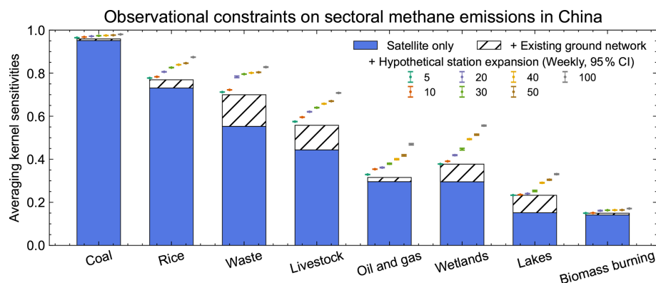
Figure 10. Observational constraint on sectoral methane emissions in China under different observational networks. The blue bars represent AK sensitivities derived from TROPOMI observations alone, while the hatched bars represent the increase in AK sensitivities achieved by incorporating existing ground-based measurements. Colored data points show the mean AK sensitivities after adding new ground stations (weekly sampling frequency), with error bars denoting 95 % confidence intervals from the 50 simulated annealing experiments.
