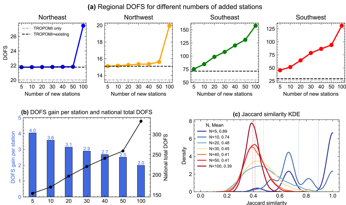
Figure 8. Performance of the simulated annealing algorithm under weekly sampling for different network sizes (5–100 stations) across 50 independent realizations. (a) Regional DOFS in China. Results are shown for four sub-regions (Northeast, Northwest, Southeast, Southwest; see Fig. 1 for regional definitions). (b) Average DOFS enhancement per each newly added station in China, calculated as the DOFS enhancement divided by the number of new sites. (c) Kernel density estimation of pairwise Jaccard similarity across 50 independent simulated annealing realizations. Solid colored curves show the probability density distributions. Vertical dotted lines indicate the mean similarity for each network size (mean values shown in legend).
