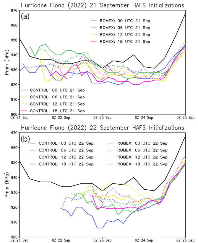
Figure 11. Hurricane Fiona (2022) P_{\text{MIN}} forecasts initialized on (a) 21 September and (b) 22 September, shown for Control (solid lines) and ROMEX (dotted lines). Lines plotting forecast P_{\text{MIN}} time series are colored by initialization time, as indicated in the inset key boxes. The black line shows the NHC Best Track P_{\text{MIN}} for Fiona.
