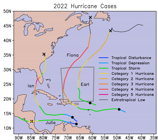
Figure 1. The observed tracks of the four 2022 Atlantic hurricanes selected for the ROMEX HAFS-A forecast experiments, with colors indicating the stage of TC development at the time. V_{MAX} stratifies hurricane intensity according to the Saffir–Simpson Scale: Category 1 (64–82 kn), Category 2 (83–95 kn), Category 3 (96–112 kn), Category 4 (113–136 kn), and Category 5 (above 136 kn). Closed circles and X-symbols mark the beginning and end, respectively, of each hurricane’s HAFS-A experiment cycling period. The dark gray polygon shows the HAFS-A moving nest boundaries for the 06:00 UTC 7 September Hurricane Earl analysis.
