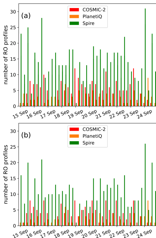
Figure 2. (a) Number of COSMIC-2, PlanetiQ, and Spire GNSS RO profiles available for assimilation in the HAFS-A moving nest for individual Hurricane Fiona (2022) DA cycles, shown as red, orange, and green bars, respectively. Each 00:00 UTC cycle time is labeled with its date on the x -axis. (b) As in panel (a), except showing the number of profiles with at least one bending angle assimilated below 800 hPa.
