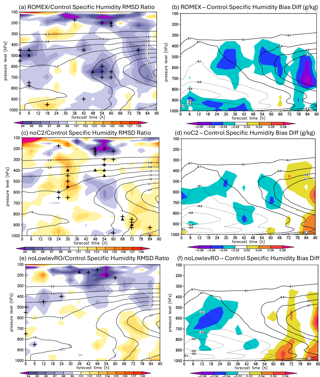
Figure 9. As in Fig. 8, but for the HAFS-A specific humidity RMSD ( \text{g kg}^{-1} ).
