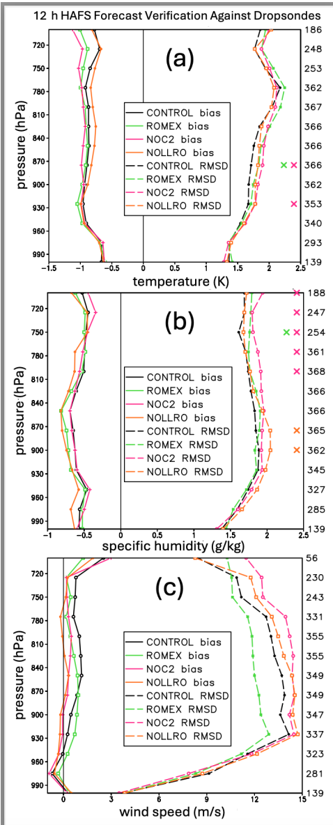
Figure 10. (a) Solid lines show profiles of the 12 h HAFS-A temperature forecast bias (K) computed against NOAA aircraft reconnaissance mission dropsondes for Control (black), ROMEX (green), Control_noC2 (magenta), and ROMEX_noLowlevRO (orange). The number of dropsonde temperature observations per verification layer is shown on the right y-axis. Dashed lines show the 12 h HAFS-A forecast temperature RMSD (K) relative to dropsonde data, colored by experiment. (b) As in panel (a) but for 12 h forecast specific humidity ( \text{g kg}^{-1} ). (c) As in panel (a) but for 12 h forecast horizontal wind speed ( \text{m s}^{-1} ). Green, magenta, and orange X-symbols, respectively, mark layers where the ROMEX, Control_noC2, and ROMEX_noLowlevRO forecast RMSDs differ statistically significantly from the Control RMSD at the 95 % level.
