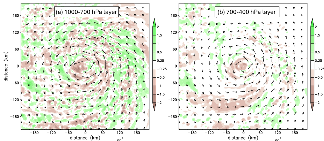
Figure 12. (a) ROMEX-minus-Control specific humidity differences ( \text{g kg}^{-1} ) averaged over the 1000–700 layer and over the 00:00, 06:00, 12:00, and 18:00 UTC 21 September analyses. Vectors show ROMEX 900 hPa horizontal winds ( \text{m s}^{-1} ) averaged over the same four analyses. (b) As in panel (a) but for ROMEX-minus-Control specific humidity differences averaged over the 700–400 hPa layer with 500 hPa ROMEX horizontal winds.
