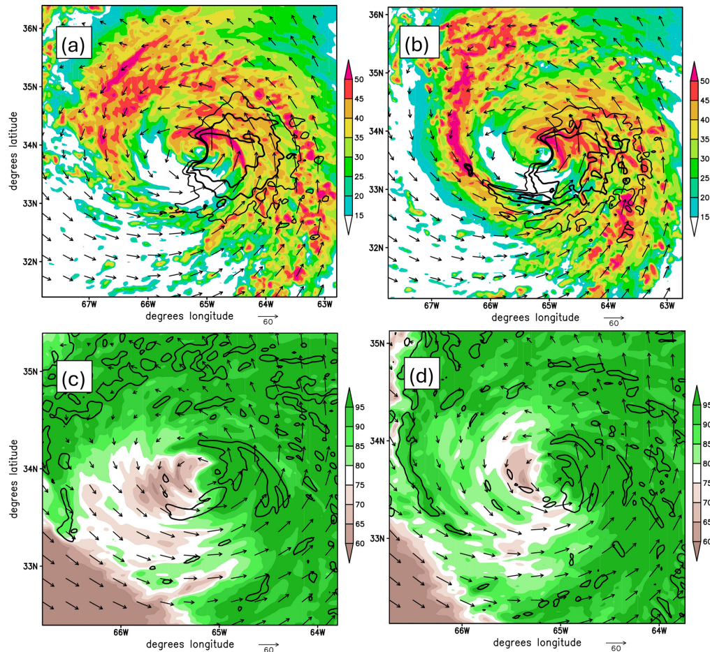
Figure 14. As in Fig. 13, but for 48 h forecasts valid at 12:00 UTC 23 September.
