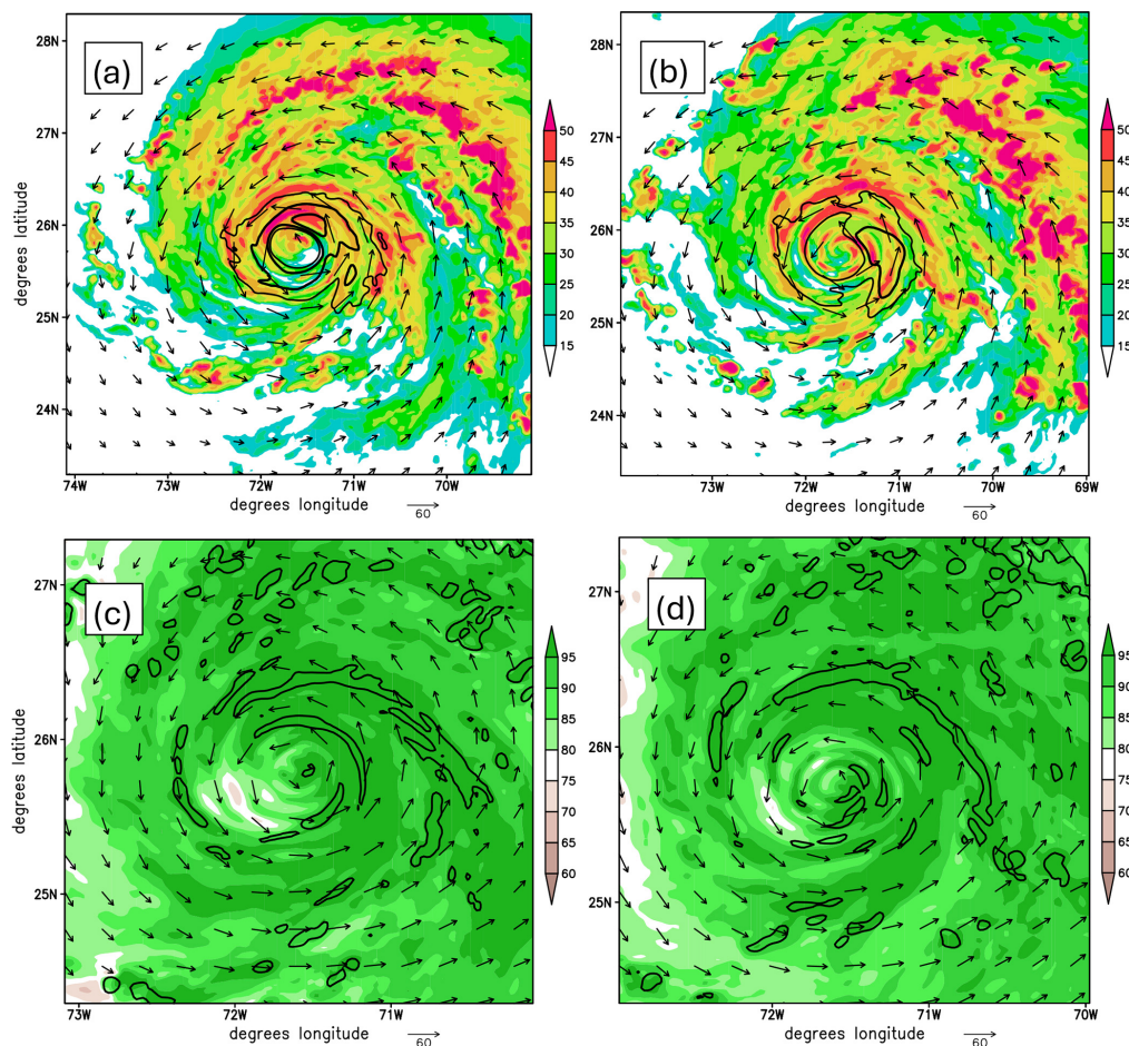
Figure 13. (a) Control 12 h forecast of Hurricane Fiona (2022) composite radar reflectivity (shading, dBZ) valid at 00:00 UTC 22 September. Horizontal winds at 900 hPa ( \text{m s}^{-1} ) are shown as vectors (see arrow scale at lower right) and their magnitudes are contoured (thin for 50 and thick for 55 and 60). (b) As in panel (a) but for the ROMEX experiment. (c) Same Control 12 h forecast shown in panel (a), but here plotting 700–400 hPa layer-averaged RH (shading, %), the 1 \text{ m s}^{-1} vertical velocity contour at 600 hPa, and 500 hPa horizontal wind vectors ( \text{m s}^{-1} ). (d) As in panel (c) but for the ROMEX experiment.
