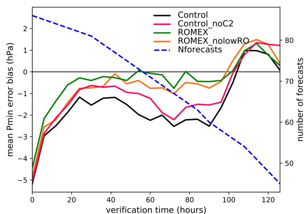
Figure 7. Forecast time series of TC P_{\text{MIN}} mean bias (hPa) for the Control (black line), Control_noC2 (magenta line), ROMEX (green line), and ROMEX_nolowRO (orange line) experiments, along with the number of forecasts used for verification (dashed blue line).
