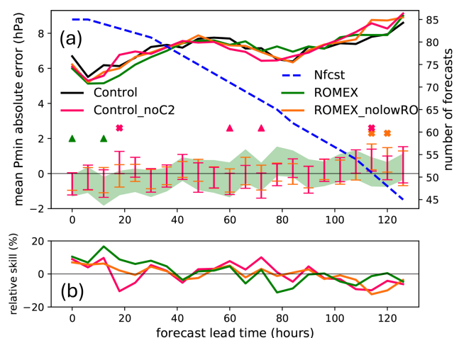
Figure 6. As in Fig. 5, but for TC P_{\text{MIN}} intensity (hPa).
