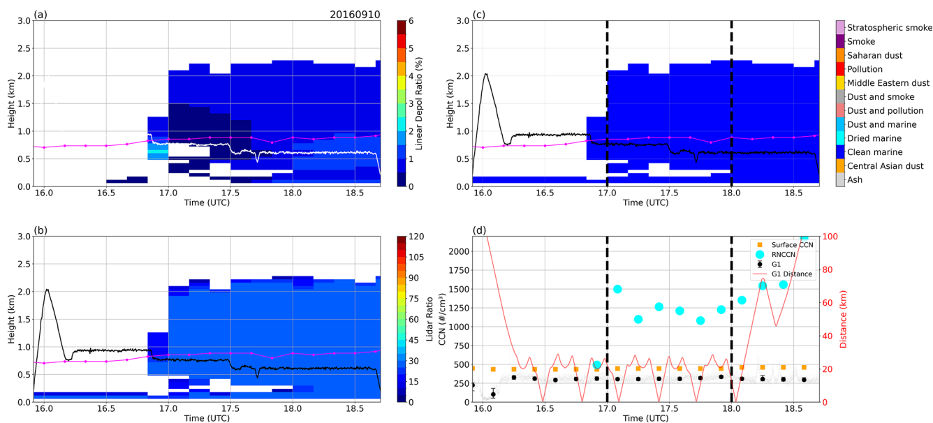
Figure D1. Same as Fig. 3, but for the case of 10 September 2016.
