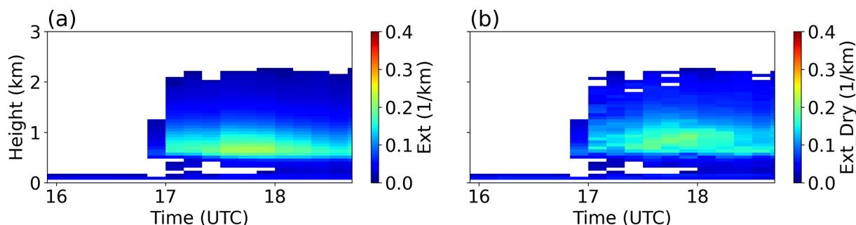
Figure D2. Time–height cross sections of Raman-lidar aerosol extinction for the case on 10 September 2016. (a) Lidar extinction coefficient (Ext, km −1 ). (b) Dry-corrected aerosol extinction coefficient (Ext Dry , km −1 ) directly used in the RNCCN.
