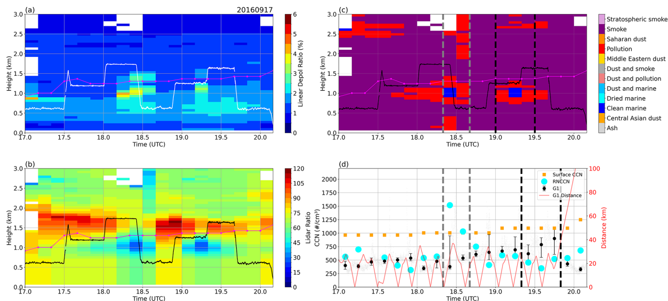
Figure 4. Same as Fig. 3, but for the case of 17 September 2016 (case #2).
