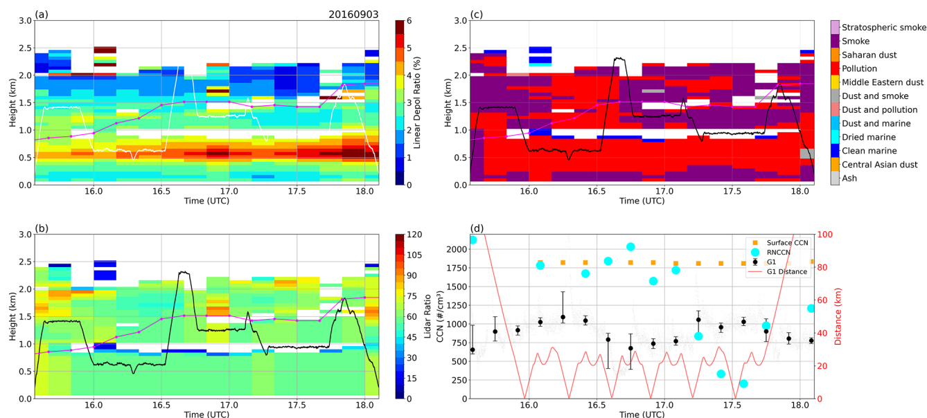
Figure 5. Same as Fig. 3, but for the case of 3 September 2016 (case #3).
