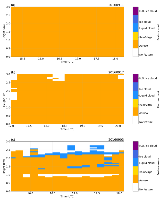
Figure C1. Feature mask from Raman Lidar on (a) 11 September 2016 (case #1), (b) 17 September 2016 (case #2), and (c) 3 September 2016 (case #3).
