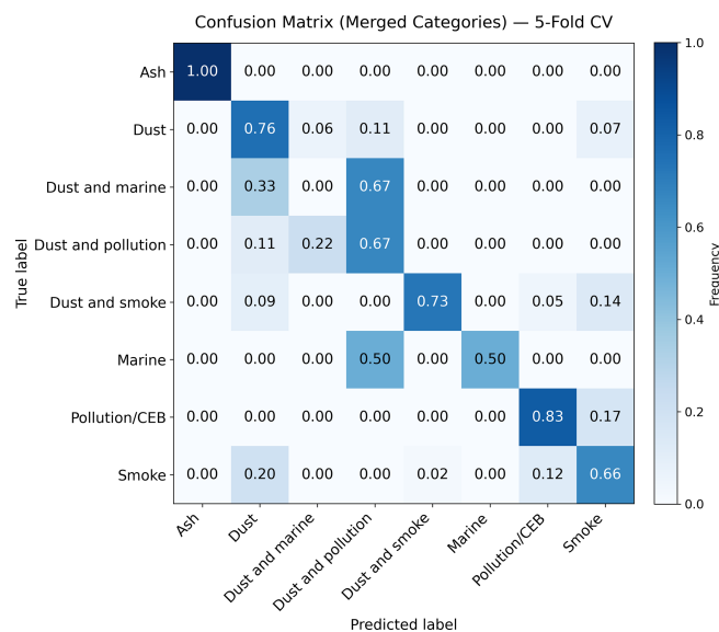
Figure 2. Row-normalized confusion matrix for the kNN aerosol-type classifier using merged DeLiAn categories, based on 5-fold stratified cross-validation. Rows denote the true class, and columns denote the predicted class; diagonal elements give the per-class recall (classification accuracy), and off-diagonal elements show the fraction misclassified into other classes. The corresponding confusion matrix for the original (unmerged) DeLiAn classes is shown in Appendix Fig. B1.
