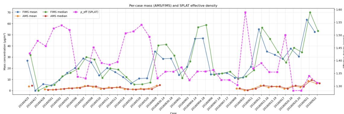
Figure A1. Per-case aerosol mass derived from the Fast Integrated Mobility Spectrometer (FIMS) and the Aerosol Mass Spectrometer (AMS), together with Single Particle Laser Ablation Time-of-Flight Mass Spectrometer (SPLAT)–derived effective particle density ( \rho_{\text{eff}} ). FIMS aerosol mass (mean and median) is estimated from measured aerosol size distributions using the case-specific effective density ( \rho_{\text{eff}} ), while AMS mass represents non-refractory submicron aerosol species, including sulfate ( \text{SO}_4^{2-} ), nitrate ( \text{NO}_3^- ), ammonium ( \text{NH}_4^+ ), chloride ( \text{Cl}^- ), and organic aerosol (Org).
