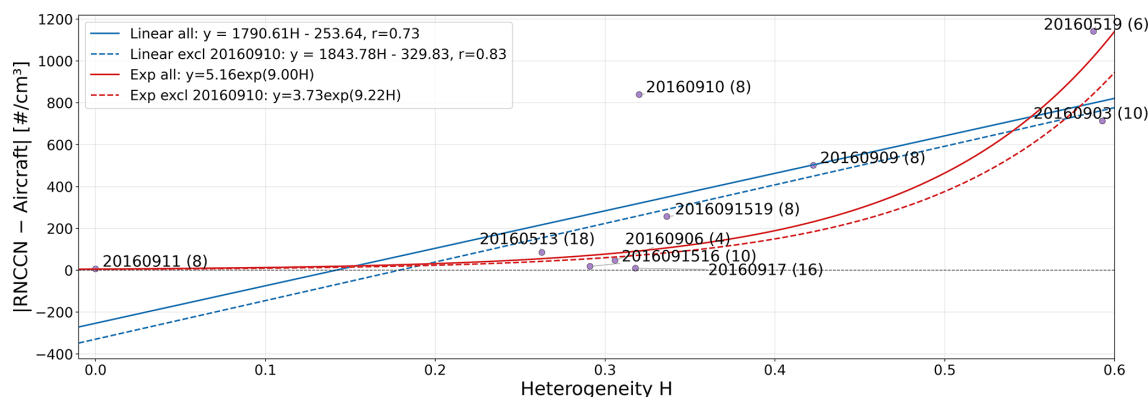
Figure 6. Case-level relationship between aerosol heterogeneity H and RNCCN Aircraft difference [\text{RNCCN} - \text{Aircraft}] . Cases are labeled by date (YYYYMMDD); when more than one qualifying flight segment occurred on the same day, the central UTC hour is appended (YYYYMMDDHH; e.g., 2016091516 and 2016091519). Solid lines represent linear and exponential fits using all cases, while dashed lines exclude the 20160910-outlier case.
