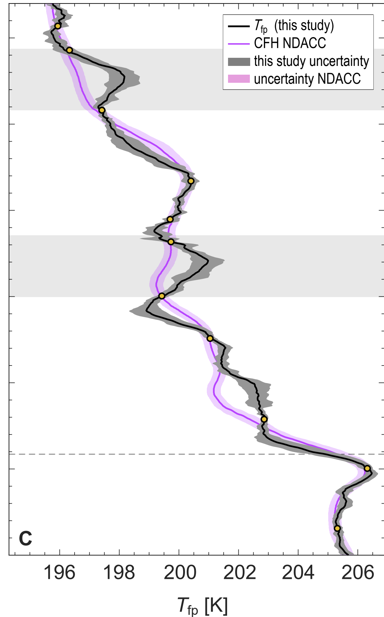
Uncertainty range of nonequilibrium-corrected T_{fp}
