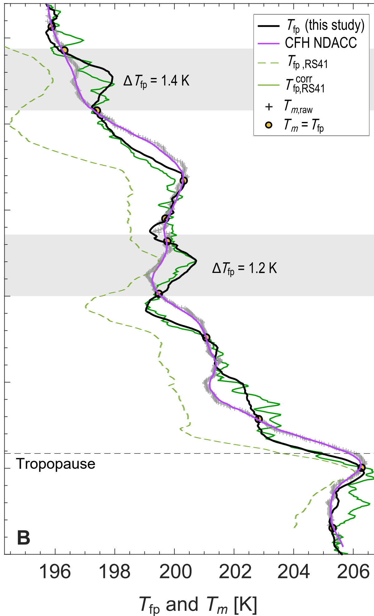
Frost point and mirror temperatures
