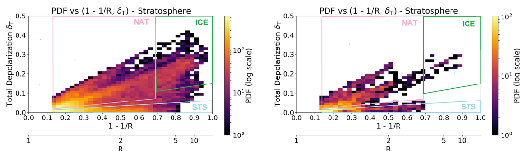
Figure 1. Point-density probability distribution of PSC measurements in the (1 - 1/R) , \delta_T optical phase space. Left: full dataset including all Young-inverted cloud layers. Right: Young-optimized subset (Sect. 3.4). The full dataset cleanly separates STS, NAT and ice PSC clusters, while the Young-optimized subset suppresses most ice PSC occurrences. Regions identified as STS, NAT and ice PSCs are indicated by areas bounded by light-blue, pink and green contours, respectively.
