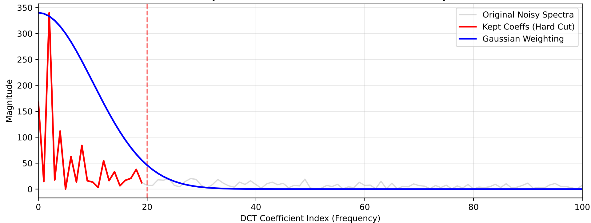
(b) DCT Spectral Domain: Hard Cut vs. Gaussian Taper
