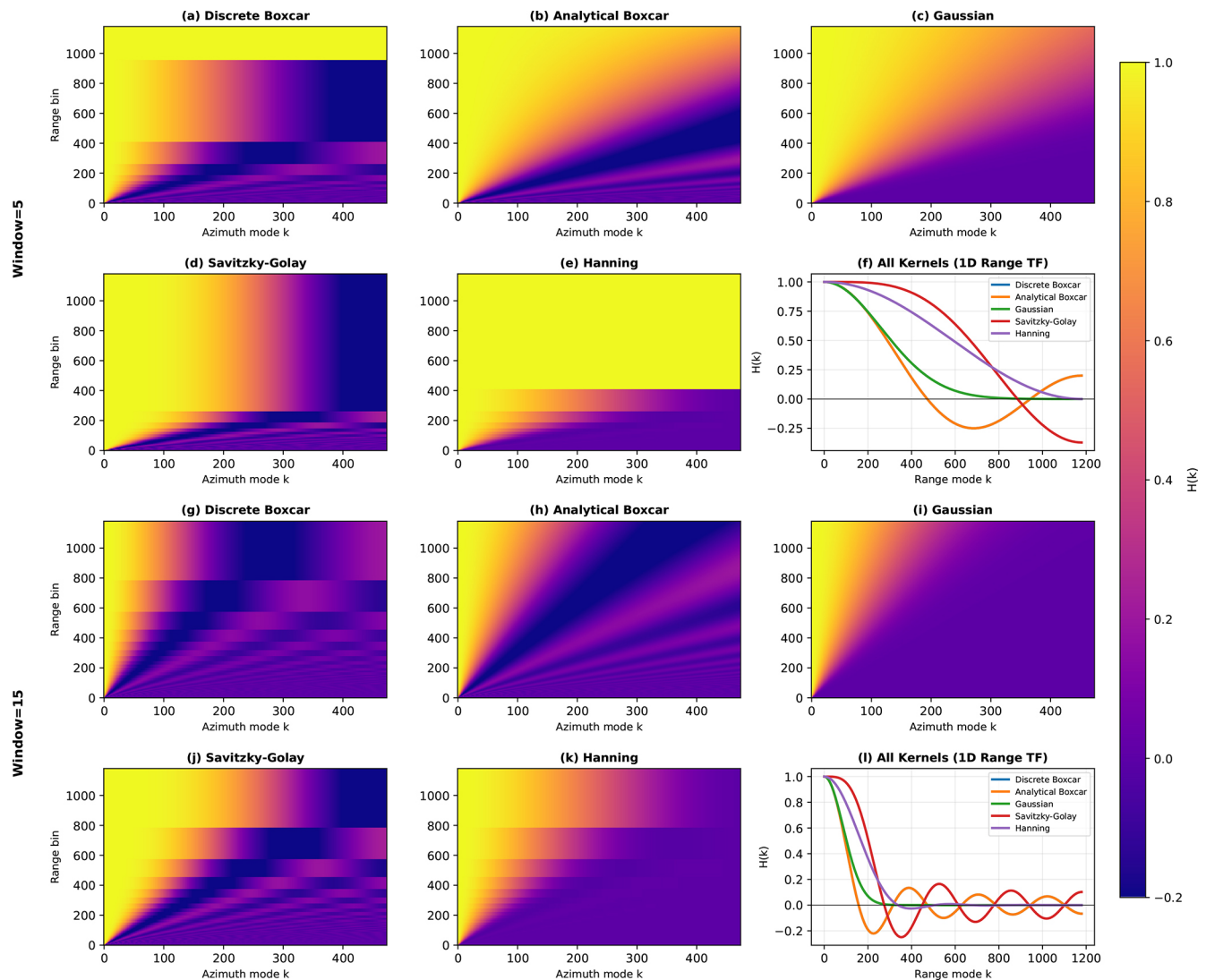
Figure 3. Spectral response of different kernels for two window sizes. Window 5: (a–e) 2D angle transfer functions, and (f) Range transfer function. Window 15: (g–k) Angle transfer functions, and (l) Range transfer function.
