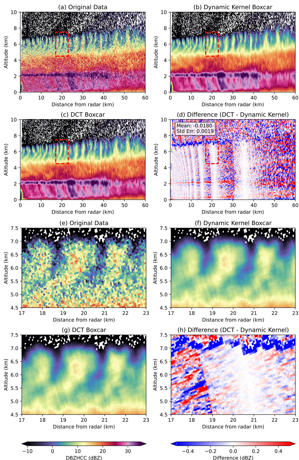
Figure 4. Application to C-band radar observations on 23 February 2022 at 02:28 UTC. (a) Original observational field with noise and gaps. (b) Result of spatial dynamic kernel smoothing (window 5 pixels). (c) Result of DCT-based smoothing (analytical continuous boxcar, window 5 pixels). (d) Difference between spatial and spectral methods. The red dashed box indicates the zoom region shown in panels (e)–(h).
