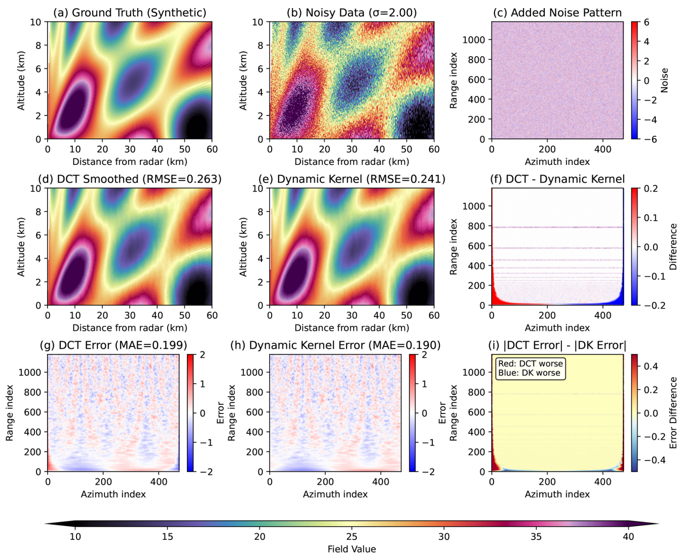
Figure 2. Comparison of synthetic ground truth, noisy observation, and smoothing performance. (a) Ground-truth synthetic Range-Height Indicator (RHI) radar image in polar coordinates. The field value mimics reflectivity ( Z_e ), but could be any dual-polarization variable. (b) Noisy observation ( \sigma = 2.00 ). (c) The added noise pattern. (d) DCT-based smoothed result. (e) Spatial Dynamic Kernel (DK) smoothed result. (f) Difference between DCT and DK results. (g) DCT error map. (h) DK error map. (i) Difference of absolute errors ( |\text{Error}_{\text{DCT}}| - |\text{Error}_{\text{DK}}| ), where positive values indicate the DCT method performed worse and negative values indicate the DK method performed worse. Performance metrics include Root Mean Square Error (RMSE) and Mean Absolute Error (MAE).
