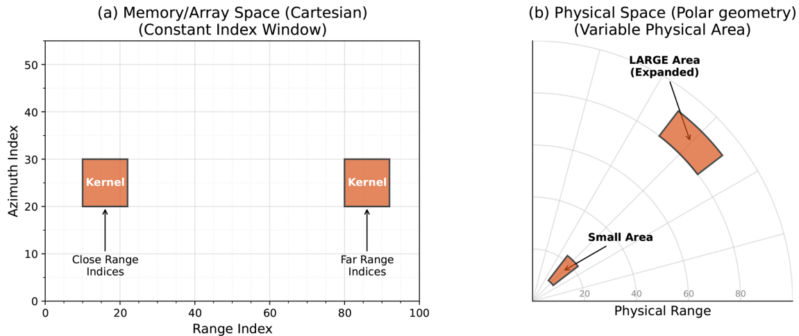
Figure 1. Conceptual comparison of coordinate distortion for (a) a window of constant size in grid space (range-angle indices) that corresponds to (b) physically different areas in a physical space depending on the range. At close range, the physical area is small, whereas at far range, it expands significantly. This distortion necessitates dynamic kernel sizing to maintain a constant physical smoothing scale.
