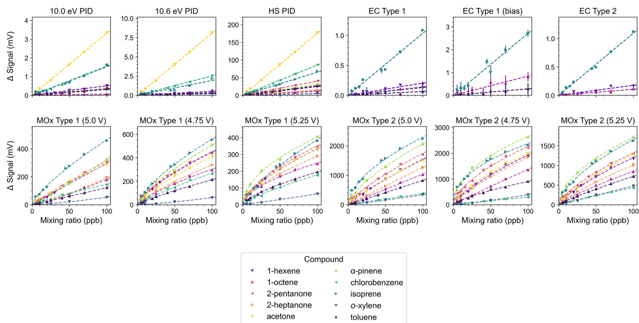
Figure 3. Summary of sensor responses (in mV over baseline) to various VOC mixing ratios between 5–100 ppb at 30 % RH. Dotted lines represent the linear least-squares regression (PID and EC) or the power-law fit (MOx) of the measured values, denoted by triangles. Note that y-axes are not shared across panels, reflecting the wide range of sensitivities across sensors. If a compound is missing from a sensor's subplot, as is the case with EC sensors, it means that the sensor does not exhibit sensitivity to that compound above its baseline noise. Error bars denote the standard deviation of measurements taken for each data point.
