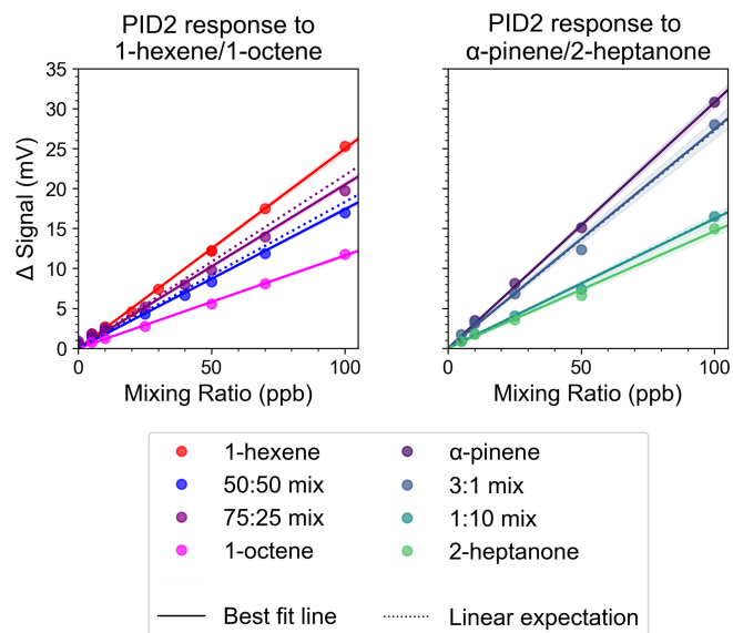
Figure 7. Left panel: high-sensitivity PID (PID2) responses to 1 : 1 (blue) and 3 : 1 (dark purple) mixtures of 1-hexene (red) and 1-octene (magenta). Right panel: PID2 responses to 3 : 1 (blue) and 1 : 10 (teal) mixtures of \alpha -pinene (indigo) and 2-heptanone (aquamarine). Solid lines indicate the best fit line for each of the points, and the shaded area indicates the 1\sigma confidence interval; dotted lines indicate the expected signal assuming additivity. The mixing ratio ( x axis) refers to the total amount of VOC (i.e., both components of the mixtures) introduced to the sensors.
