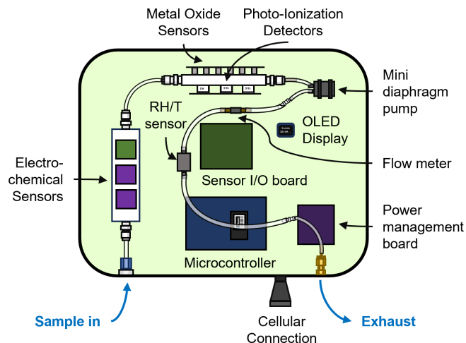
Figure 1. Schematic of the VOC air sensor array. Sample air is pulled in by a miniature diaphragm pump through custom flow cells that house 12 different VOC sensors. Several custom circuit boards manage power and sensor inputs/outputs.
