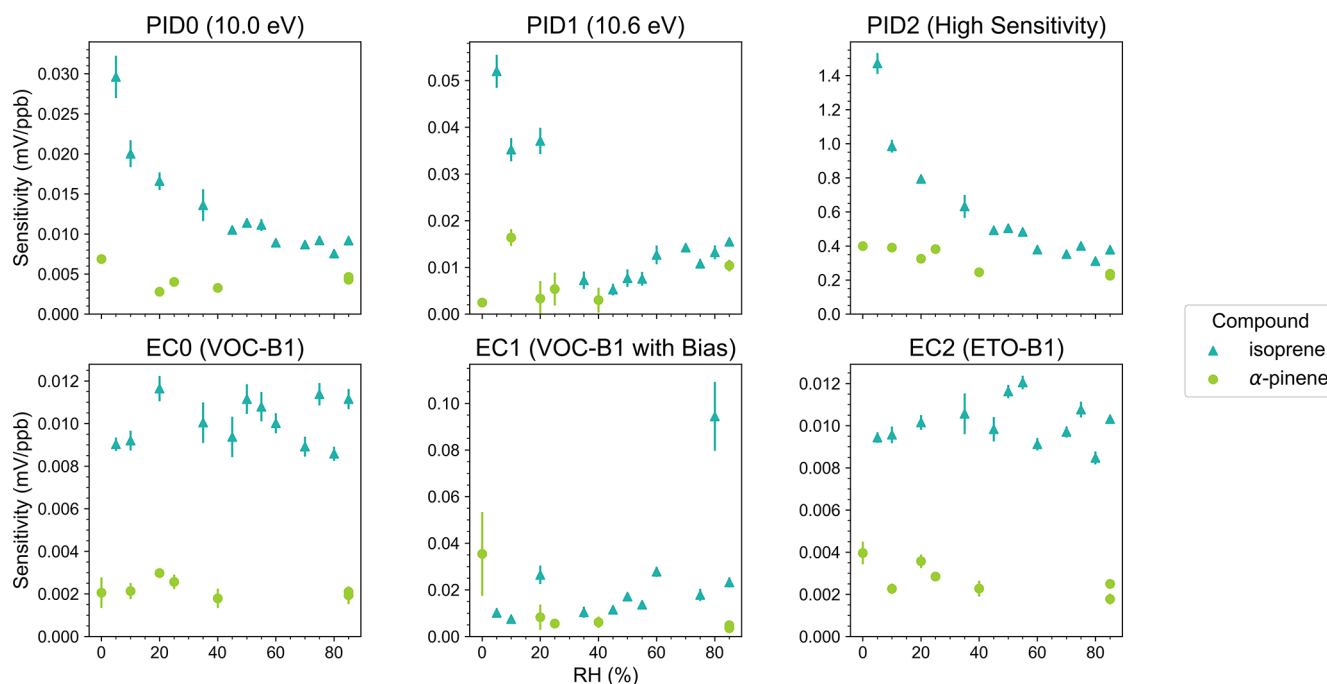
Figure 5. Sensitivities (in \text{mV ppb}^{-1} ) of 3 PIDs (top row) and 3 EC sensors (bottom row) to isoprene and \alpha -pinene as a function of RH. Vertical bars denote 1\sigma confidence intervals. Note that each panel features a different y-axis.
