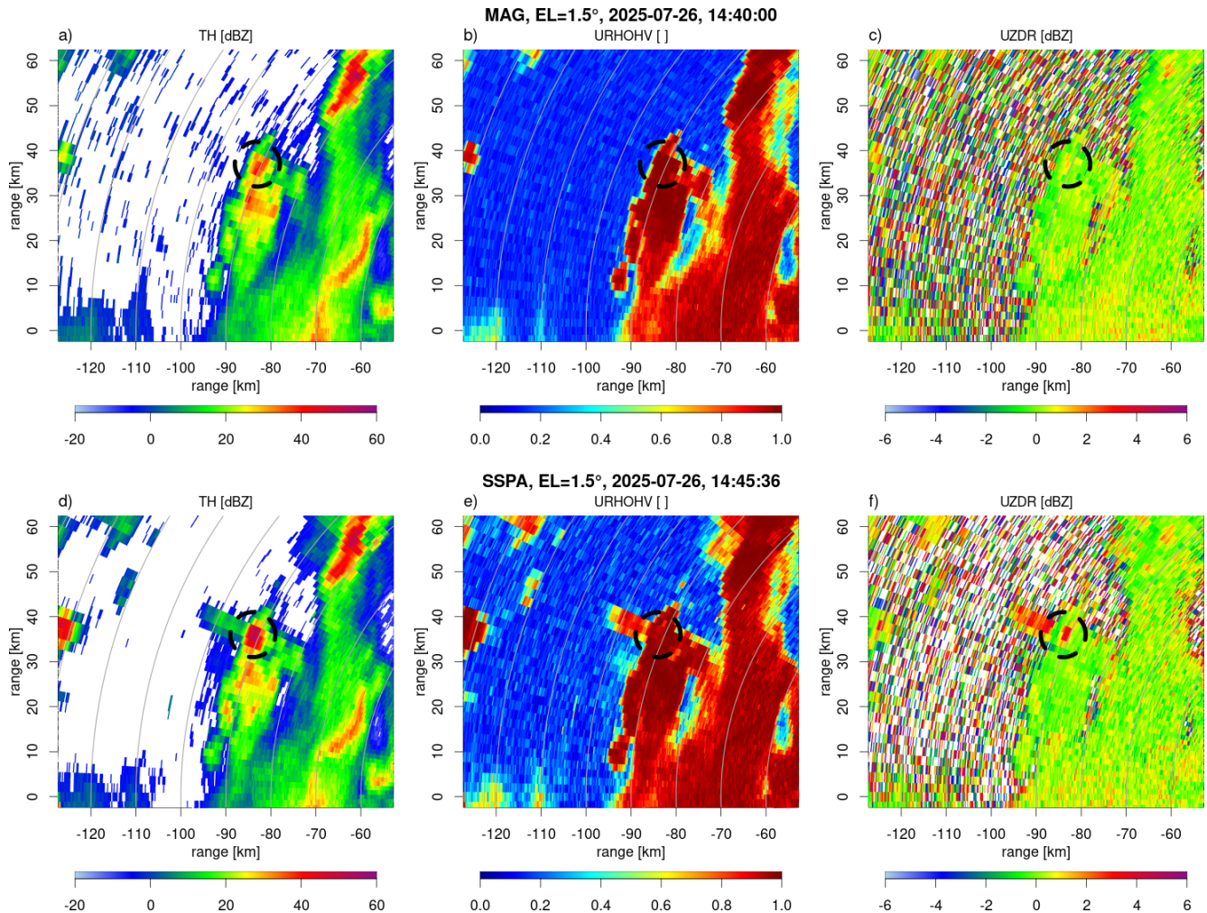
Figure 19. Example of range sidelobes around a convective core, recorded on 26 July 2025. Shown are TH, URHOHV and UZDR for MAG in panels (a)–(c) and for SSPA in panels (d)–(f). The black dashed circle shows the precise location of the convective core. Small differences between the two transmitters are caused by the five minute time difference in which the strength of the convective core increased.
