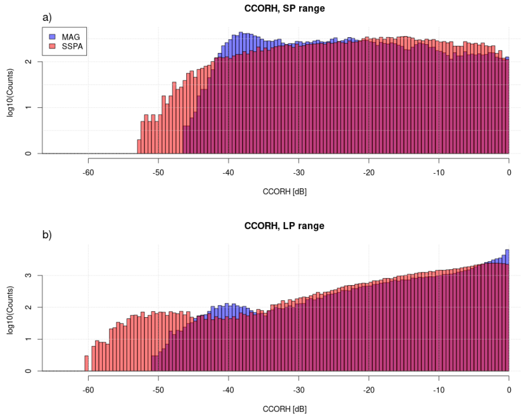
Figure 20. Distribution of CCORH values in two sweeps of SSPA in red and MAG in blue. Data recorded during clear sky conditions on 20 April 2025. (a) Short pulse range or inner 16 km, (b) long pulse range. Counts are displayed in a logarithmic scale.
