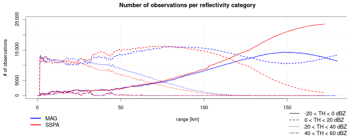
Figure 7. Amount of valid data points per reflectivity category and transmitter during the 2024 stratiform event. These values are valid for Figs. 6, 10, 13, 14 and 16.
