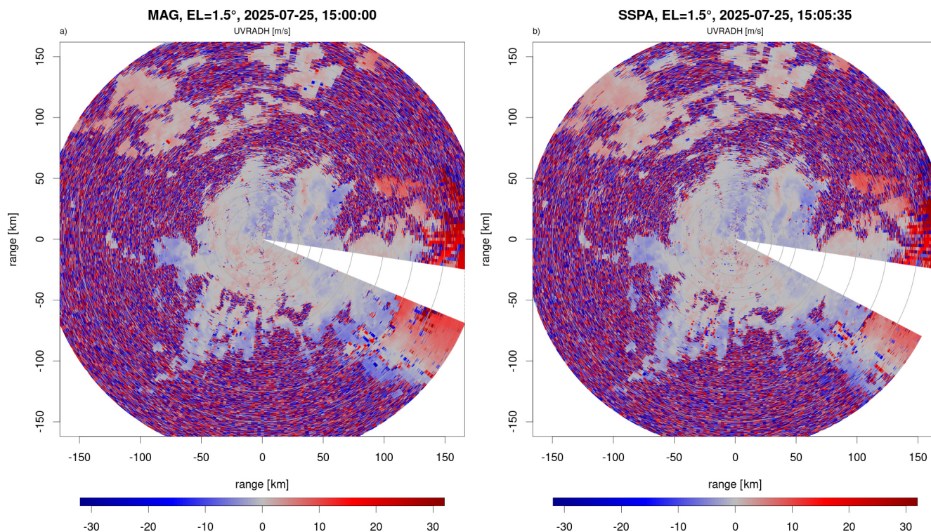
Figure 9. PPI images of the uncorrected and unfolded radial velocity (UVRADH) from a scan in 1.5^\circ elevation from (a) MAG and (b) SSPA. Data were recorded during a convective event in July 2025. No thresholding was applied. See also Fig. 3.
