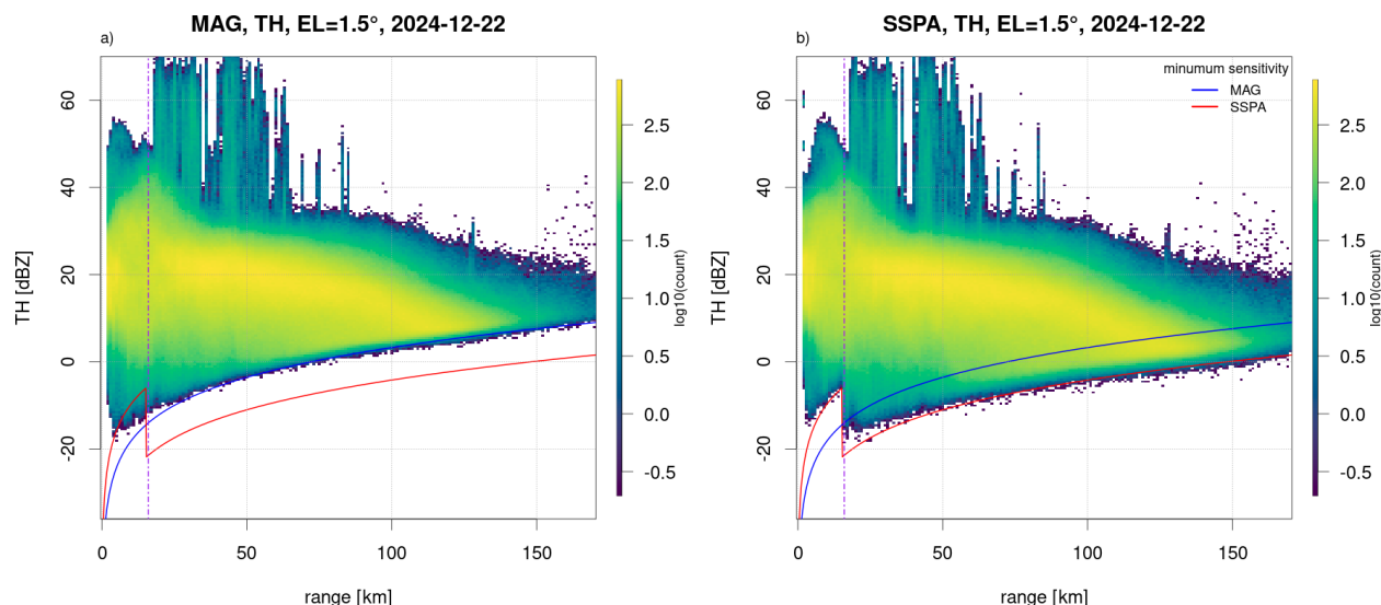
Figure 5. Frequency of reflectivity values in dependence on range, from 1.5° elevation and (a) MAG and (b) SSPA. Data thresholded with \text{RhoHV} < 0.6 and aggregated over 13 h (72 sweeps per transmitter). Blue and red lines show the calculated minimum sensitivity for MAG and SSPA respectively. The vertical purple dashed line marks the short pulse/long pulse border. Logarithmic histogram counts are shown as colors.
