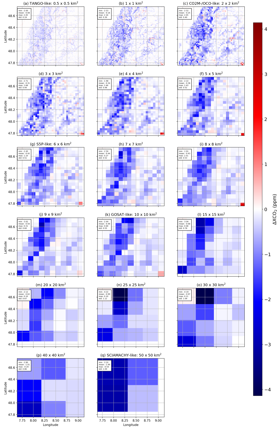
Figure S6. \Delta XCO_2 with variable size of the spatial samples as in the left column of Fig. 21 of the main text, but for more spatial sample sizes.
