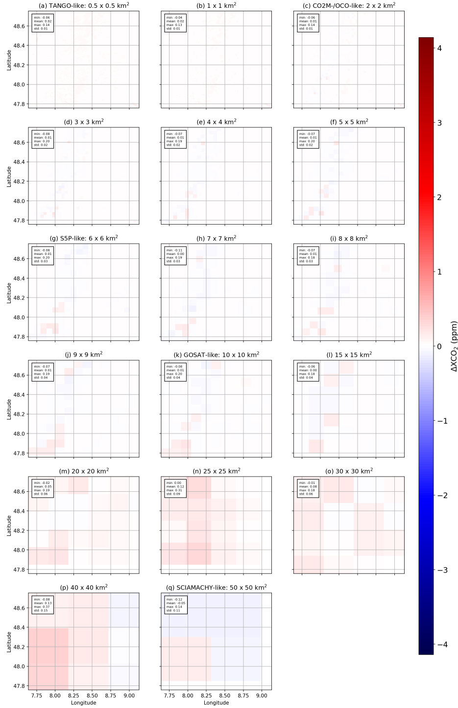
Figure S7. \Delta XCO_2 with variable size of the spatial samples as in the center column of Fig. 21 of the main text, but for more spatial sample sizes.
