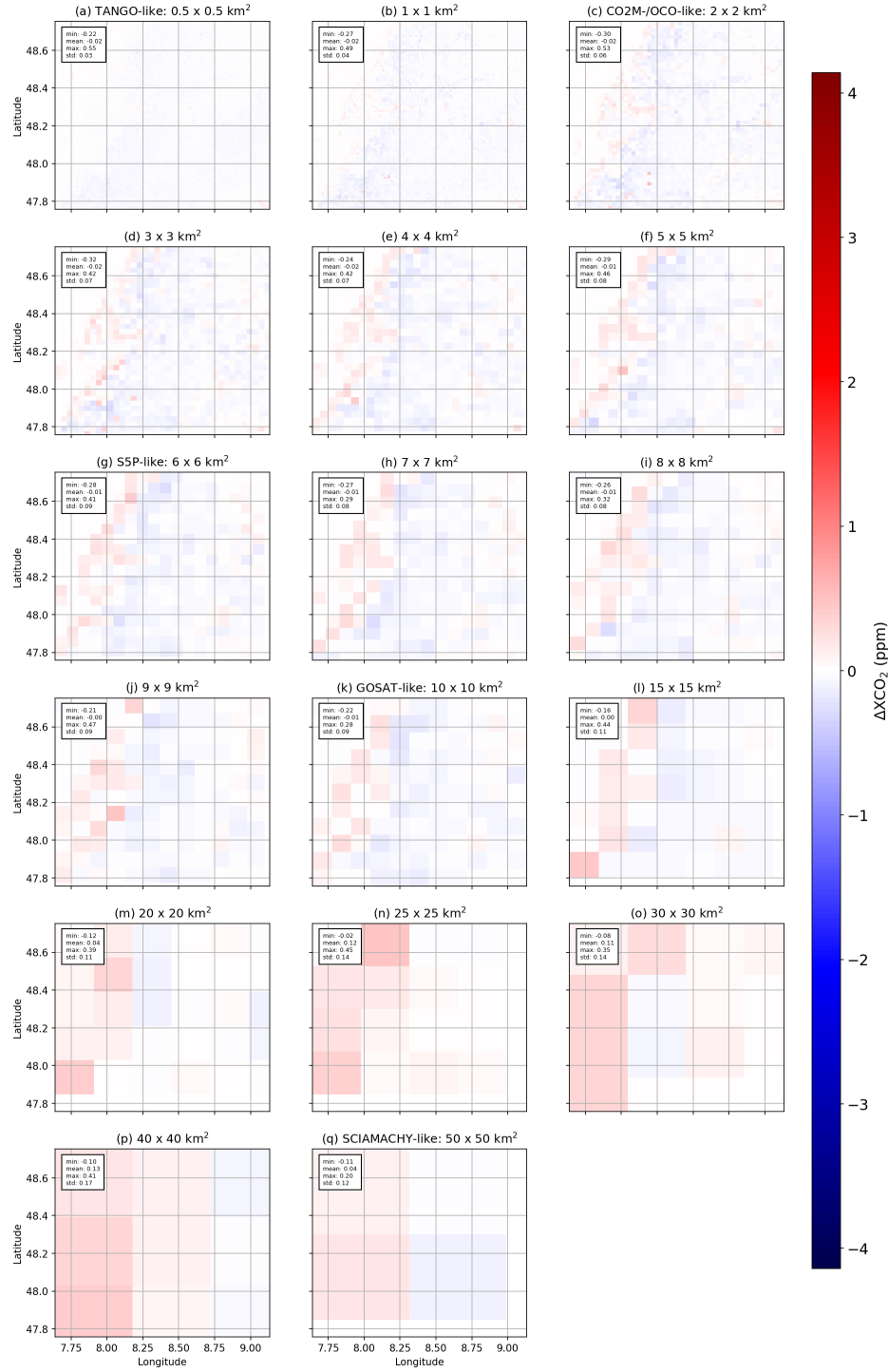
Figure S8. \Delta XCO_2 with variable size of the spatial samples as in the right column of Fig. 21 of the main text, but for more spatial sample sizes.
