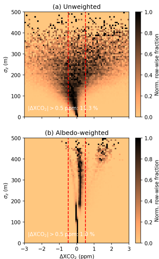
Figure 17. Normalized occurrence frequency of \Delta\text{XCO}_2 for surface roughness values between 0 and 500m using (a) the unweighted and (b) the albedo-weighted surface altitude. The frequencies in each row are normalized such that the maximum value is always one, for illustration purposes. The red dotted lines correspond to the accuracy requirement of \pm 0.5 ppm for CO2M (ESA, 2020).
