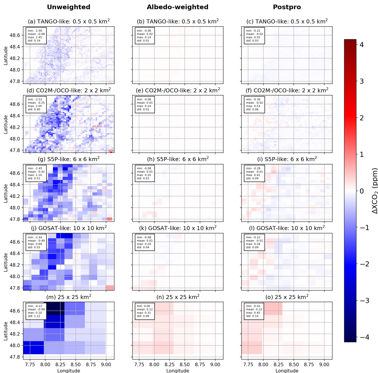
Figure 21. \Delta\text{XCO}_2 values for spatial samples of different sizes, defined on a regular latitude-longitude grid, corresponding to the size in the title of each panel using the unweighted average (first column) and the albedo-weighted average of the surface altitude (second column) and after applying the post-processing correction (third column). The region shown is the Black Forest. Each panel includes the minimum, average and maximum values of \Delta\text{XCO}_2 in the region shown. The titles of the panels indicate the spatial sample sizes that are closest to known Note that there are more examples in the Supplement of this study (Figs. S6 to S8).
