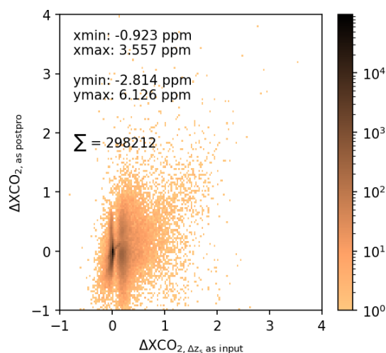
Figure 20. Deviation from 400ppm when applying the post-processing given in Eq. (30) (y-axis) and using the albedo-weighted averaged surface altitudes in each wavelength band \Delta z_s directly as input for the retrieval (x-axis). Note the logarithmic color scale.
