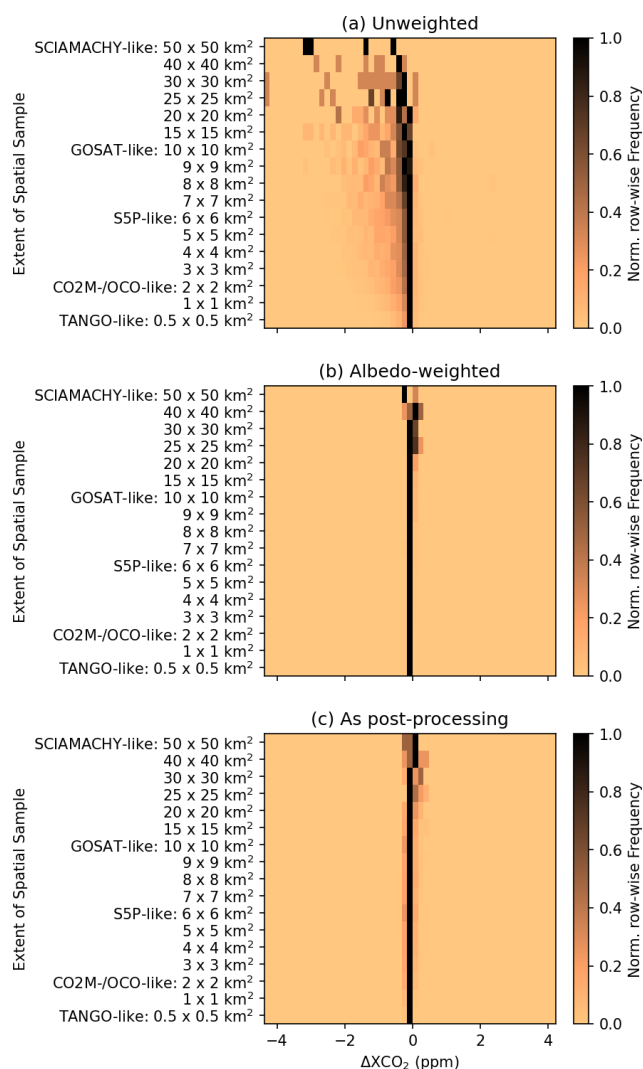
Figure 22. Normalized occurrence frequency of \Delta\text{XCO}_2 values in the Black Forest region using the (a) unweighted and (b) albedo-weighted average of the surface altitude, and (c) after applying the post-processing equation.
