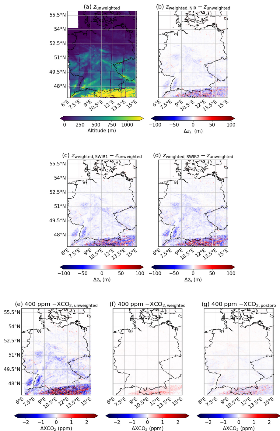
Figure 15. Same as Fig. 9, but for the whole country of Germany. We added a figure with the complete color scales to the Supplement of this study (Fig. S5).
