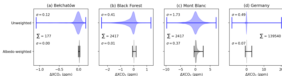
Figure 16. Variability of \Delta\text{XCO}_2 for the regions discussed in this section: (a) Bełchatów, (b) Black Forest, (c) Mont Blanc and (d) Germany. Note that the total number of data points differs largely between the panels. The \sigma values correspond to the standard deviations of the \text{XCO}_2 values (in ppm).
