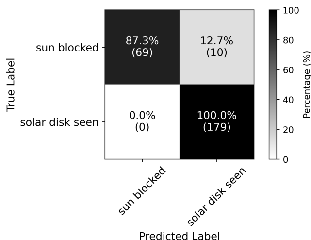
Figure 5. Confusion matrix of the solar disk state classification algorithm output against the testing data.
