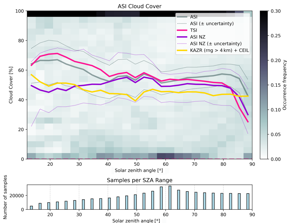
Figure 9. (Top) ASISKYCOVER-determined cloud cover occurrence frequency histogram as a function of SZA (bin sizes of 4 % and 3°, respectively) normalized for each SZA bin (i.e., each column of histogram bins sums to 1) for SGP in 2024. The mean cloud cover as a function of SZA is illustrated by the grey curve, with the dotted grey curves designating the mean \pm sample uncertainties. The pink and yellow curves designate the mean cloud cover as a function of SZA for the TSI and the 5 min running average combination of ceilometer cloud base detections and KAZR moderate sensitivity (MD) mode echoes above 4 km, respectively (see Sect. 3.1). The purple solid and dotted curves represent the 5 min running average mean and mean \pm sample uncertainty cloud cover as a function of SZA determined using the ASISKYCOVER near-zenith product (NZ; see text), rendering a more equivalent comparison to the KAZR-CEIL data. (Bottom) The total number of samples (images) per SZA bin range.
