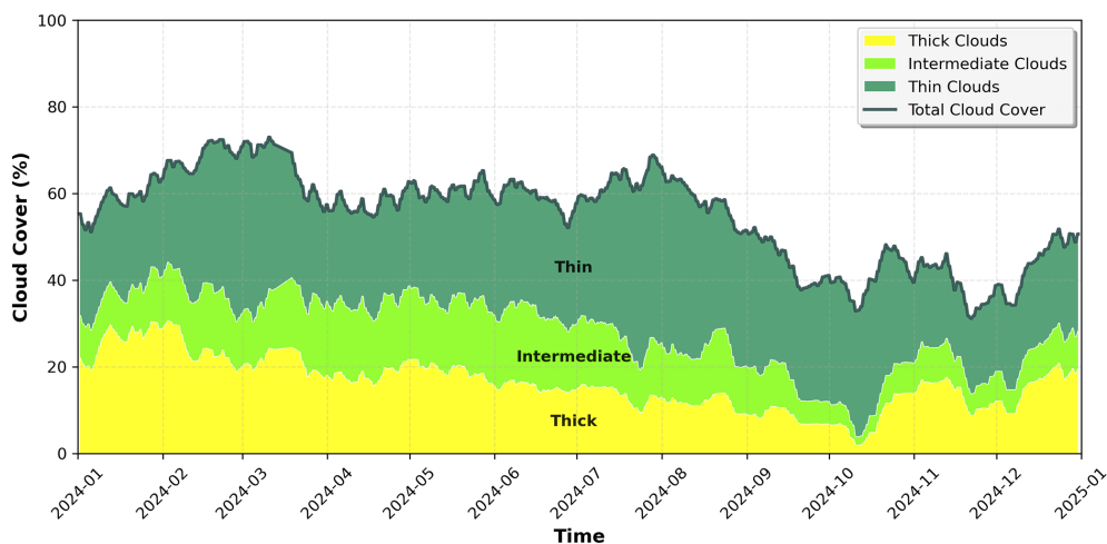
Figure 7. Cloud cover 31 d running-mean time series for the SGP site as determined by ASISKYCOVER for 2024. The stacked colored areas represent the distribution of cloud types (see legend and labels).
