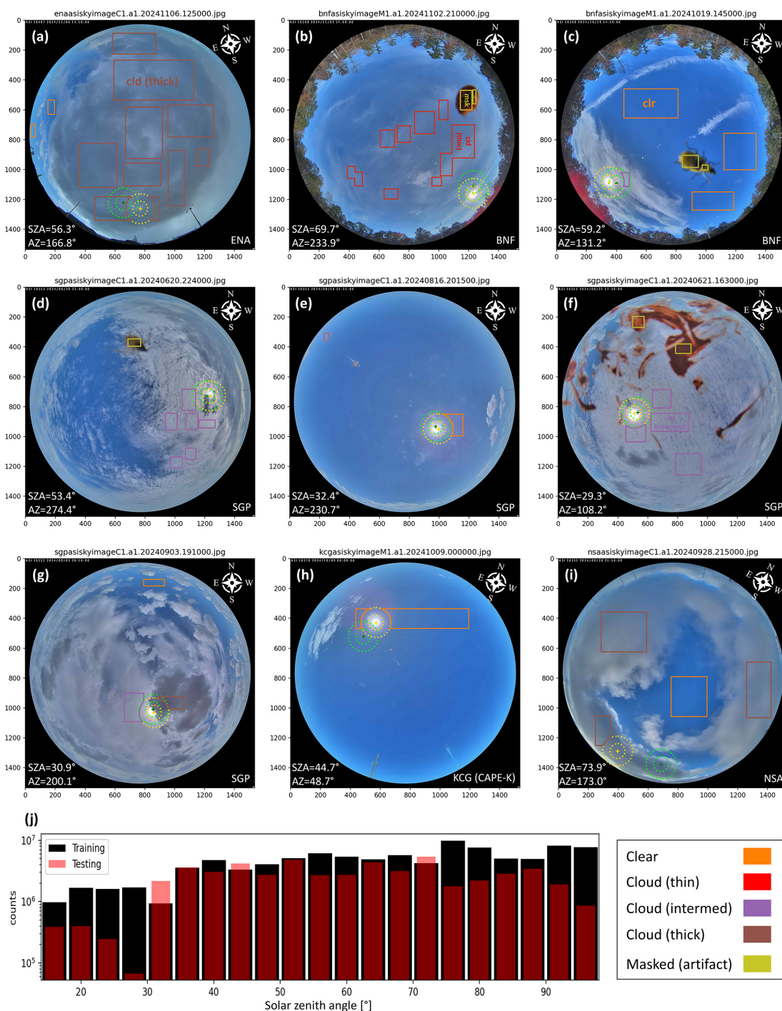
Figure 2. (a–i) Examples of images from different ARM deployments with manually labeled sectors of clear (orange), thin clouds (red), intermediate-thick clouds (purple), thick clouds (brown), and artifacts (masked; yellow), which are included in the training dataset (see legend and a selected set of in-box labels). In the depicted images, the x - and y -axis values represent pixel indices. The compass rose at the top right of each panel denotes the location of the north, south, east, and west directions, with compass tilting reflecting the site-specific solar misalignment. (Note that the ASI images appear mirrored in the east-west direction; see Sect. 2.1 for details.) The concentric green and yellow circles designate the analytically calculated and misalignment-corrected solar disk positions, respectively (outer circle radius of 100 pixels). Solar zenith and azimuth angles are shown at the bottom left corner of each image. The corresponding ARM deployments are shown at the bottom-right of each panel (ENA – Eastern North Atlantic; BNF – Bankhead National Forest; SGP – Southern Great Plains; KCG – Cloud And Precipitation Experiment at Kennaook; NSA – North Slope of Alaska). (j) Distribution of training (black) and testing (red) pixel samples as a function of solar zenith angle (SZA; bin size of 2°).
