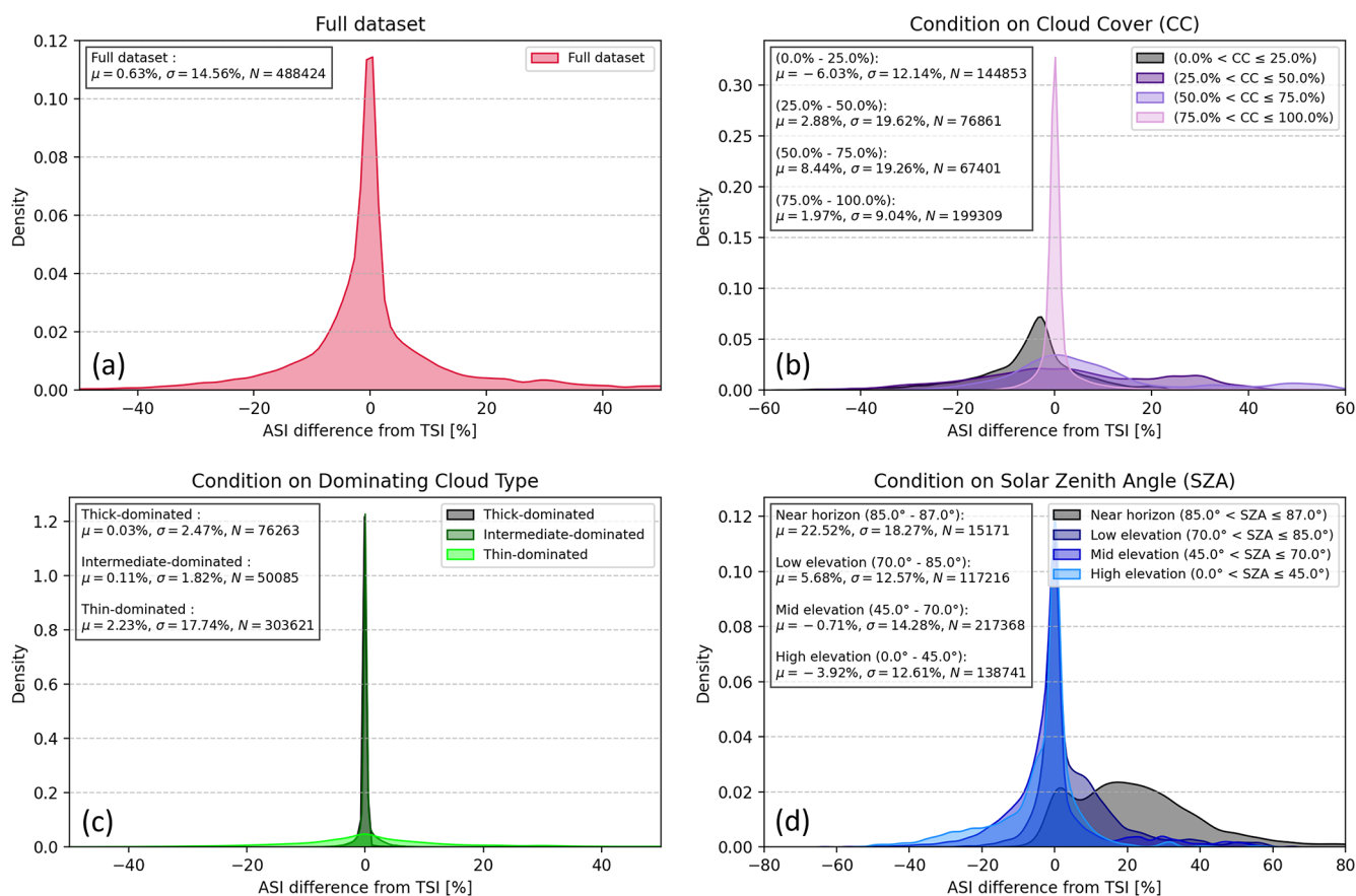
Figure 8. ASISKYCOVER deviations from the TSI cloud cover product kernel density estimations (KDEs) for SGP in 2024 while conditioning on different variables: (a) Full dataset (no conditioning), (b) ASISKYCOVER cloud cover (CC), (c) dominating cloud type per scene with CC greater than 5 % based on ASISKYCOVER, and (d) SZA (see legend). Mean deviation ( \mu ), standard deviation ( \sigma ), and number of TSI-ASISKYCOVER sample pairs in the conditioned data subset ( N ) are given on the top left of each panel.
