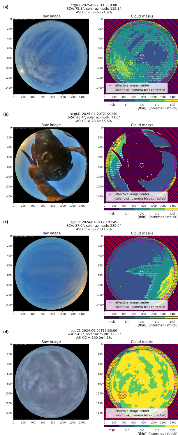
Figure 3. ASISKYCOVER pixel segmentation algorithm output for selected scenes. (Left) Raw ASI image (note that the ASI images appear mirrored in the east-west direction; see Sect. 2.1 for details), (right) algorithm output. The resolved classes are given in the legend at the bottom of the classification masks. In each classification mask, the red “+” denotes the determined image center, the dashed magenta and white circles designate the image areas covering up to 80 and 5° off-zenith, respectively, the white star marker indicates the corrected position of the solar disk, dotted white hatched areas denote uncertain classification pixels, and the dotted magenta hatched areas mark masked pixels (site mask + solar disk mask). The ASI image site, facility and time, as well as the corresponding SZA, azimuth angle, and algorithm-resolved cloud cover (following Sect. 2.3) are given in the title of each image pair.
