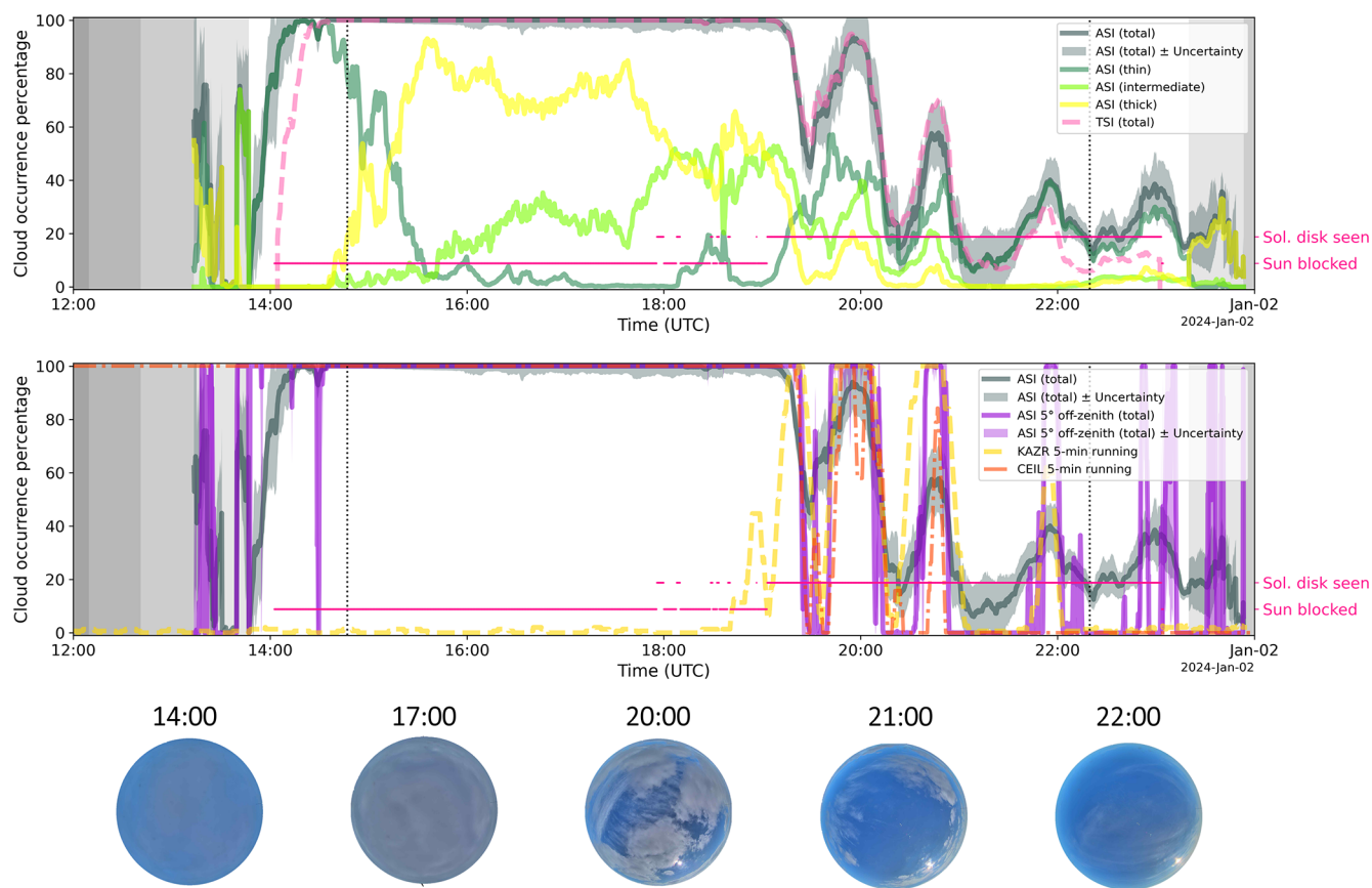
Figure 6. ASISKYCOVER cloud cover time series for the SGP central facility on 1 January 2024. (Top) Total cloud cover time series using the full 80^\circ off-zenith field-of-view together with time series for the three cloud classes (see legend). The light pink curve illustrates the TSI sky cover time series. The pink markers denote the solar disk state classification output (see right y-axis labels). The grey-shaded regions extending until nearly 14:00 UTC and from roughly 23:00 UTC designate (in decreasing brightness) the civil twilight, nautical twilight, astronomical twilight, and nighttime. The vertical dotted black lines denote 80^\circ SZA crosspoints. (Bottom) Similar, but showing the near-zenith ( 5^\circ off-zenith) product time series together with the 5 min running mean Ka-band ARM Zenith Radar (KAZR; using moderate sensitivity mode echoes above 4 km range) and ceilometer cloud occurrence (see legend). A selected set of raw ASI images are shown at the bottom of the figure together with their corresponding times. (Note that the ASI images appear mirrored in the east-west direction; see Sect. 2.1 for details.)
