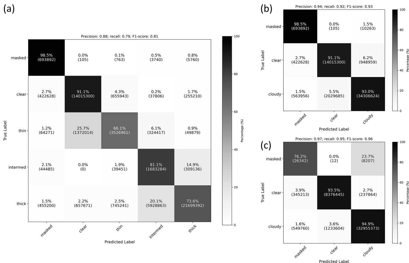
Figure 4. Confusion matrices of the segmentation algorithm output against the testing dataset. (a) Using all segmentation algorithm classes; (b) merging all cloudy classes to focus on cloudy-clear separation; and (c) same, but excluding testing samples with SZA exceeding 80^\circ . The weighted precision, recall, and F1-score metrics for each testing subset are given in panel titles.
