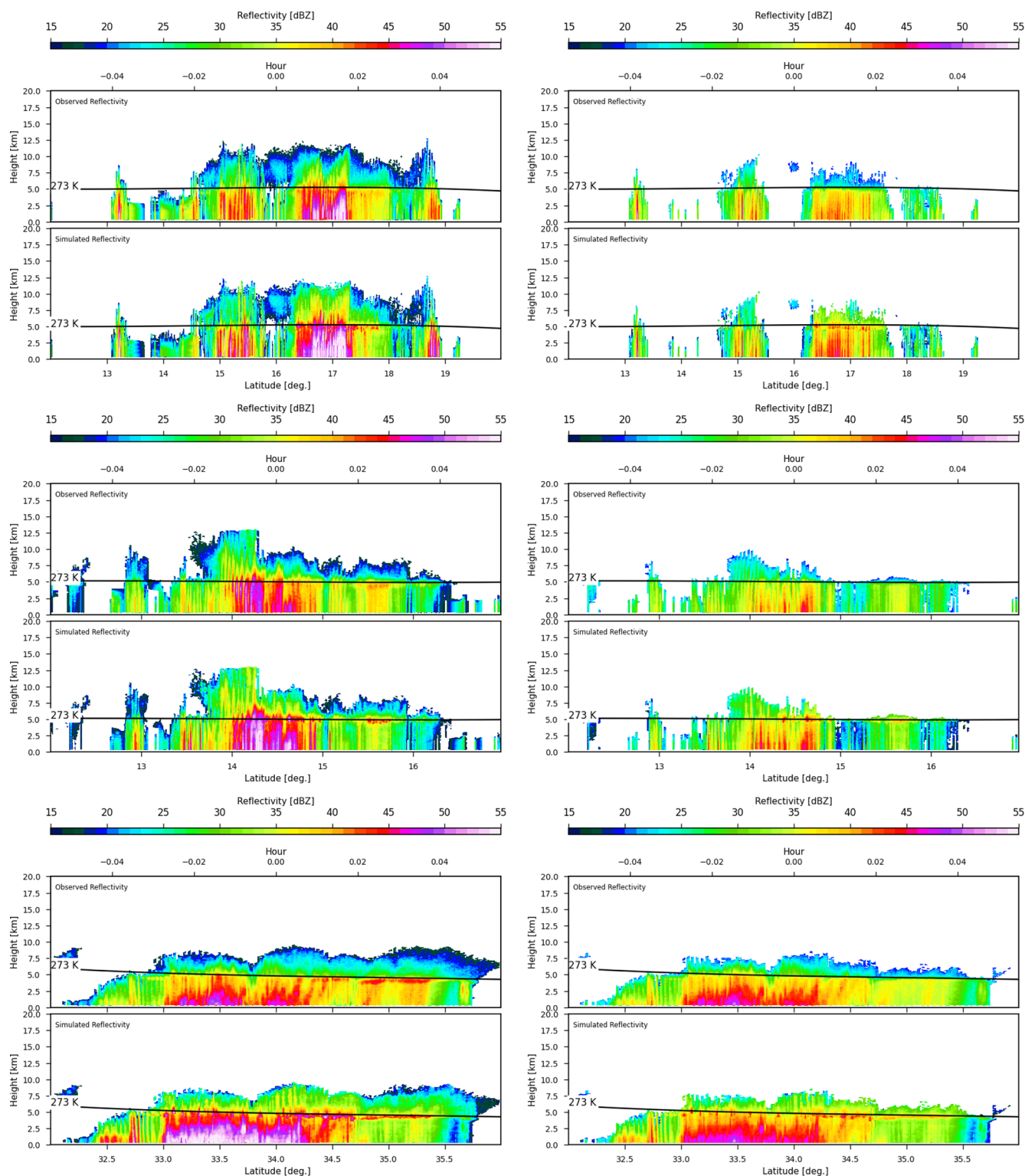
Figure 3. Observed vs. simulated GPM DPR reflectivities for Ku (left) and Ka (right) bands during Hurricane Irma (5 September 2017, 16:50 UTC), Hurricane Maria (18 September 2017, 02:01 UTC), and Hurricane Jose (18 September 2017, 03:39 UTC).
