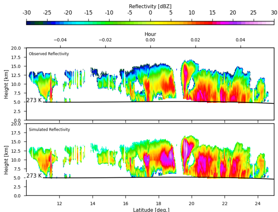
Figure 1. Simulated vs. observed CloudSat CPR reflectivities for Hurricane Bill on 19 August 2009, at 17:19 UTC. Simulations include contributions from liquid cloud, ice cloud, and snow water content.
