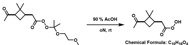
Figure A15. Cis -2-(3-Acetyl-2,2-dimethylcyclobutyl)ethaneperoxoic acid ( 7 ).
