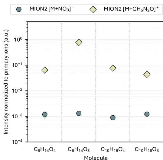
Figure 6. Intensities normalized to primary ions for nitrate and uronium adduct peaks of PNPA ( C_9H_{14}O_4 ), PPA ( C_{10}H_{16}O_4 ), and their corresponding carboxylic acids (NPA ( C_9H_{14}O_3 ) and PA ( C_{10}H_{16}O_3 )). Symbols represent mean intensities, and shaded areas indicate standard uncertainties calculated from all repeated syntheses and measurements. If no error bar is visible, it is obscured by the symbol.
