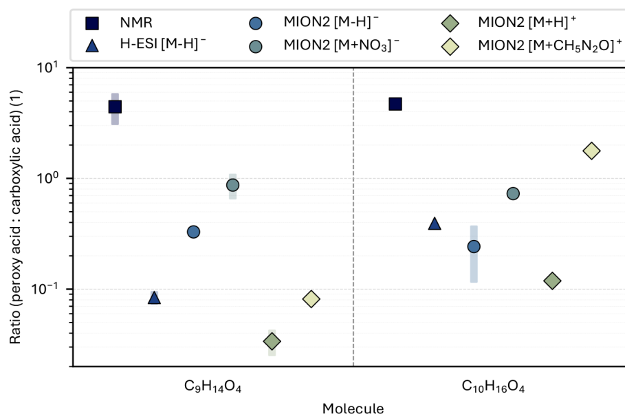
Figure 3. Ratios of peroxy acids to their corresponding carboxylic acids for PNPA ( C_9H_{14}O_4 ) and PPA ( C_{10}H_{16}O_4 ) measured by NMR and MION- and H-ESI-Orbitrap. Symbols represent mean ratios, and shaded areas indicate standard uncertainties calculated from all repeated syntheses and measurements. If no error bar is visible, it is obscured by the symbol. Circles represent MION-Orbitrap operated with nitrate, and diamonds represent MION-Orbitrap operated with uronium.
