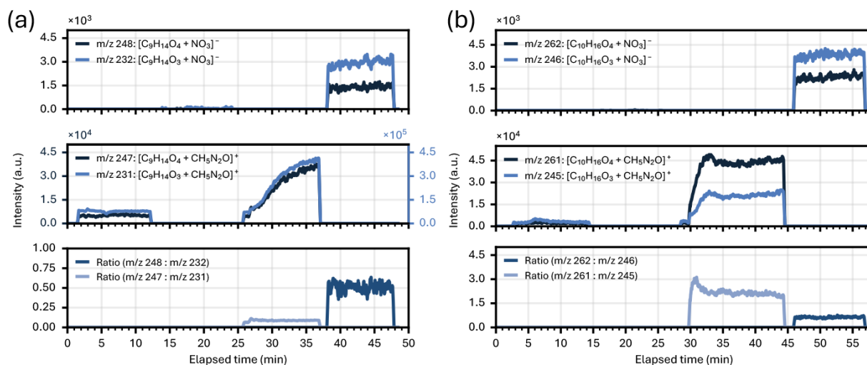
Figure 5. Extracted-ion chromatograms of the nitrate and uronium adduct ions of (a) peroxy norpinonic acid (PNPA; \text{C}_9\text{H}_{14}\text{O}_4 ; m/z 248 for the nitrate adduct and 247 for the uronium adduct) and norpinonic acid (NPA; \text{C}_9\text{H}_{14}\text{O}_3 ; m/z 232 for the nitrate adduct and 231 for the uronium adduct) and (b) peroxy pinonic acid (PPA; \text{C}_{10}\text{H}_{16}\text{O}_4 ; m/z 262 for the nitrate adduct and 261 for the uronium adduct) and pinonic acid (PA; \text{C}_{10}\text{H}_{16}\text{O}_3 ; m/z 246 for the nitrate adduct and 245 for the uronium adduct). Absolute intensities and the ratios (peroxy acid to carboxylic acid) are shown.
