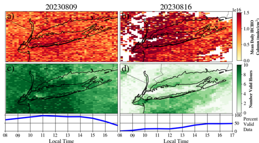
Figure 7. (a, b) Daily average TEMPO HCHO columns for NYC3 and NYC4 from 08:00–17:00 EDT. (c, d) Number of data points included in the average for each grid box and time series of the percentage of valid data in the domain.
