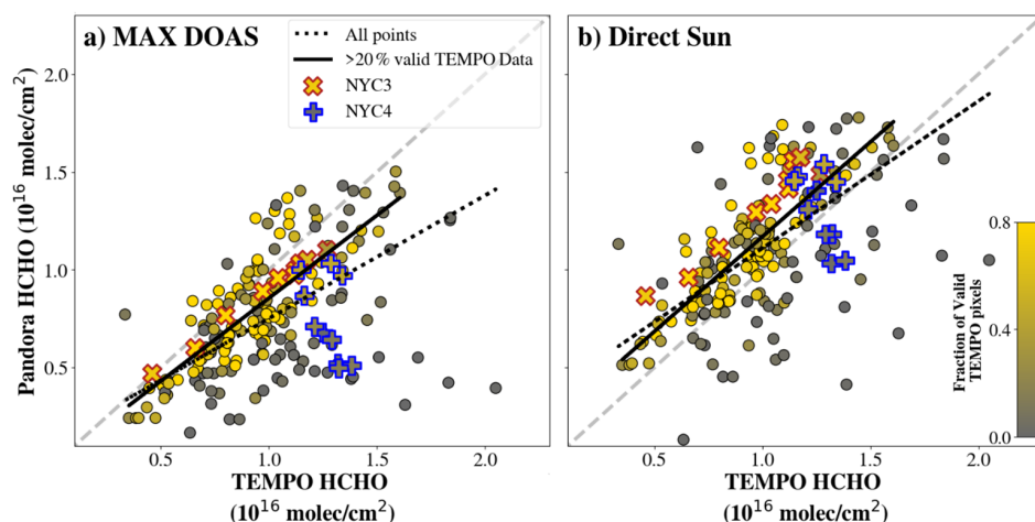
Figure 8. Average TEMPO HCHO column for the entire NYC domain (Fig. 4) versus average NYC Pandora MAX DOAS tropospheric column (a) and Direct Sun total column (b) from 2–31 August 2023. Each marker represents one hour of data and are colored by the percentage of available TEMPO data for the domain. Data from NYC3 and NYC4 are outlined as the red X's and blue crosses, respectively. Theil Sen lines of best fit for all data (dotted) and those with > 20 % valid data (solid) are included.
