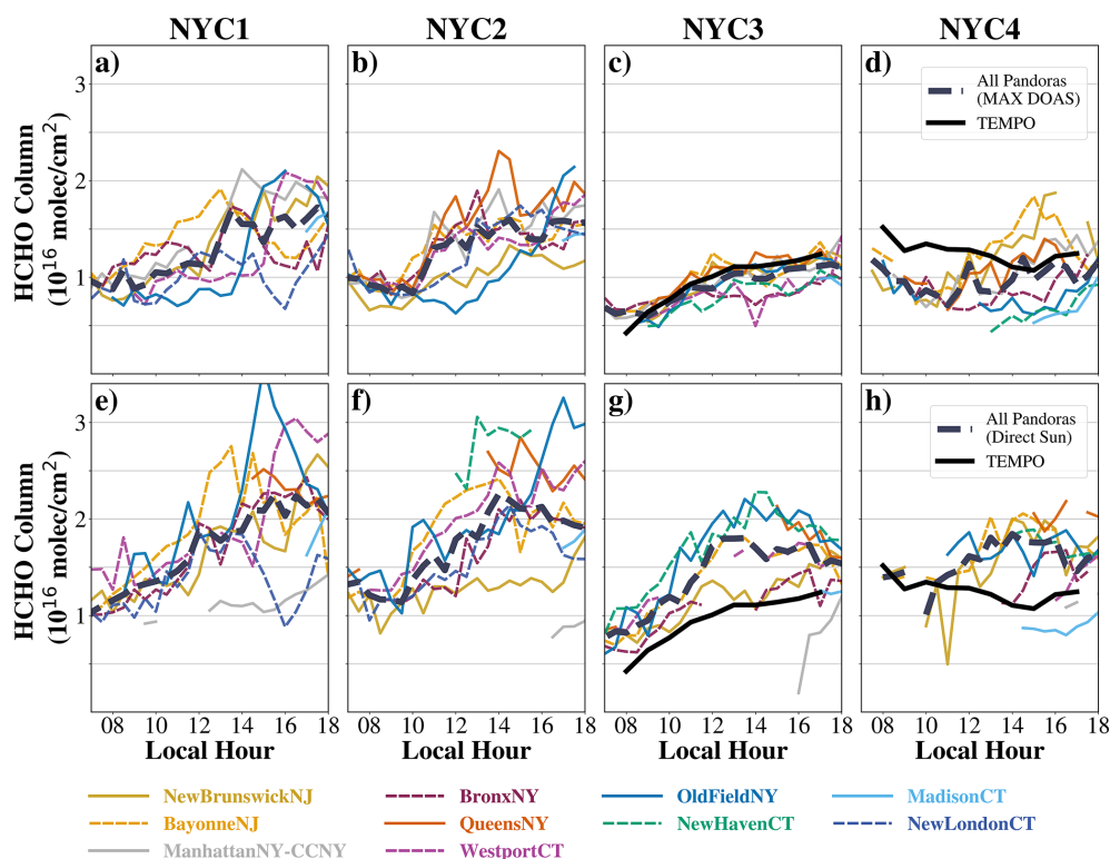
Figure 5. MAX DOAS tropospheric column (a–d) and DS total column (e–h) HCHO from NYC Pandoras on the four flight days averaged to 30 min. The individual stations are colored, and the mean value is shown as the dotted gray line. The hourly NYC domain (Fig. 4) average TEMPO HCHO column is included on NYC3 and NYC4 as the solid black line.
