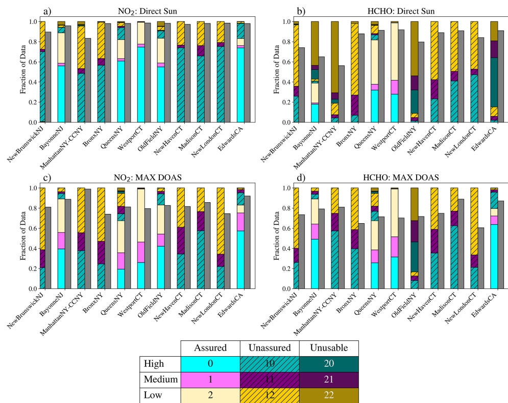
Figure 1. Distribution of the data quality flags for each station used in this study for (a) DS NO 2 , (b) DS HCHO, (c) MAX DOAS NO 2 , and (d) MAX DOAS HCHO. Gray bars indicate the portion of retained data for each station after applying the filtering method described in Sect. 2.2.1.
