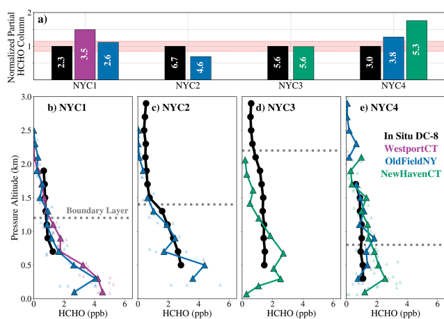
Figure 6. (a) HCHO partial columns from integrated in situ observations during DC-8 profiles and mean Pandora MAX DOAS scans during the same time frame ( \pm 45 min) from the nearest operational monitors normalized to the in situ column. Actual column values in molecules \text{cm}^{-2} are included as the white text on the bars. We include 15 % error (shaded red area) representing instrumentation accuracy of the in situ data; uncertainties for Pandora vertical profiles are not available. (b–e) Vertical profiles of HCHO from the NYC flights including the airborne in situ data (black solid line) and individual Pandora profiles (colored lines). Data are binned to 250 m (except the NewHavenCT profile on NYC3, which only has one Pandora profile during this time range). Dotted gray lines denote approximate boundary layer heights based on potential temperature gradients (not shown).
