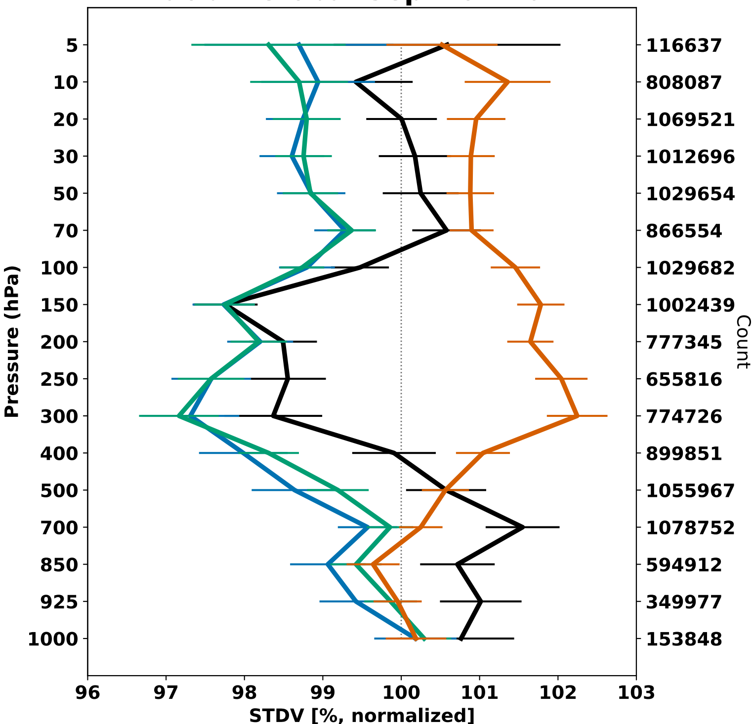
Raob-U Global Sep-Nov 2022
