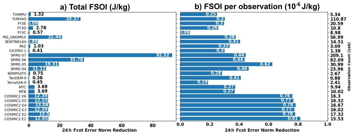
Figure 4. (a) Total forecast sensitivity to observation impact (FSOI, \text{J kg}^{-1} ) and (b) per-observation FSOI for all the ROMEX missions from September to November 2022 from the romex_n1 experiment. Spire instrument receiver IDs are grouped as follows: Spire 04 (99–102), Spire 05 (103–117), Spire 06 (118–125), and Spire 07 (126–169).
