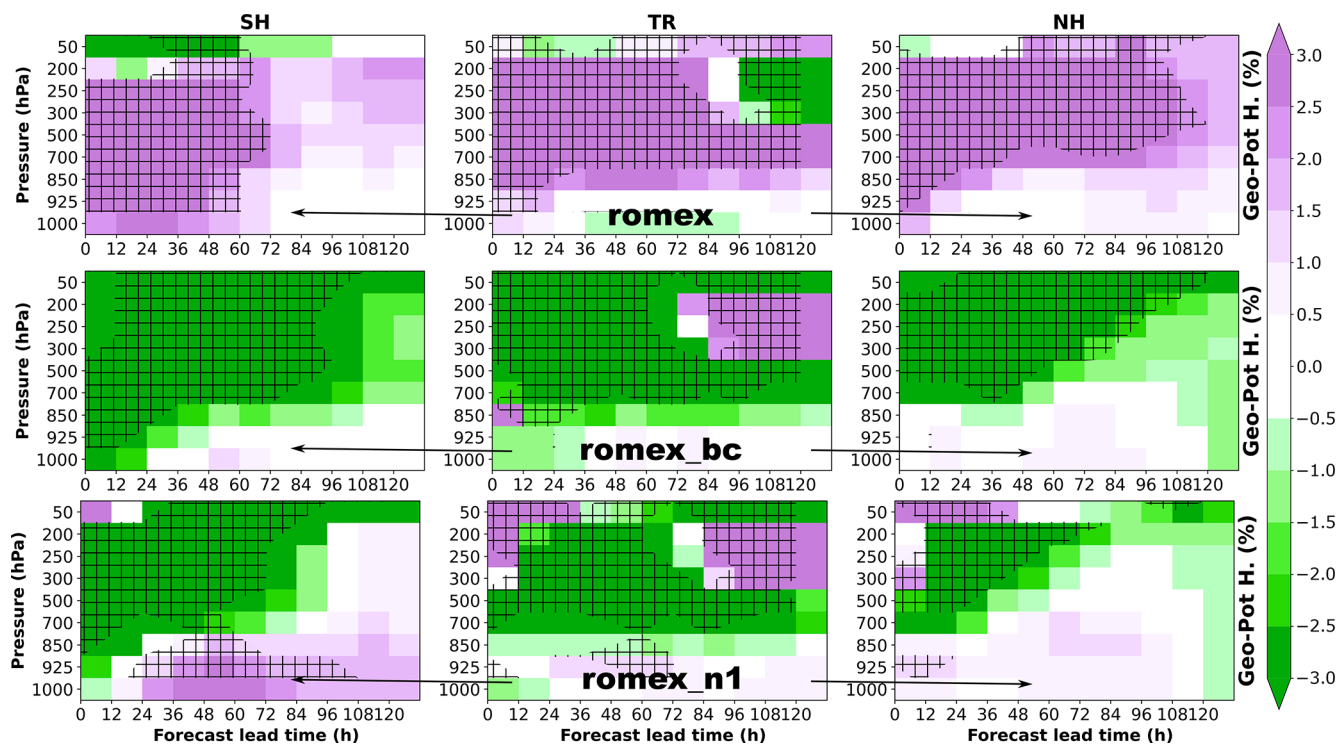
Figure 5. Percentage change in root-mean-square-error (RMSE) reduction for geopotential height forecasts in the “romex”, “romex_bc”, and “romex_n1” experiments relative to the control, verified against ECMWF analyses for September–November 2022. Forecast RMSE is computed every 12 h for the control and comparison experiment at three distinct regions: Southern Hemisphere (SH, 20–80° S), tropics (TR, 20° S–20° N), and Northern Hemisphere (NH, 20–80° N). Green shading indicates improved forecast skill from the assimilation of ROMEX observations, while purple shading signifies degraded skill. Hatched areas denote impacts that are statistically significant at the 95% confidence level.
