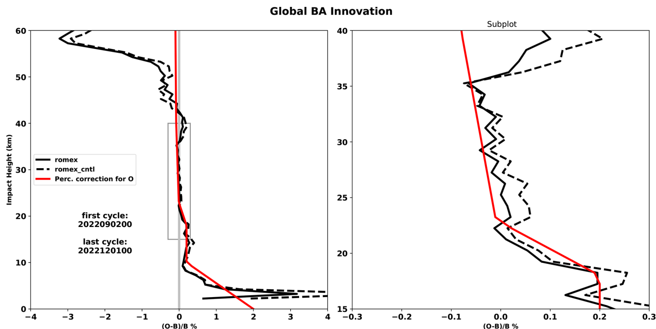
Figure 1. Global bending angle normalized innovation for the ROMEX experiment (“romex”) and the control experiment (“romex_cntl”) as a function of impact height. The empirical bias correction model derived from all ROMEX RO bending angle observations is also shown (red lines). The right panel shows a subplot of the left panel for impact heights between 15 and 40 km (grey box in the left panel).
