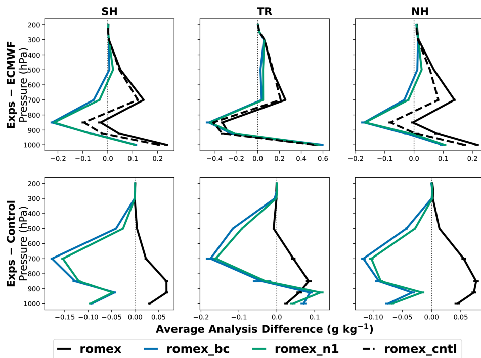
Figure 10. Same as Fig. 6, but for specific humidity (unit: \text{g kg}^{-1} ).
