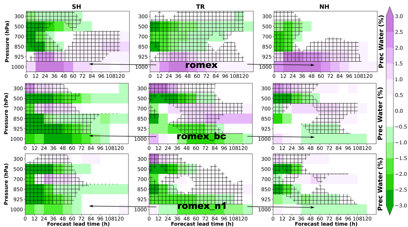
Figure 9. Same as Fig. 5, but for precipitable water.
