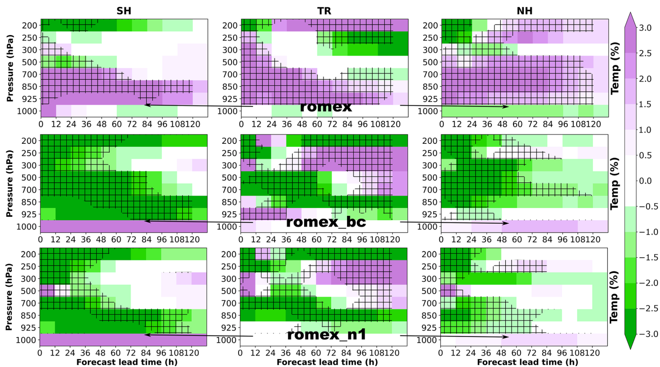
Figure 7. Same as Fig. 5, but for temperature.
