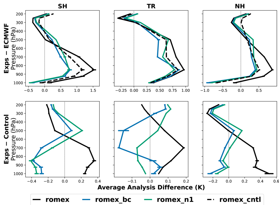
Figure 8. Same as Fig. 6, but for temperature (unit: K).
