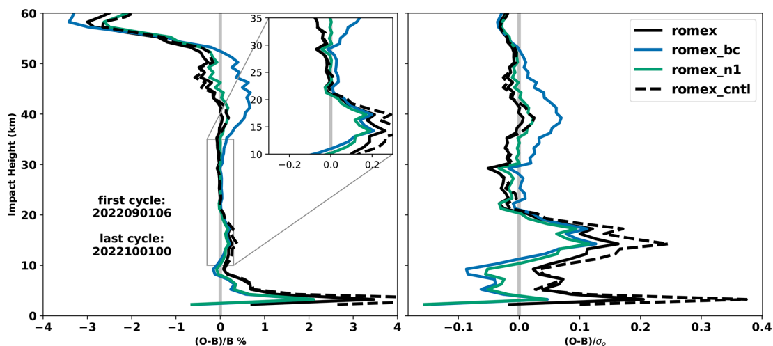
Figure 2. Global bending angle innovation normalized (a) by the background ( B ) and (b) by the observation error ( \sigma_o ) for the ROMEX experiment (“romex”), bias-corrected ROMEX experiment (“romex_bc”), adjusting refractivity coefficient ROMEX experiment (“romex_n1”), and the control experiment (“romex_cntl”) as a function of impact height.
