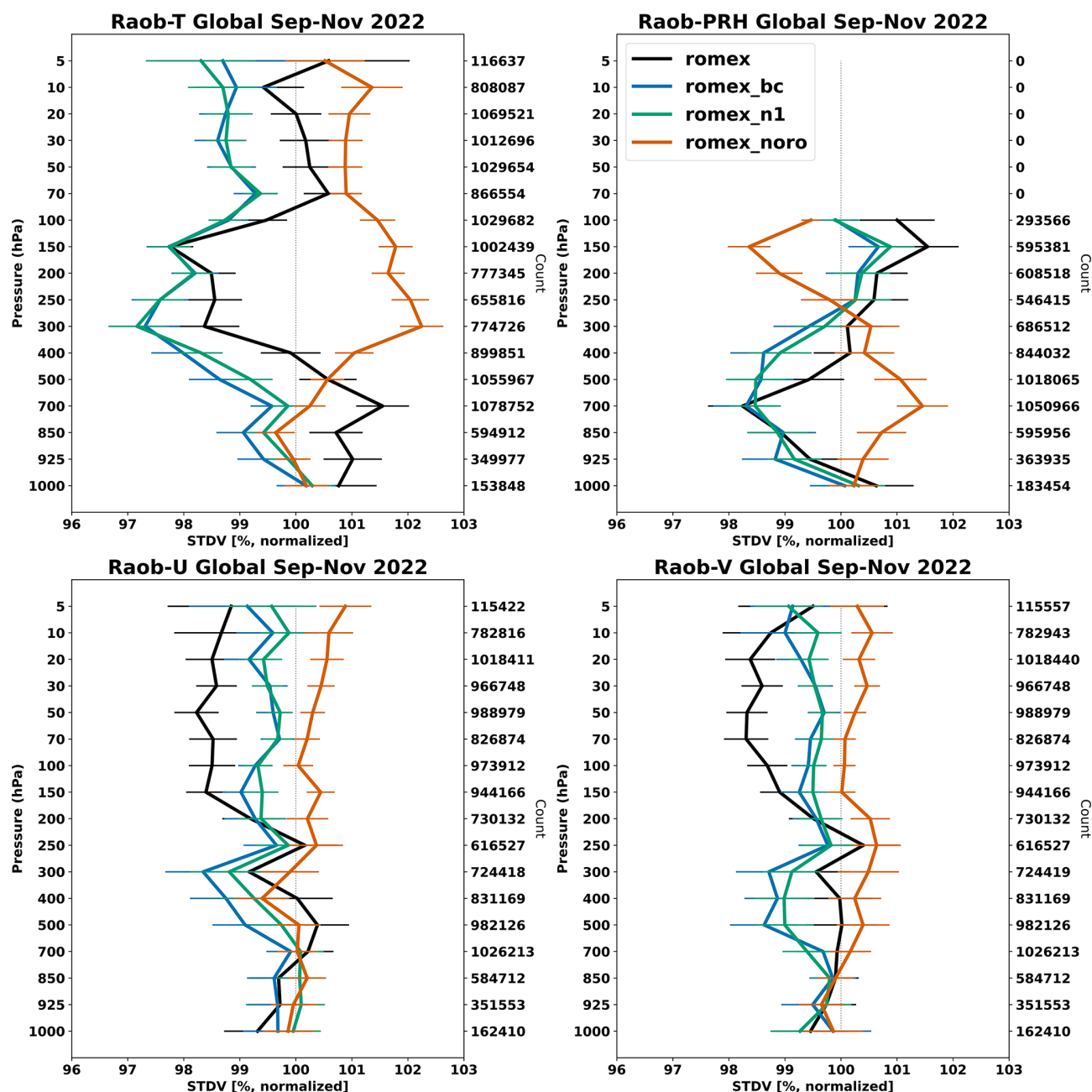
Figure 3. Change in standard deviation of observed minus background for radiosondes temperature, pseudo relative humidity (PRH), and zonal and meridional wind for ROMEX (“romex”), bias-corrected romex (“romex_bc”), adjusting the first refractivity coefficient ROMEX experiment (“romex_n1”), and the one without RO data (“romex_noro”) experiment relative to the ROMEX control experiment (“romex_cntl”) from September–November 2022. The number of observations is indicated on the vertical axis to the right, and the horizontal bars represent the 95 % significance level.
