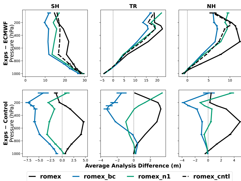
Figure 6. (Top) Mean geopotential height analysis bias (units: m) between each romex experiment (romex, romex_bc, romex_n1) and ECMWF analyses, (bottom) and between each romex experiment and the control run. Statistics are computed using analyses initialized at 00:00 and 12:00 UTC from 1 September–30 November for the southern hemisphere (SH), tropics (TR) and northern hemisphere (NH). Error bars indicate the 95 % confidence interval estimated using a two-sample t -test accounting for lag-1 autocorrelation (Wilks, 2011, 145–149). Note that the x -axis range in the top panel differs from that in the bottom panel.
