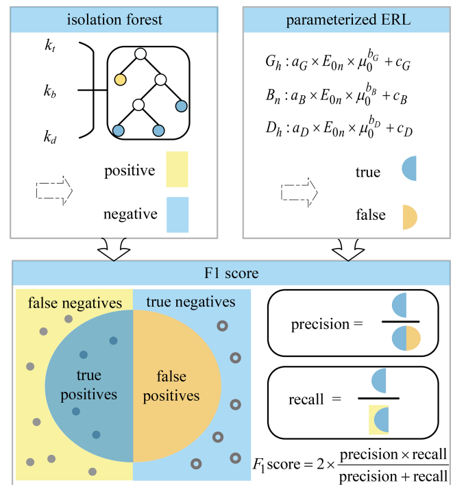
Figure 4. Workflow for configuring climatological QC limits. The procedure iteratively adjusts the parameters of two independent outlier detection algorithms to maximize the F_1 score derived from their agreement.
