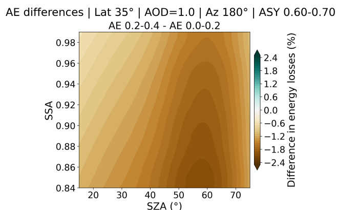
Figure 8. Differences in PV energy losses (%) as a function of solar zenith angle (SZA) and single-scattering albedo (SSA) for the Ångström exponent sensitivity analysis, under fixed latitude ( 35^\circ ), aerosol optical depth ( AOD = 1.0 ), south-facing orientation ( Az = 180^\circ ), and asymmetry parameter range ASY = 0.60\text{--}0.70 . The panel shows the difference in losses between the AE intervals 0.2–0.4 and 0.0–0.2.
