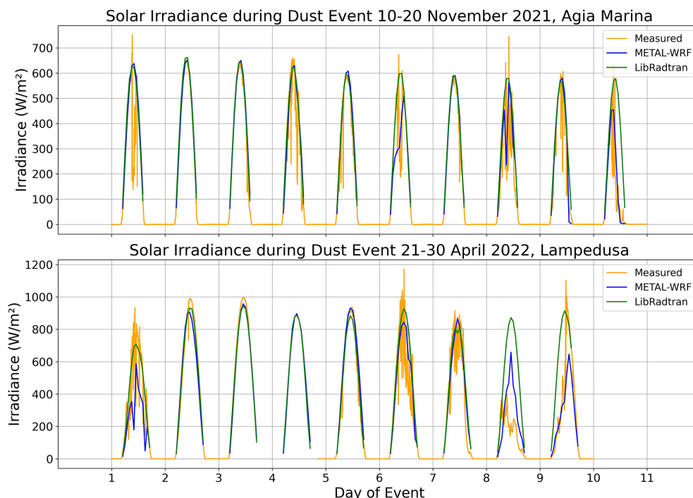
Figure 10. Timeseries of the GHI at Agia Marina Xyliatou, Cyprus, during event C (upper panel) and Lampedusa, Italy, during Event D (lower panel). In the case of AMX, during days 2, 3, 5 and 7 clear-sky conditions dominated, while in the case of Lampedusa, days 1, 6, 7, 8 and 9 indicated cloudy conditions.
