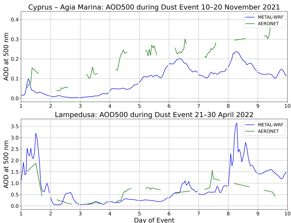
Figure 11. AOD at 500 nm from AERONET (green line) and METAL-WRF (blue line) for Agia Marina Xyliatou (upper panel) and Lampedusa (lower panel). The presented AERONET values are those interpolated to the time of the simulations as described in Sect. 2.3.
