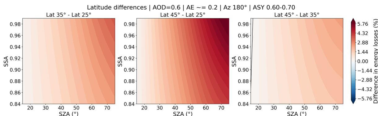
Figure 6. Differences in PV energy losses (%) as a function of solar zenith angle (SZA) and single-scattering albedo (SSA) for the latitude sensitivity analysis, under fixed aerosol optical depth ( AOD = 0.6 ), Ångström exponent ( AE \approx 0.2 ), south-facing orientation ( Az = 180^\circ ), and asymmetry parameter range ASY = 0.60\text{--}0.70 .
