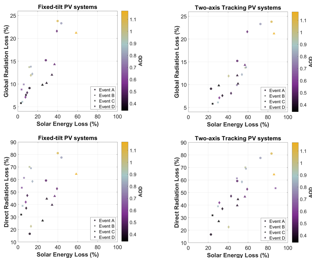
Figure 5. Global (top panel) and direct (lower panel) radiation losses (%) versus losses in produced PV solar energy (in %) during the four dust events for fixed-tilt PV systems (left) and two-axis tracking systems (right), along with AOD.
