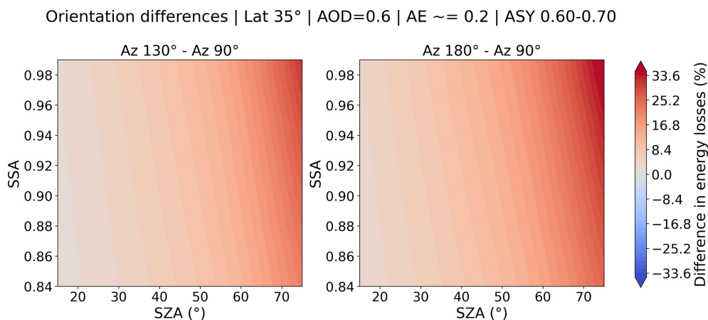
Figure 9. Differences in PV energy losses (%) as a function of solar zenith angle (SZA) and single-scattering albedo (SSA) for the panel-orientation sensitivity analysis, under fixed latitude (35°), aerosol optical depth (AOD = 0.6), Ångström exponent (AE \approx 0.2), and asymmetry parameter range ASY = 0.60–0.70.
