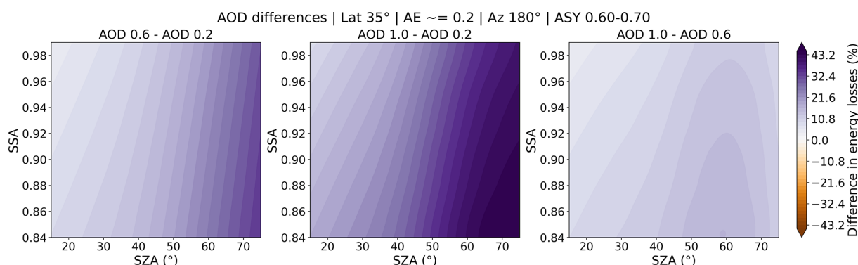
Figure 7. Differences in PV energy losses (%) as a function of solar zenith angle (SZA) and single-scattering albedo (SSA) for the AOD sensitivity analysis, under fixed latitude ( 35^\circ ), Ångström exponent ( AE \approx 0.2 ), south-facing orientation ( Az = 180^\circ ), and asymmetry parameter range ASY = 0.60\text{--}0.70 . Panels show the pairwise differences in losses between AOD values of 0.6 and 0.2, 1.0 and 0.2, and 1.0 and 0.6.
