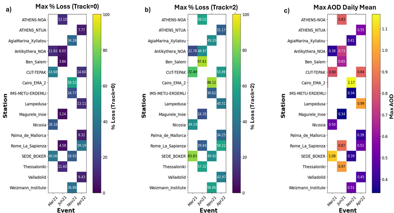
Figure 4. Losses (in %) in produced solar energy in the day of the maximum (daily average) AOD a) for fixed-tilt PV systems (Tracking = 0), two-axis tracking systems (Tracking = 2), along with (c) the maximum observed (daily average) AOD values.
