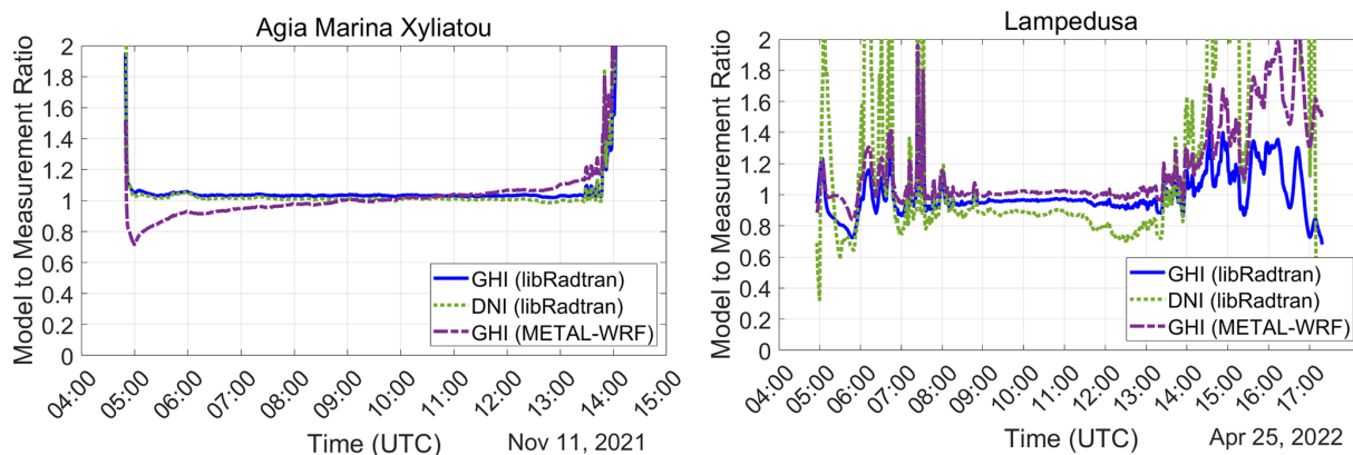
Figure 13. Ratios of modelled (libRadtran and METAL-WRF) to measured irradiances for a selected day at Agia Marina Xyliatou (left) and Lampedusa (right). GHI and DNI as calculated from the libRadtran model have been compared with the respective measured components, while only the comparison of GHI is presented in the case of METAL-WRF.
