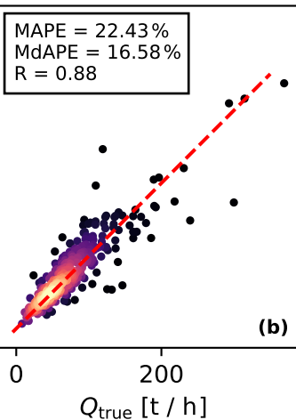
WRFChem with ERA5
