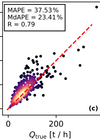
HYSPLIT with ERA5
