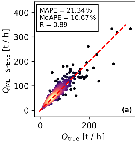
WRFChem with NCEP
