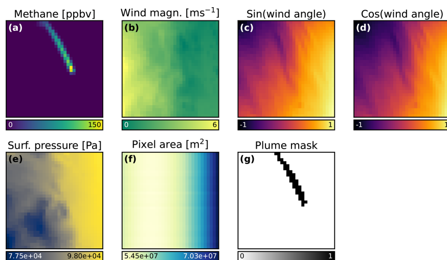
Figure 1. Channels used for input to ML-SPERE. All channel dimensions are 32 \times 32 TROPOMI pixels. (a) Methane channel. For training and validation data, resampled plume abundances are provided, but test dataset methane scenes must be background-reduced and masked to zero outside of the defined plume mask as described in Sect. 2.2 and shown in Fig. 2. (b–d) Wind vector information, split over three channels. (e) Surface pressure. (f) Pixel area. (g) Binary plume mask. Prior to input to ML-SPERE, each of the seven channels is standardized independently using channel-wise statistics (mean and standard deviation) computed across all training images.
