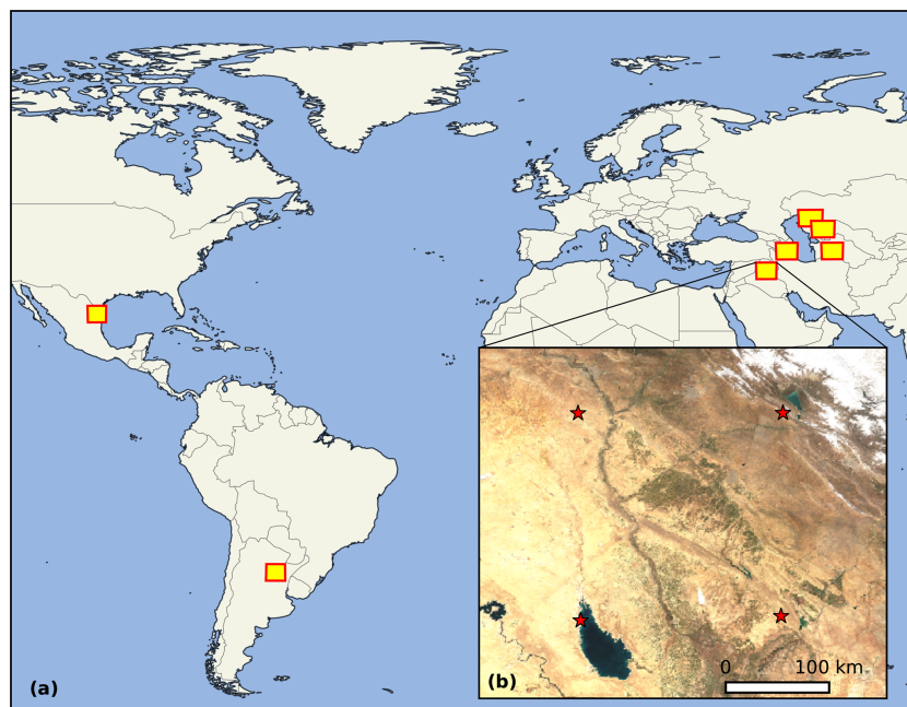
Figure A1. (a) The inner domain of the nested WRF-Chem setups, shown with the yellow rectangles. For each of these inner domains, 8 passive tracers are initialized to emit over the duration of the simulations, at 4 different locations and 2 different release heights. Tracer locations are shown with the stars in the example domain shown in (b), and at each star, tracers are initialized at approximately 25 and 250 m heights. Background imagery in (b) relies on non-concurrent Sentinel-2 data (2022) adapted from Google Earth Engine (Gorelick et al., 2017; European Union, 2026).
