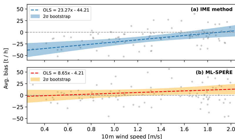
Figure 4. Estimate bias (expressed as the residual between an emission rate estimate for a method and the true emission rate) for HYSPLIT test set plumes, estimated via the IME method (a) and ML-SPERE (b) as a function of 10 m wind speeds. Also shown are ordinary least square regressions for both datasets. Due to the linear calibration of the effective wind speed to the input 10 m wind speed, the IME estimate residuals show a strong negative bias at low wind speeds, however ML-SPERE yields unbiased estimates at wind speeds below 2 \text{ m s}^{-1} .
