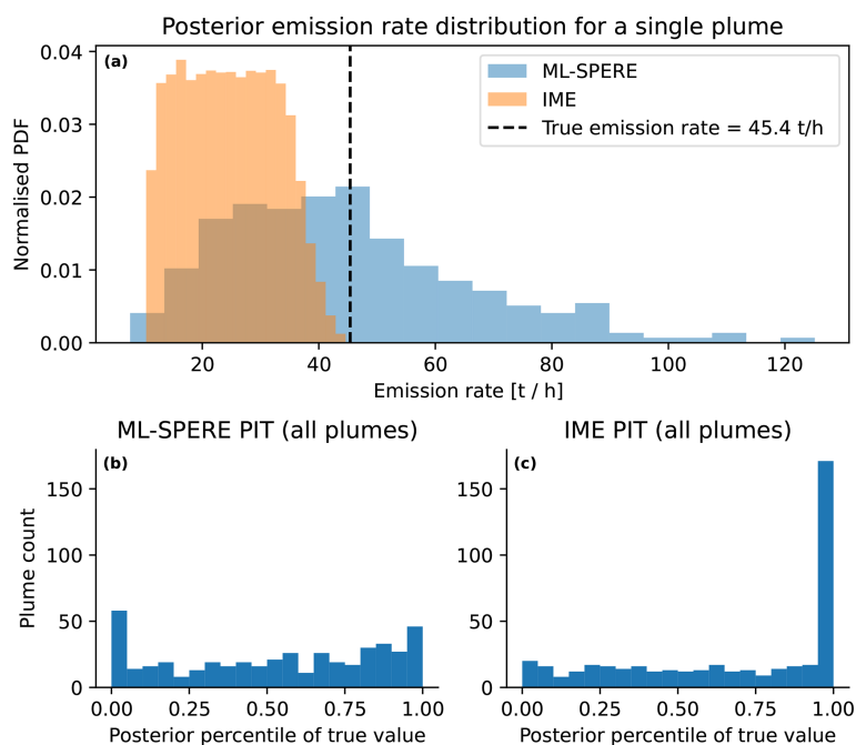
Figure A6. (a) Examples of estimated posterior emission rate distributions for a single scene via both ML-SPERE and the IME method. The true emission rate for this plume ( 45.4 \text{ t h}^{-1} ) lies at a posterior percentile of 0.57 for ML-SPERE, and 1 for the IME method. Calculating and binning such values for both methods and all plumes in the synthetic test set generates (b) the PIT for ML-SPERE and (c) the PIT for the IME method.
