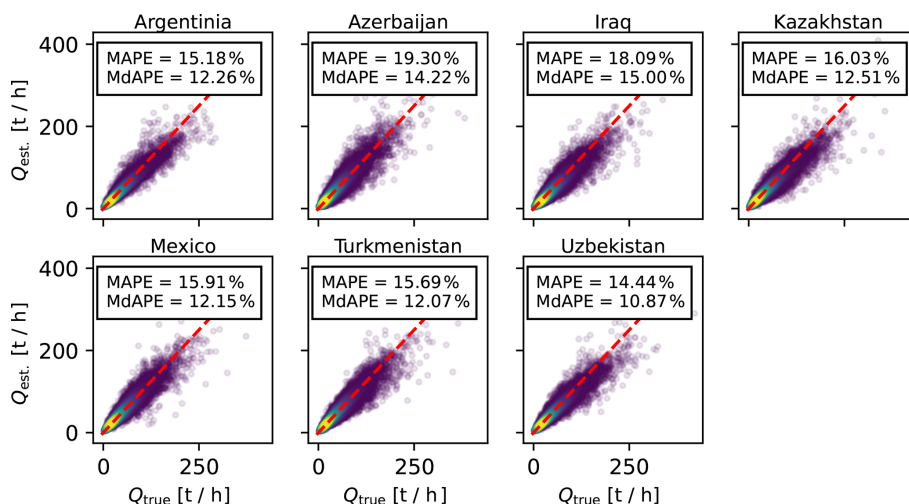
Figure A7. Visualizations of ML-SPERE estimated emission rates Q_{\text{est}} vs. true emission rates Q_{\text{true}} for each of the K -fold test sets. Values for MAPE and MdAPE are shown in each panel, and the red dashed lines show the 1 : 1 line. The colormaps represent the relative density of the visualised data.
