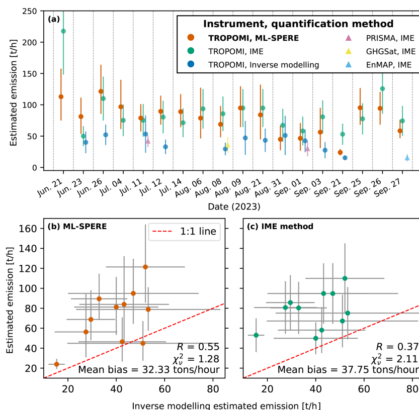
Figure 5. (a) Time series of daily estimated methane emission rates for the Karaturun East oilfield blowout. TROPOMI inverse modeling estimates and high-resolution satellite IME estimates are taken from Guanter et al. (2024). ML-SPERE data points are median values of the estimated posterior distribution of estimated emissions. Errorbars shown are \pm 1\sigma , with the exception of error bars for ML-SPERE estimates, which extend from the 16th to the 84th percentile of the posterior distribution of emission estimates (all statistics are given in Table A3). We choose to represent error bars for ML-SPERE with percentiles to show the skewed shape of the posterior distribution of the estimate (e.g. see Fig. A6a). (b) ML-SPERE estimates of the daily emission rate compared to the TROPOMI inverse modeling estimate for that same day. (c) IME estimates of the daily emission rate compared to the TROPOMI inverse modeling estimate for that same day.
