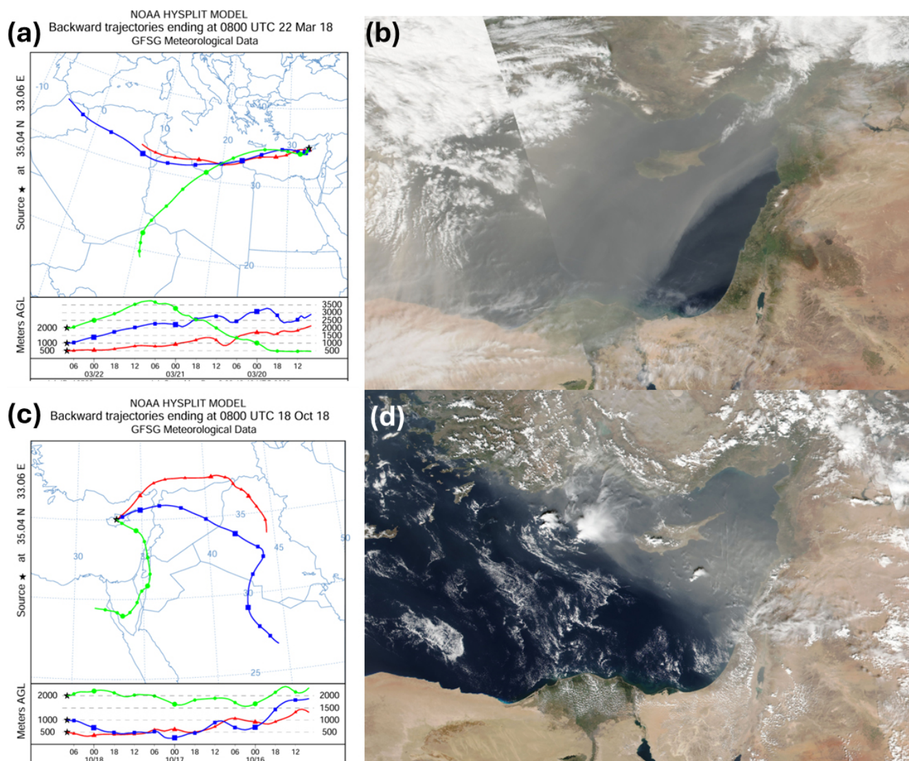
Figure 3. (a–b) Saharan dust event on 22 March 2018 and (c–d) Middle Eastern dust event on 18 October 2018 over Cyprus. Panels (a) and (c) show 72 h backward air mass trajectories calculated using the NOAA Hybrid Single-Particle Lagrangian Integrated Trajectory (HYSPLIT) model with reanalysis meteorological data. Trajectories are presented for three arrival heights, indicated by red, green, and blue lines, revealing distinct source regions for each event. Panels (b) and (d) display corresponding MODIS satellite imagery (GIBS/Worldview), illustrating the spatial extent and transport of dust over the region during the two episodes.
