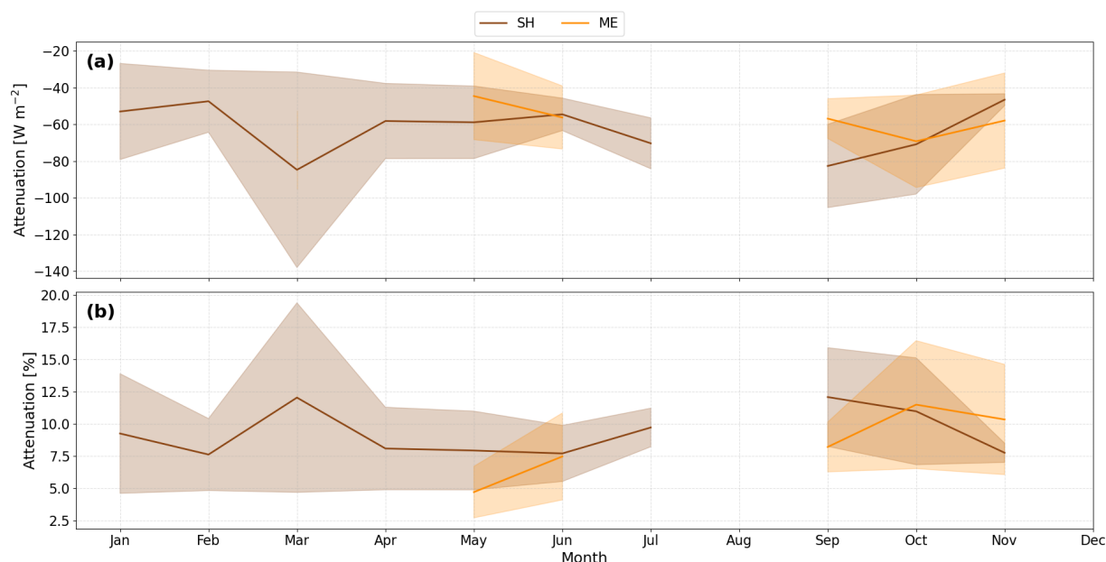
Figure 12. Seasonal variation in aerosol-induced attenuation of global horizontal irradiance (GHI) for Saharan (brown) and Middle Eastern (orange) dust events over Cyprus. (a) Monthly mean attenuation in absolute terms ( \text{W m}^{-2} ). (b) Monthly mean attenuation (%). Shaded areas represent \pm 1 standard deviation, indicating interannual variability.
