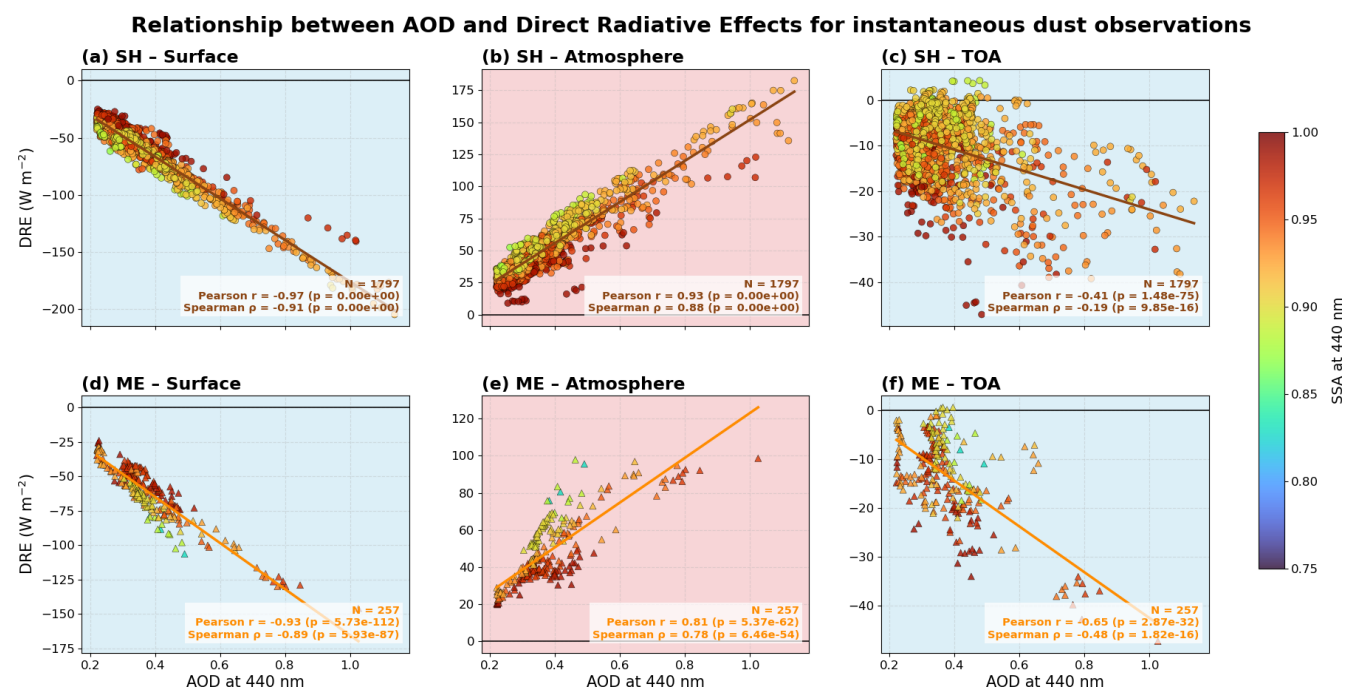
Figure 9. Relationship between aerosol optical depth at 440 nm ( AOD_{440} ) and instantaneous shortwave direct radiative effects (DRE) at the surface, atmosphere, and top of the atmosphere (TOA) for Saharan (SH; a–c ) and Middle Eastern (ME; d–f ) dust observations. Symbols are coloured according to the single-scattering albedo (SSA) at 440 nm. Solid lines represent linear regression fits. Pearson and Spearman correlation coefficients ( \rho ), associated p -values, and the number of observations ( N ) are reported in each panel.
