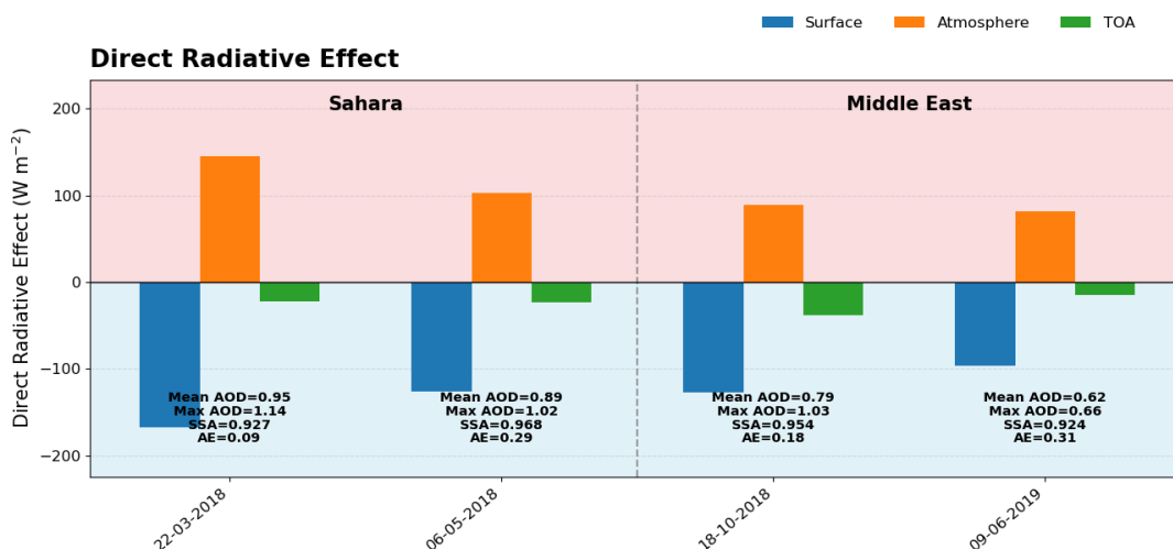
Figure 11. Daily mean DREs at the surface, within the atmosphere, and at the TOA for four selected dust events (22 March 2018, 6 May 2018, 18 October 2018, and 9 June 2019). Negative values indicate cooling (surface and TOA), while positive values represent atmospheric heating. Shaded regions highlight cooling (blue) and heating (red) regimes. Annotations provide mean and maximum AOD at 440 nm, along with SSA and Ångström exponent (AE) values for each case.
