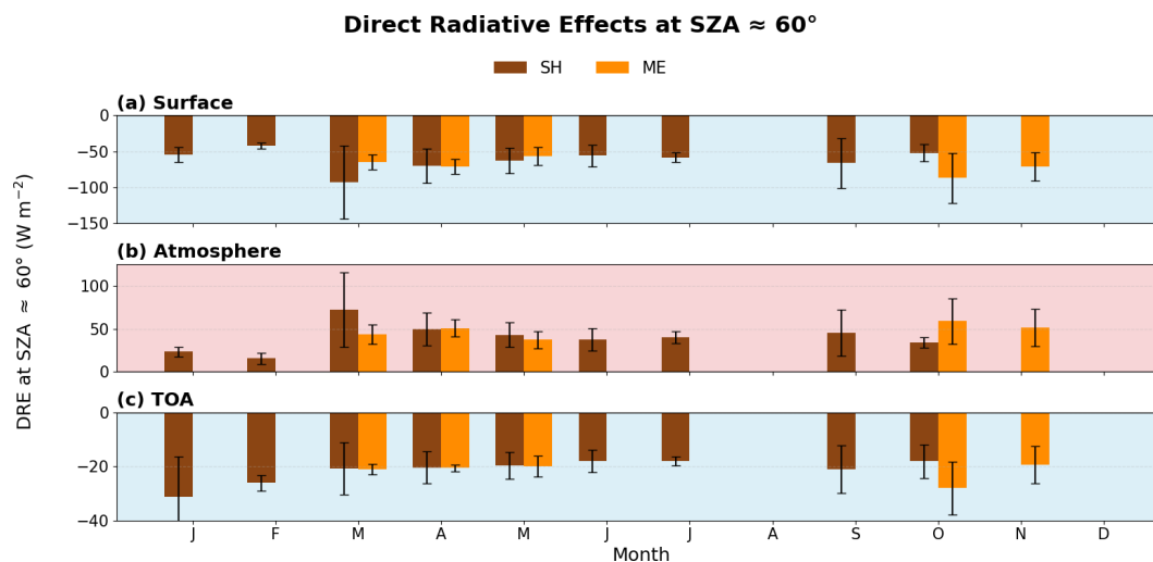
Figure 8. Monthly mean shortwave direct radiative effects (DRE, \text{W m}^{-2} ) at \text{SZA} = 60 \pm 4^\circ over AMX (2015–2022) under clear-sky conditions for (a) surface, (b) atmosphere and (c) TOA. Saharan dust is shown in brown and Middle Eastern dust in orange. Bars represent monthly mean values and error bars denote \pm 1 standard deviation. Background colours denote cooling (blue) and warming (red) effects.
