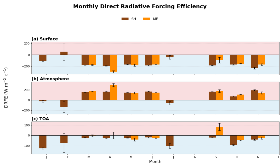
Figure 10. Monthly mean dust DRFE (in \text{W m}^{-2} \tau^{-1} ) over AMX (2015–2022) under clear-sky conditions for (a) surface, (b) within the atmosphere, and (c) TOA. Saharan dust events are shown in brown and Middle Eastern dust events in orange. Bars represent monthly mean values ( \text{W m}^{-2} ), and error bars denote \pm 1 standard deviation, indicating the intra-month variability of dust radiative effects. Background colors denote cooling (blue) and warming (red) effects.
