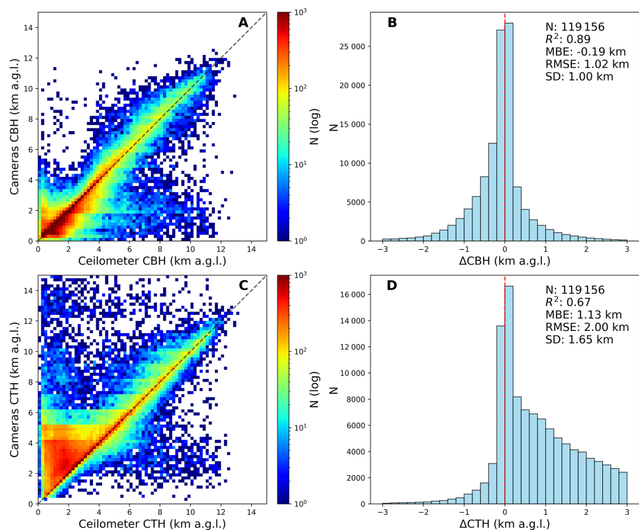
Figure 11. Bidimensional frequency histogram of camera values against ceilometer ones for cloud base height (CBH) and cloud top height (CTH) in panels (A) and (C), respectively. Colorbar represents the number of data of each bin in a log scale. Panels (B) and (D) represent the frequency histogram of the differences ( \Delta CBH and \Delta CTH) between both instruments. Statistical metrics provided include the total number of cases ( N ), coefficient of determination ( R^2 ), mean bias error (MBE), root mean square error (RMSE) and standard deviation (SD).
