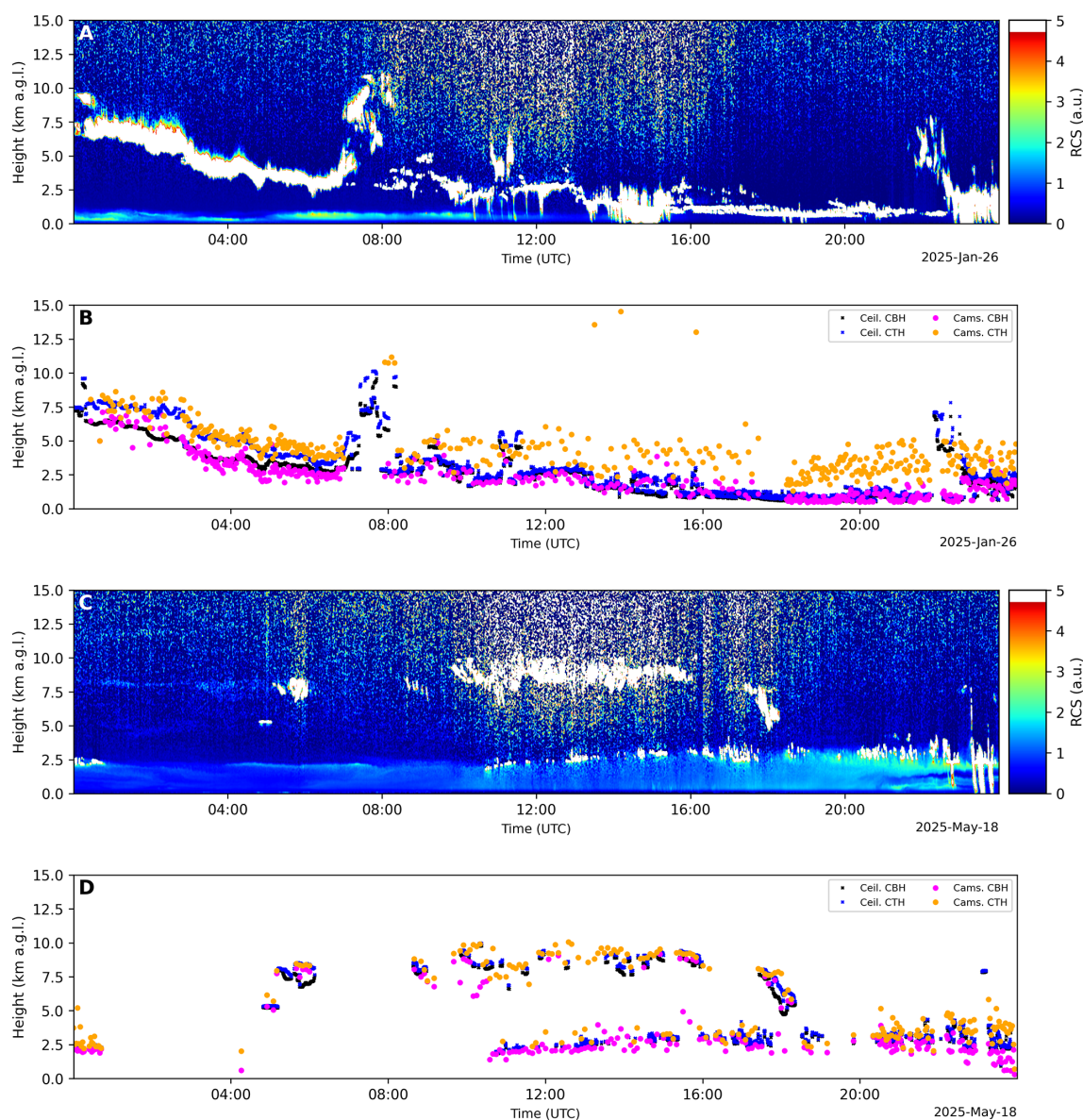
Figure 15. Temporal evolution for two different days of the ceilometer range corrected signal (RCS) overlaid with the cloud base and top heights (CBH and CTH) and those estimated by the all-sky camera network. Camera values are based on the median height value within a 150 m radius of the ceilometer location.
