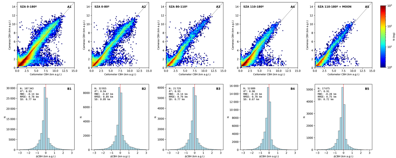
Figure 12. First row (A) presents the bidimensional frequency histogram of median cloud heights values from the camera network within a 150 m radius of the Valladolid ceilometer location, against ceilometer values for cloud base height (CBH). Second row (B) presents the frequency histogram of the differences ( \Delta CBH) between both instruments. Filtering criteria have been applied to discard heights provided by two or fewer cameras, with fewer than 20 height values and a standard deviation higher than 1 km. Rows represent different lighting conditions: SZA 0–180° (all conditions), SZA 0–80° (daylight), SZA 80–110° (twilight), SZA 110–180° (night), and SZA 110–180° (night with moon presence). Results include total number of cases ( N ), coefficient of determination ( R^2 ), mean bias error (MBE), root mean square error (RMSE) and standard deviation (SD).
