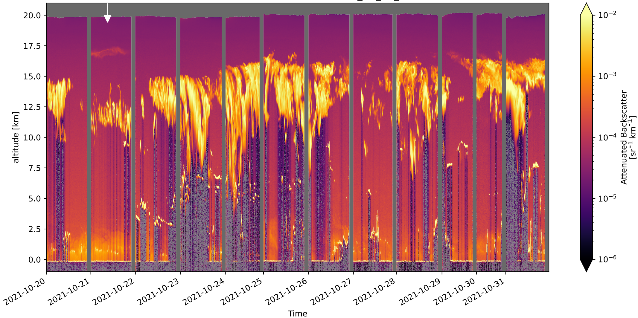
Strateole-2 first BeCOOL flight (ST2_C1_02_STR1)
