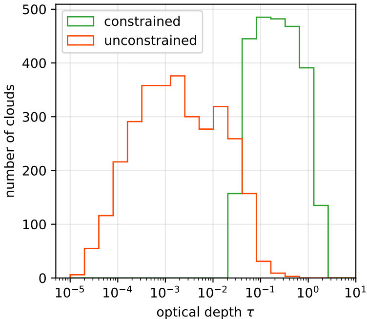
Cloud optical depth distributions
