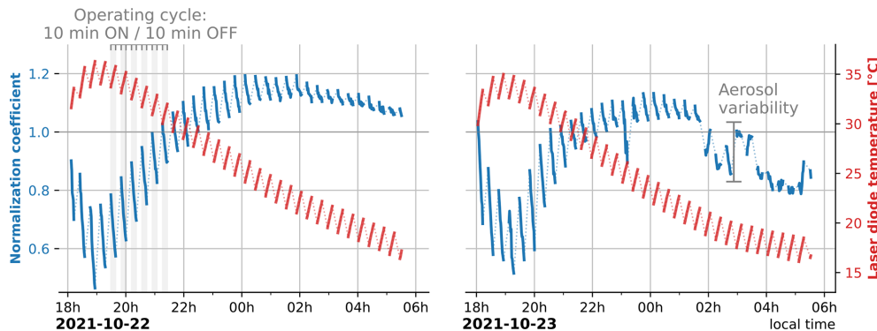
Figure 5. Time series of laser diode temperature (Celsius degrees, red line) and normalization coefficient (arbitrary unit, blue line) for two nights (local time) of flight ST2_C1_02_STR1. The normalization coefficient is the instrumental constant arbitrarily scaled to 1 at a given time. On the left panel (22 October 2021) the operating cycle (10 min ON/10 min OFF) is highlighted in grey.
