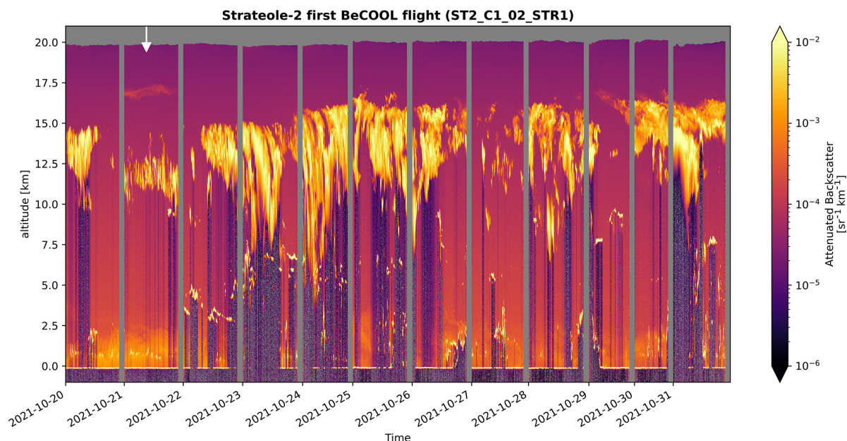
Figure 6. Lidar cross section (time vs. altitude) of the attenuated backscatter signal for the first BeCOOL flight of Stratéole2 2021–2022 scientific campaign, between 20 and 31 October 2021. Vertical grey lines separate two consecutive nights (BeCOOL is not operated during daytime). The upper horizontal grey-shaded area stands for no data. The upper white arrow is pointing the time corresponding to the profile retrieved in Sect. 4.
