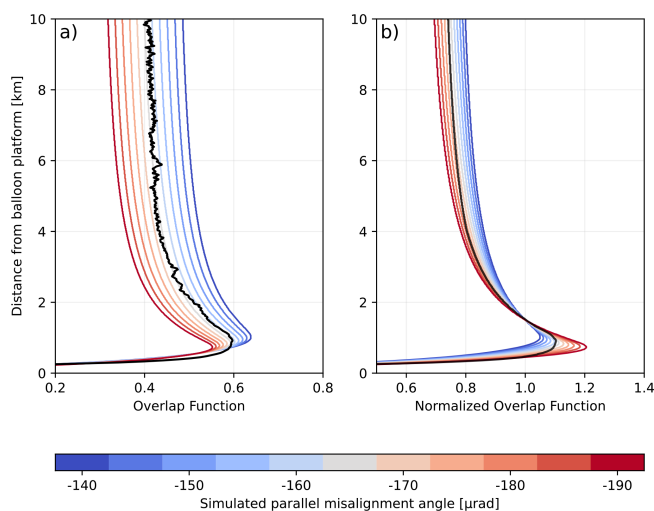
Figure 3. (a) Simulated overlap functions for different parallel misalignment angles between the emission and the reception optical channels. The parallel misalignment angle varies from -140 (blue line) to -190 \mu\text{rad} (red line). Negative values correspond to slightly converging optical axes. The solid black line is a reference clear sky profile used to derive the empirical overlap correction for a given instrument: it is the ratio of the mean lidar profile over a 3 h cloud-free window to a synthetic Rayleigh lidar profile. (b) Same overlap functions (blue to red lines) normalized at a distance of 1.5 km from the platform, along with the empirical overlap correction (smooth solid black line) derived from the reference clear-sky profile, normalized at the same distance.
