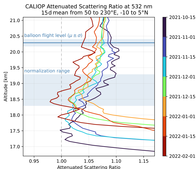
Figure 4. Mean CALIOP attenuated scattering ratio profiles averaged (50 to 230° E, -10 to 5° N) between October 2021 and January 2022. Each color line correspond to a mean over 15 d (red-blue color bar). The mean flight level of the balloon, and its variability is shown (horizontal blue line and upper blue-shaded area). The region where the normalization coefficient is computed (normalization range) is also shown (lower blue-shaded area).
