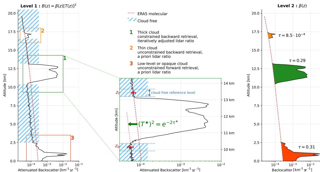
Figure 7. 10-min averaged lidar profile on 21 October 2021 (white arrow on Fig. 6). The attenuated backscatter profile \beta[T(z)]^2 is plotted on the left panel, the backscatter profile \beta(z) on the right panel (the red dashed line is corresponding to \beta_m(z) ). The middle panel is a zoom of the left panel for the cloud in the middle of the profile. The upper and lower red dots correspond respectively to the values of the averaged quantity ( B^r ) at the bottom ( z_b ) and the top ( z_t ) of the cloud. The red brackets show the lower ( B^{r-} ) and upper ( B^{r+} ) values of these reference quantities. The colored areas on the right panel materialize the optical depth for backward constrained retrieval (green), backward unconstrained retrieval (orange) and forward unconstrained retrieval (dark orange).
